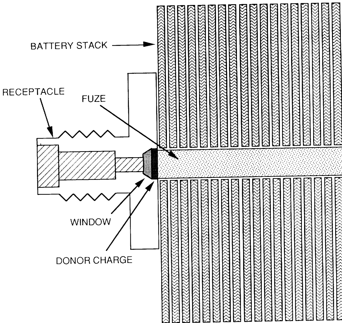
FIGURE 8. Battery Initiator Configuration
