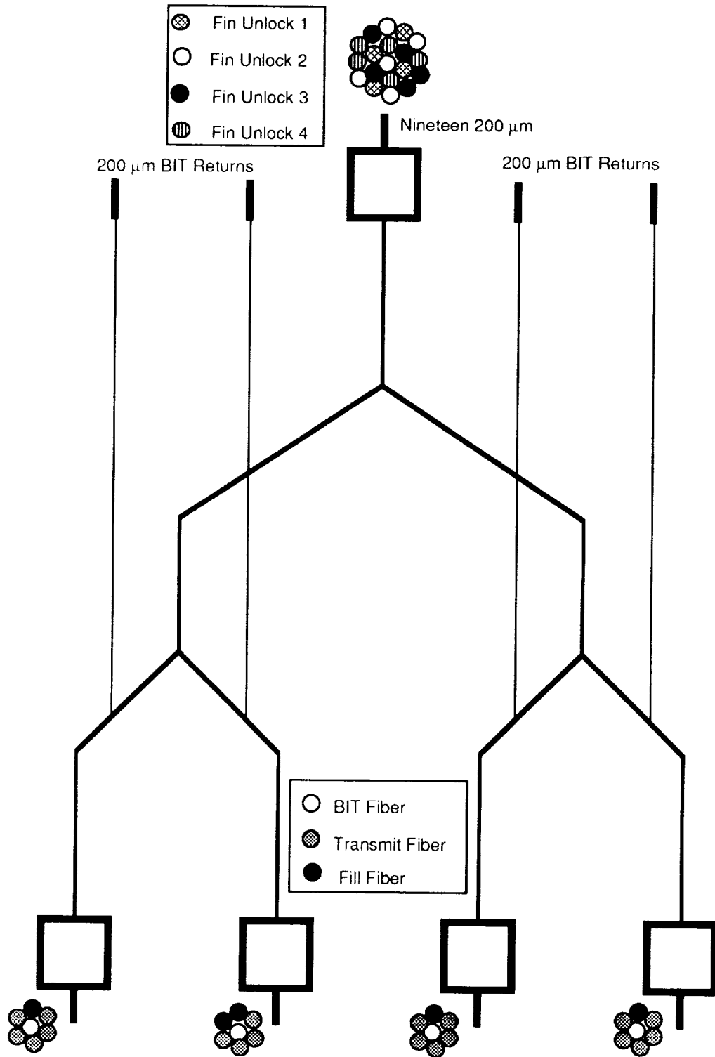
FIGURE 9. Fin Unlock Fiber Optic
