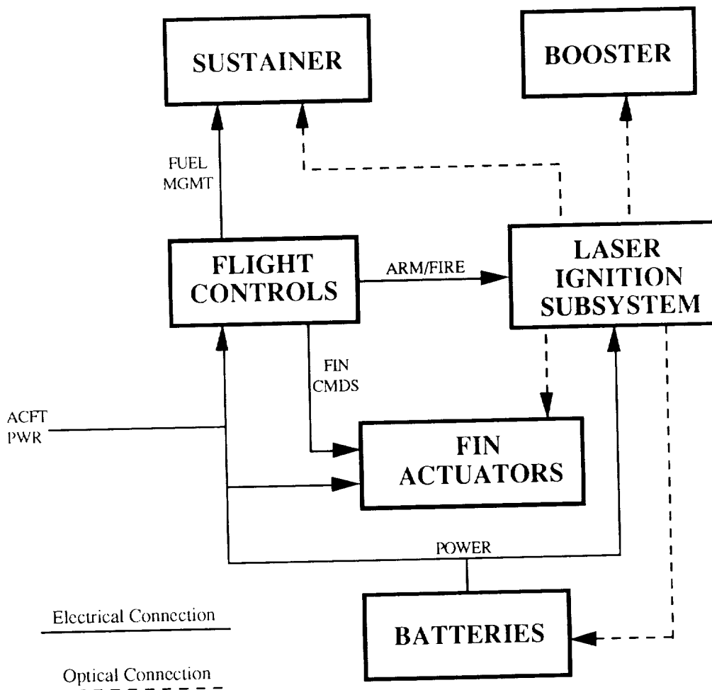
FIGURE 1. Integral Rocket Ramjet System Concept
