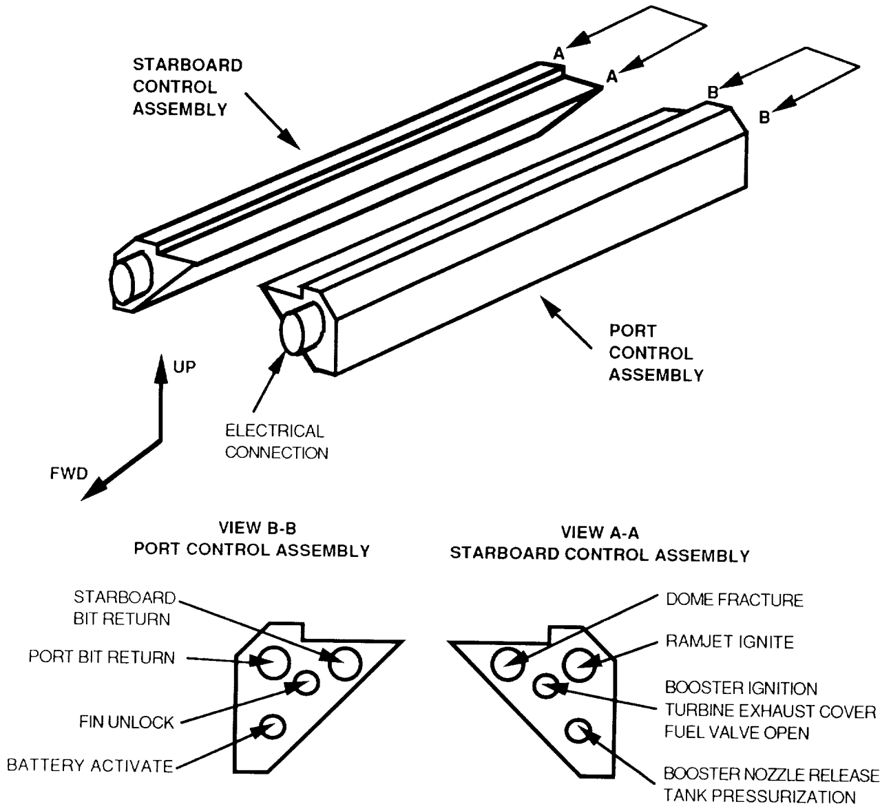
FIGURE 2. Laser Ignition Subsystem (LIS) Control Assemblies
