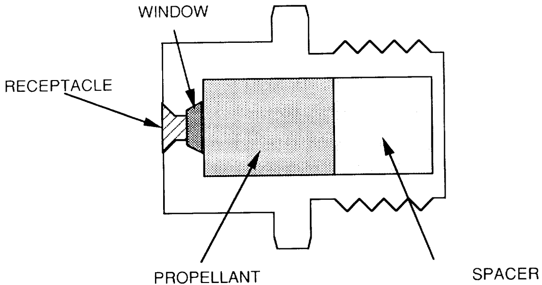
FIGURE 6. Fin Unlock Initiator Configuration
