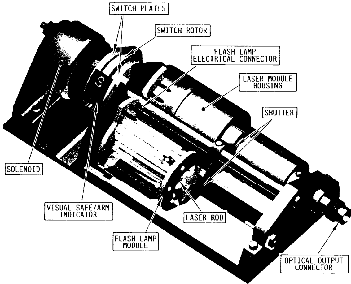
FIGURE 4. A Two-Pulse Laser Assembly
