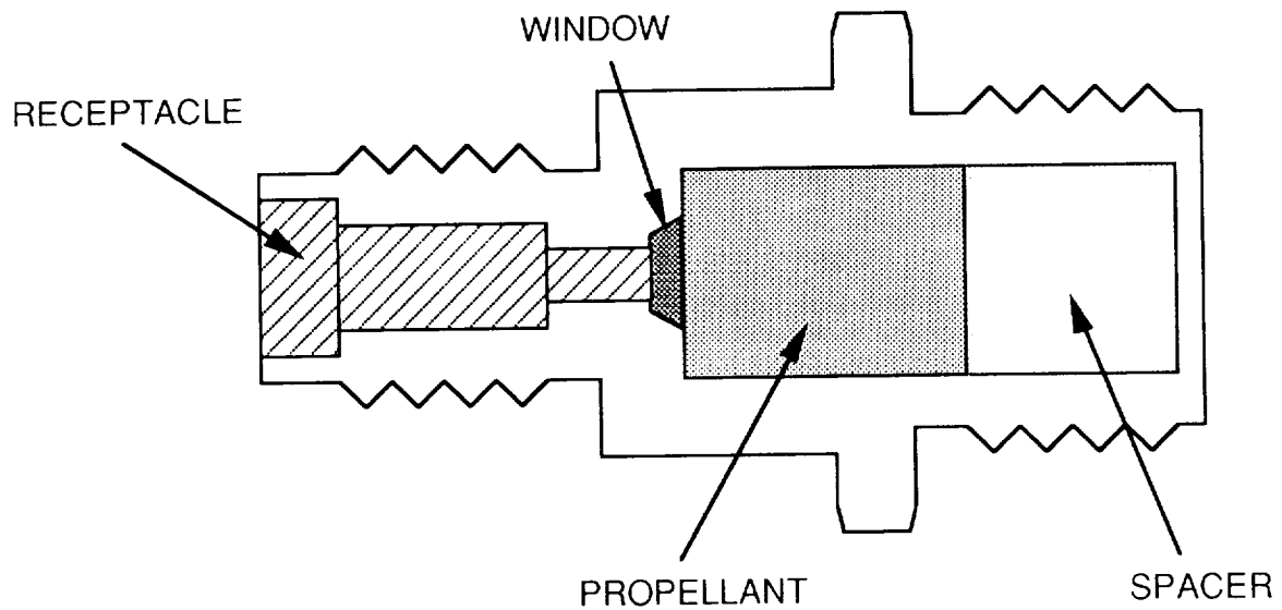
FIGURE 5. Standard Initiator Configuration
