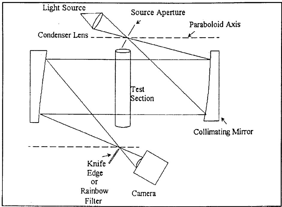
Figure 1 Typical Schlieren Optical System
