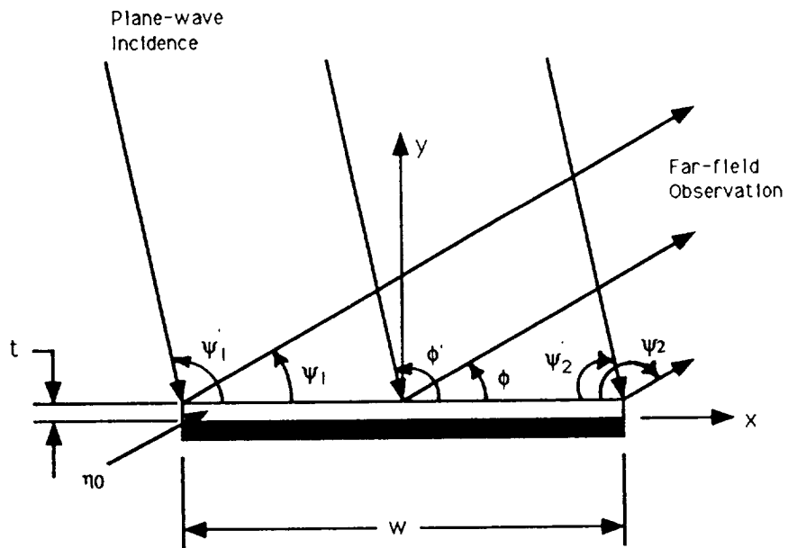
Figure 2: Geometry for principal-plane scattering from a strip/plate with a finite-thickness coating backed by a perfect conductor.
