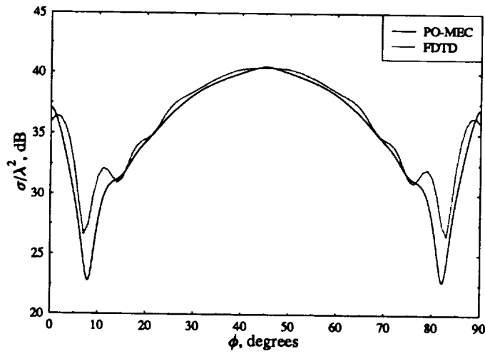
Figure 9: Monostatic RCS of the square trihedral corner reflector with dimensions a = b = c = 5.0\lambda , incident angle \theta = 66^\circ , and polarization of the E-field in the theta direction.
