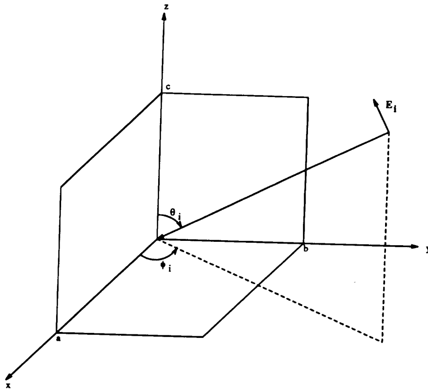
Figure 6: Geometry of the trihedral corner reflector.
