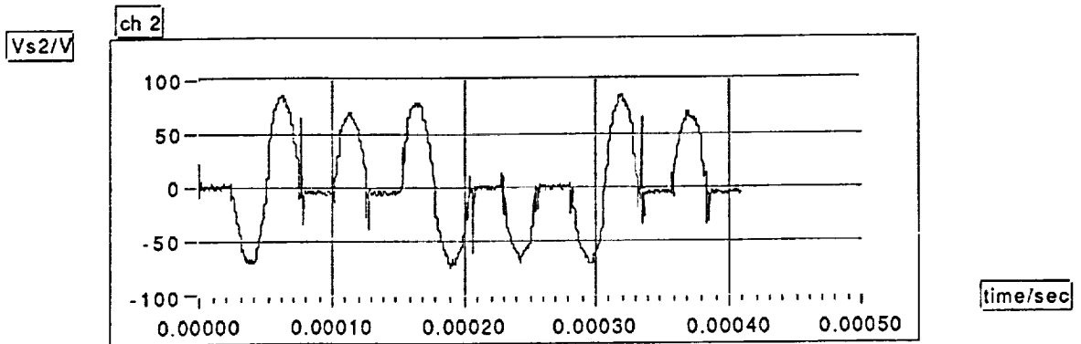
Figure 7 Current shoot-through due to turn-on advance
