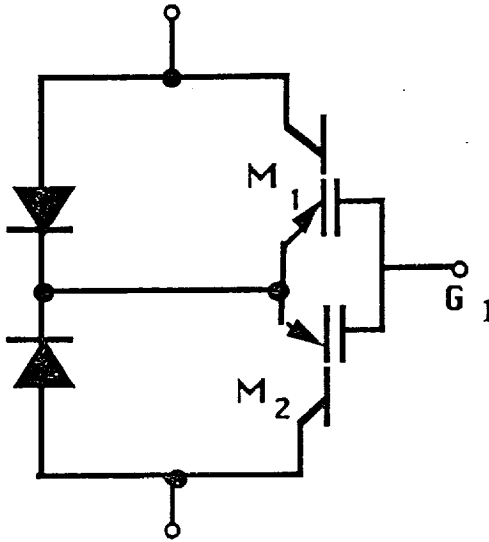
Figure 1 MCT bidirectional Switch
