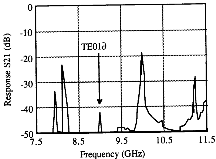
Figure 4. Response of Cavity with DR in Place
