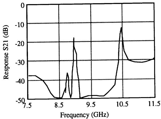
Figure 3. Air Filled Cavity Response
