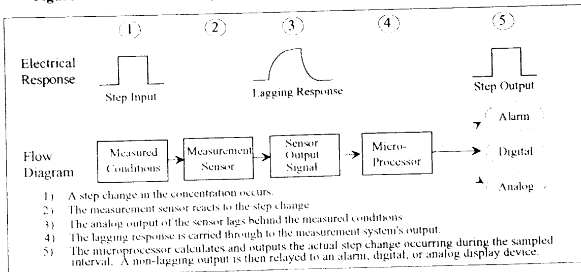
Figure 2. Illustration of Predictive Sensor Method and Apparatus
