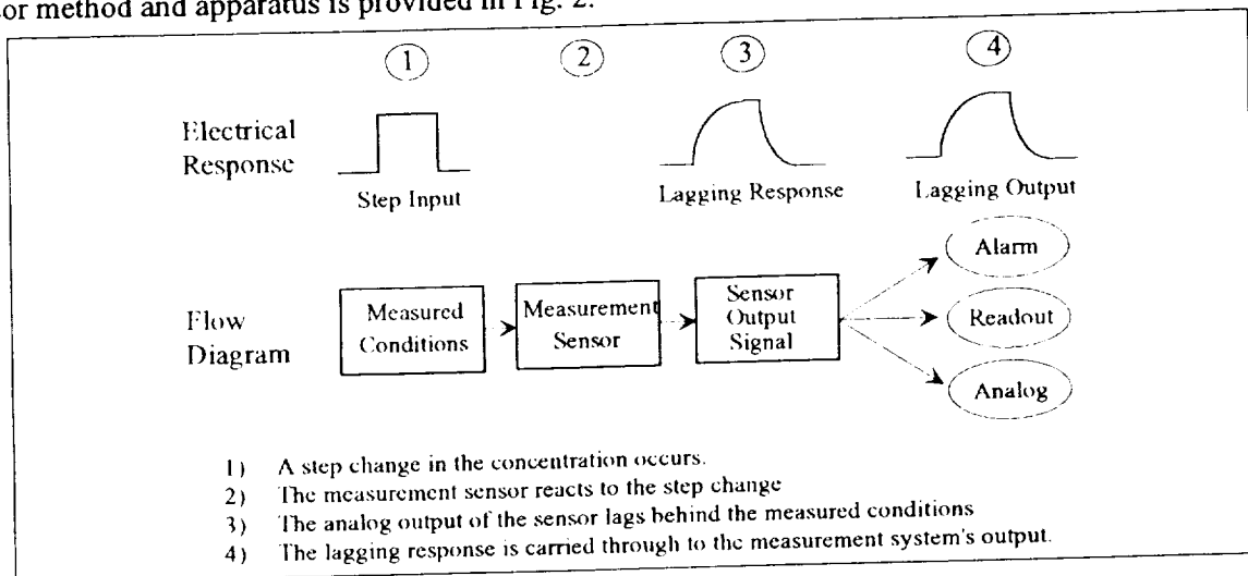
Figure 1. Illustration of Lagging Response in Conventional Measurement Systems
