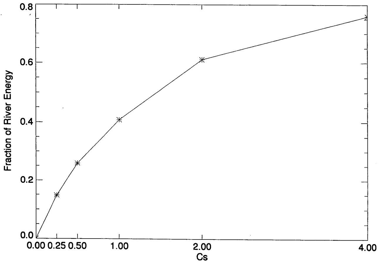
Figure 14. The river fraction of total energy used to melt the ice cover as a function of the heat transfer coefficient, C_s . The effect on the energy partition is non-linear and, since the river parameterization in the model responds proportionally to all of the constant terms ( u , f_{int} , \Delta T ), a similar change to any single parameter will have the same effect on the energy partition.
