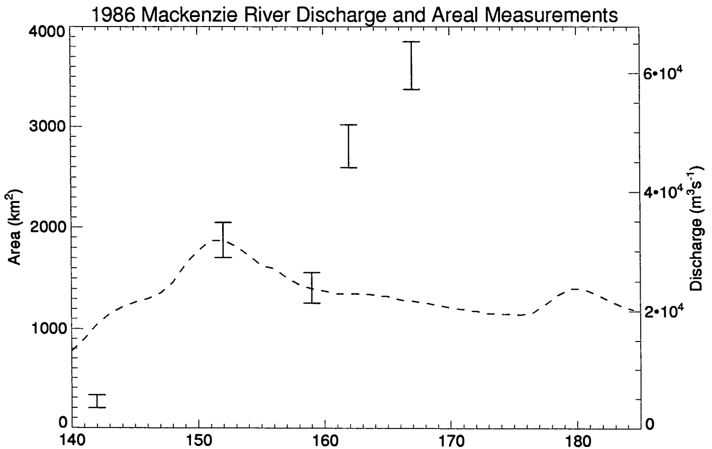
Figure 9. Comparison of 1986 Mackenzie River discharge to areal measurements of river-induced open water. The dashed line is the discharge curve ( m^3s^{-1} ) while the data points are a calculation of the overflow or open water areas ( km^2 ) immediately adjacent to the coast. The area of open water is derived from digitally processed AVHRR satellite images. The first three data points follow the discharge and for the most part represent overflows on top of the ice while the later points diverge as the area of open water enlarges as the ice cover recedes from the coastline.
