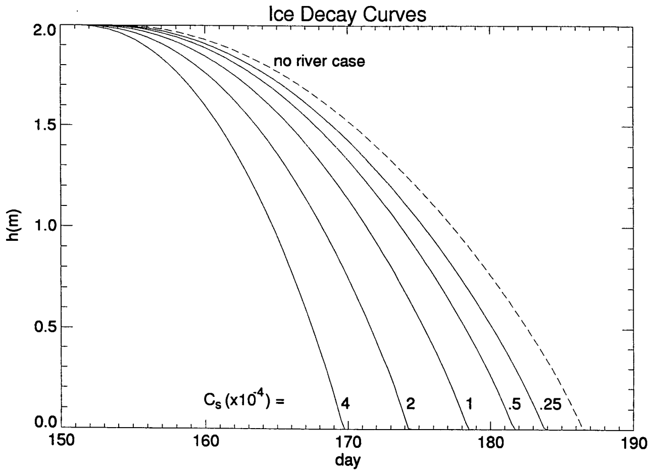
Figure 11. Ice decay curves depict the simulated results of melting due to atmospheric forcing and river heat. The dashed line is the limiting case of no basal heat flux (i.e. no river term) while the solid curves result from varying the river's heat transfer coefficient, C_s , from 0.25 \times 10^{-4} to 4 \times 10^{-4} .
