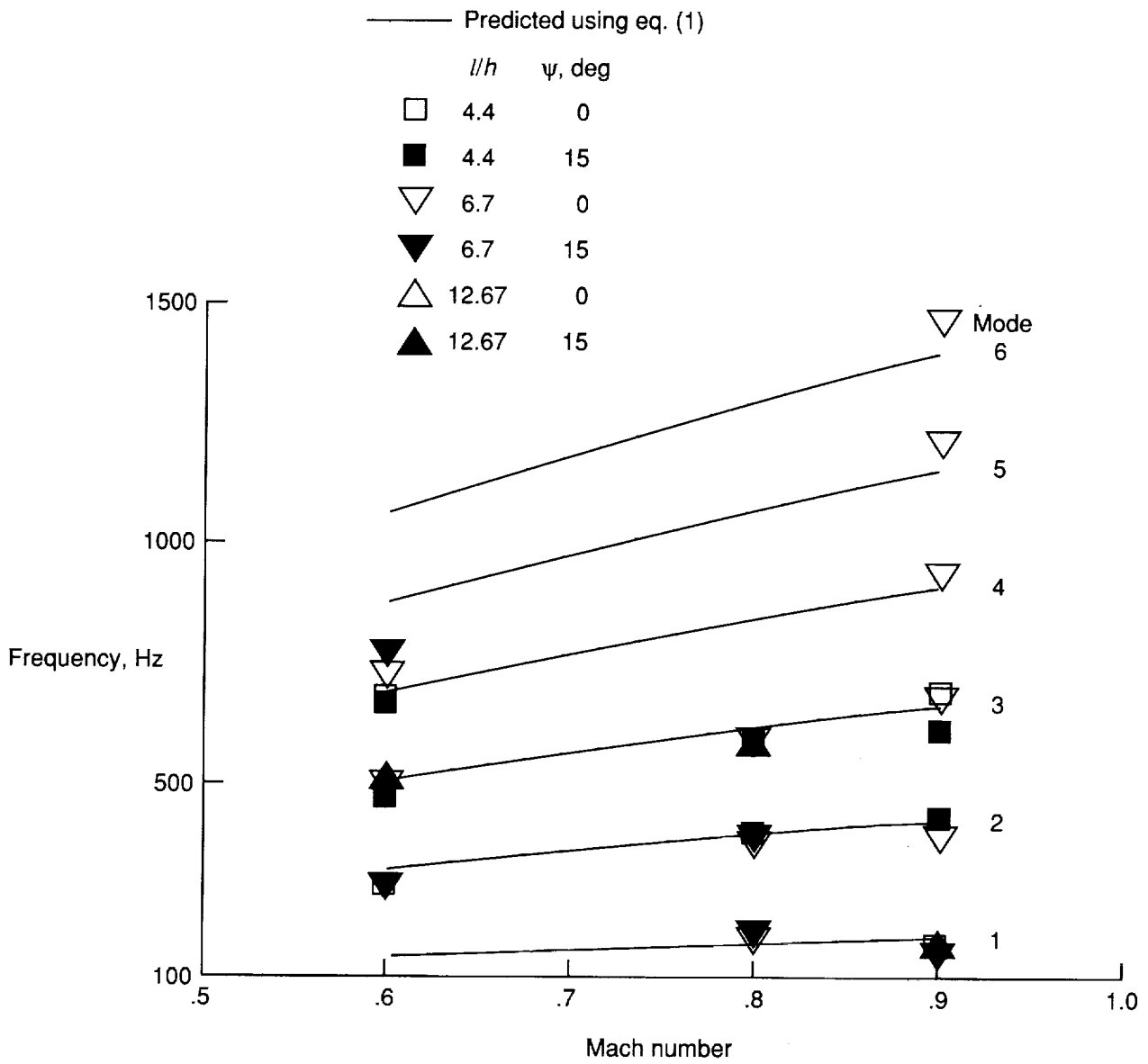
Figure 15. Predicted and observed modal frequencies from tables V and VI, respectively.
