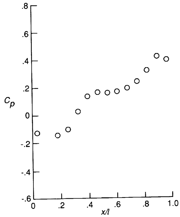
(c) Static pressure distribution for l/h = 12.67 .
