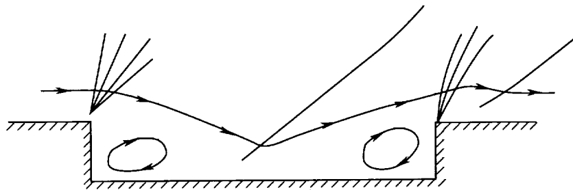
(a) Transitional-closed flow field model.
