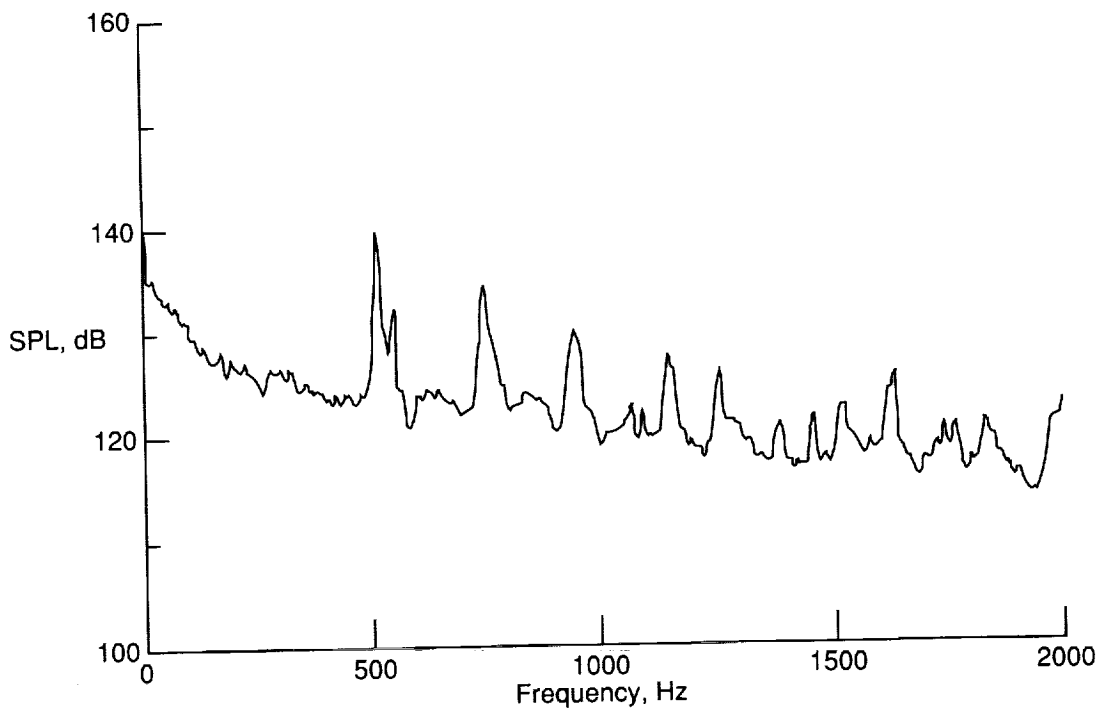
(d) Acoustic spectra measured on forward floor for l/h = 12.67 .
