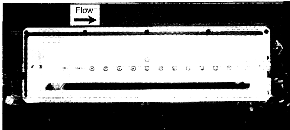
Figure 7. Rectangular cavity model prior to installation in sidewall of Langley 0.3-m TCT. Dynamic pressure transducers are shown.
