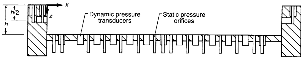
(b) Section side view.
