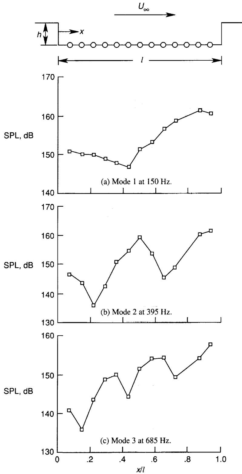
Figure 13. Six mode shapes of a cavity for l/h = 6.7 at M_\infty = 0.9 and \psi = 0^\circ .
