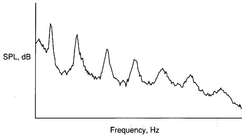
(c) Typical fluctuating pressure spectra.
