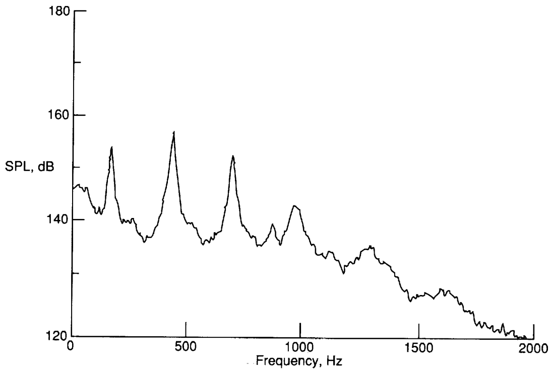
(b) Acoustic spectra measured on forward floor.
