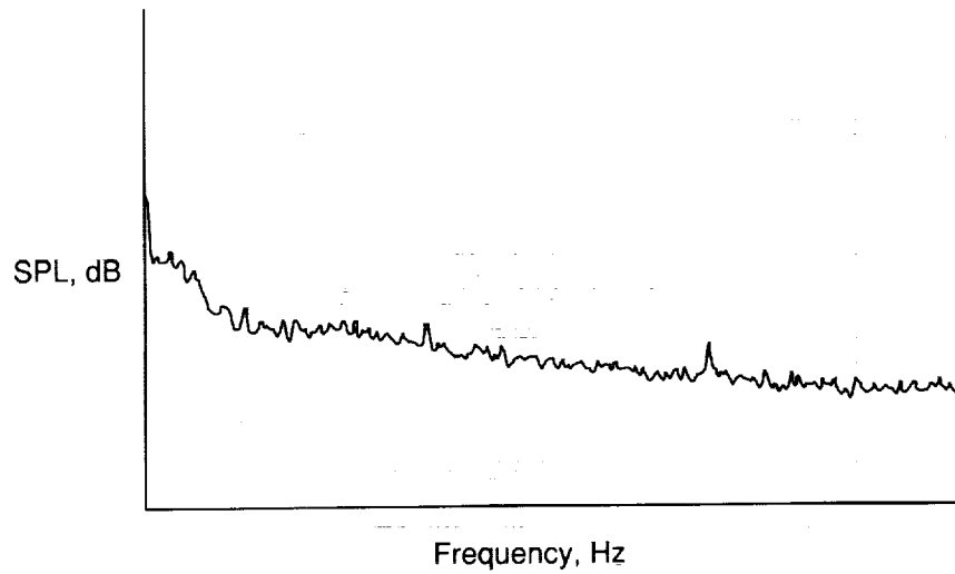
(c) Typical fluctuating pressure spectra.
