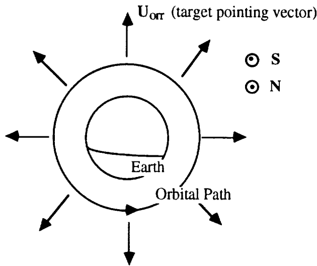
Fig. 3b ORR Mode Target Pointing Vector Along The Orbital Path With Sun Perpendicular To Orbit Plane
