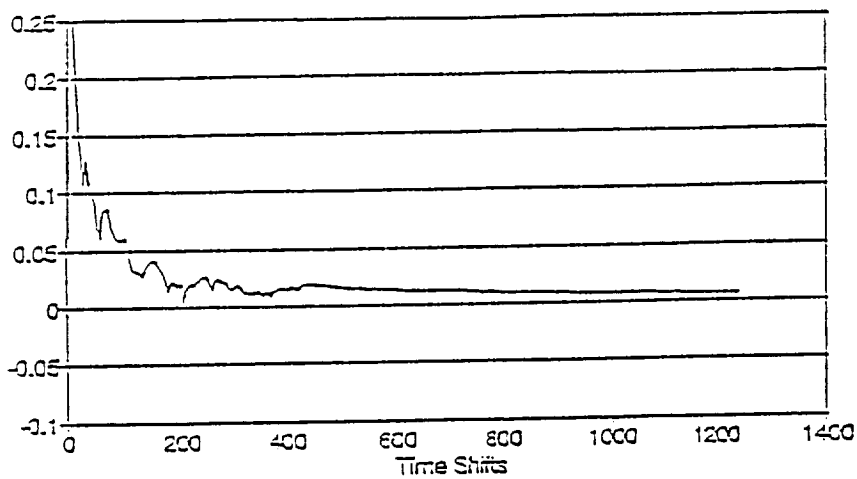
Figure 4. Actual Solar Flux Time Series
