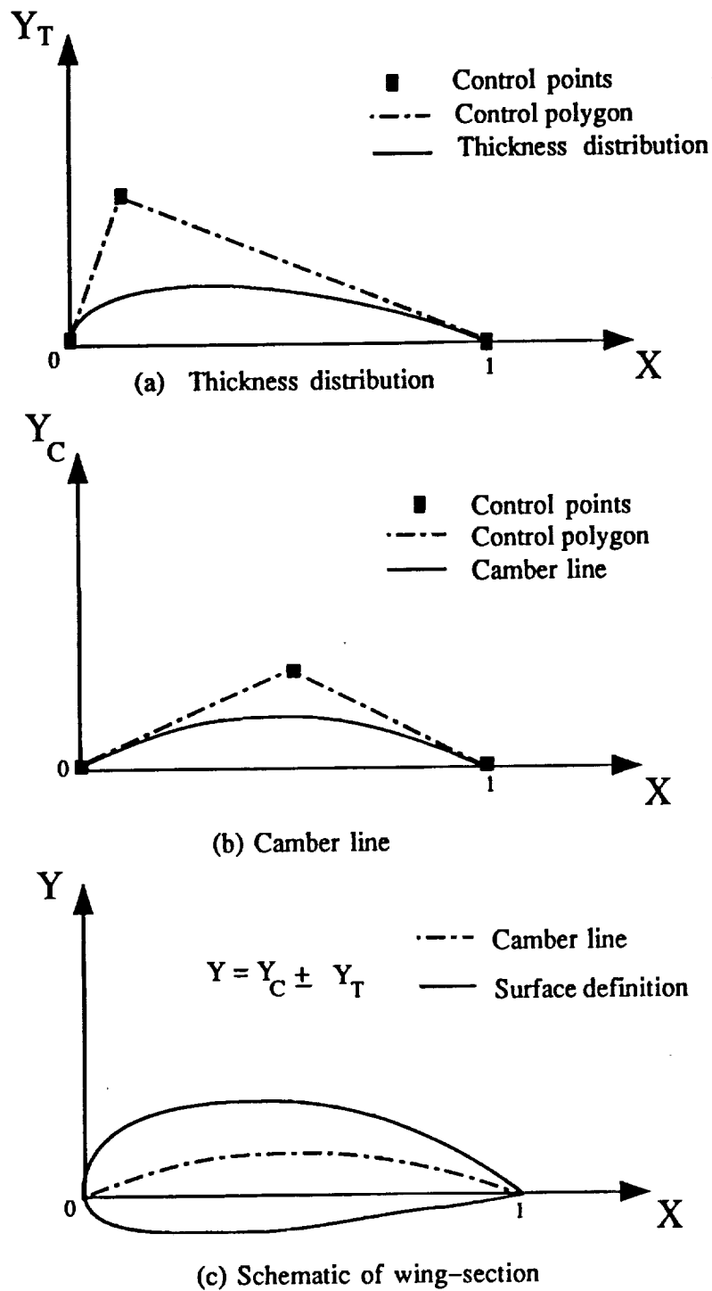
Fig. 2.6 Wing-section specification using NURBS (option 2).
