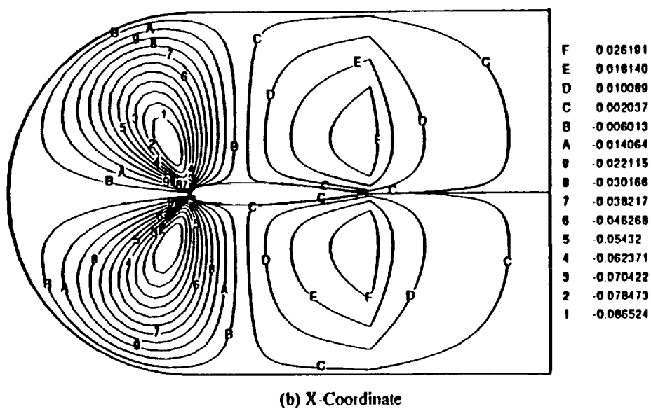
Fig. 6.1 Coordinate sensitivity with respect to maximum thickness T (DD).
