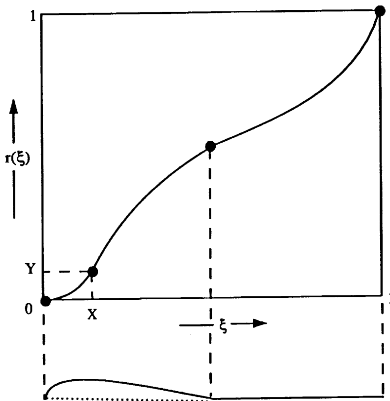
Fig. 3.8 Control domain for lower boundary discretization.
