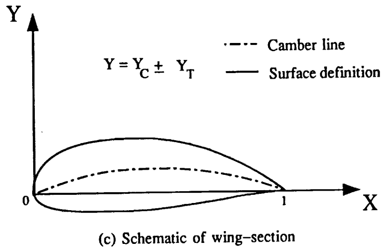
Fig. 2.2 Wing-section specification using NURBS (option 1).
