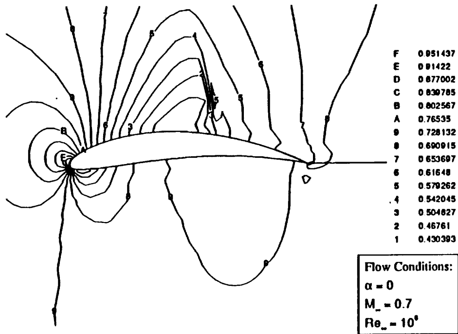
Fig. 6.14 Pressure contours for NACA 8512 wing-section.
