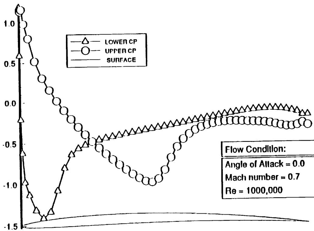
Fig. 6.16 Surface pressure coefficient for NACA 8512 wing-section.
