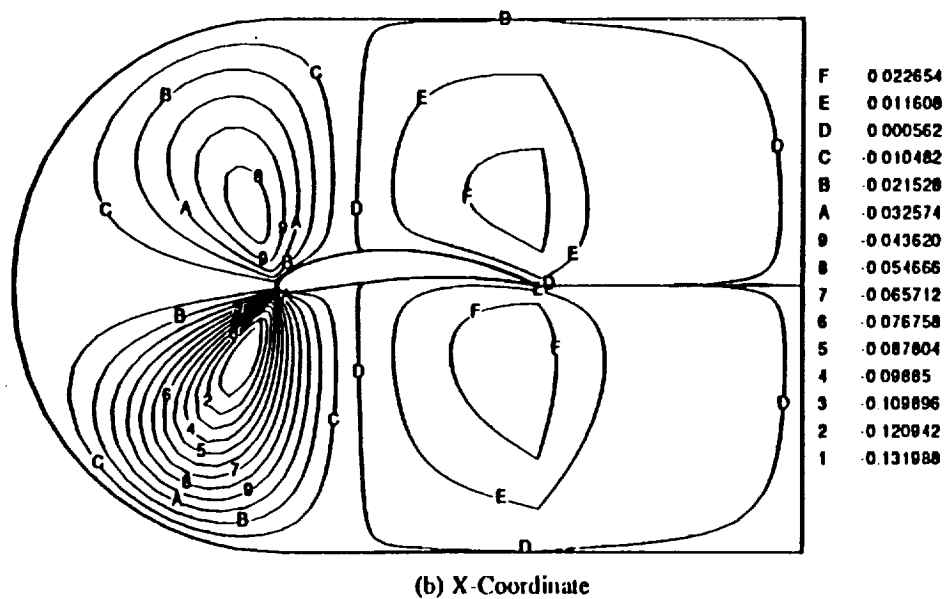
Fig. 6.7 Coordinate sensitivity with respect to maximum thickness T .
