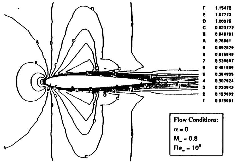
Fig. 6.5 Mach number contours for NACA 0012 wing-section.
