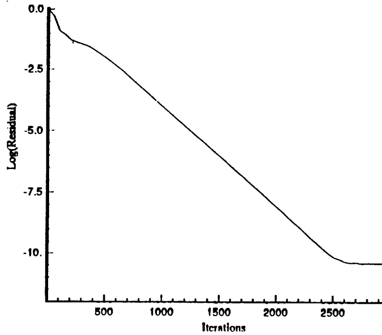
Fig. 6.3 Residual convergence history.
