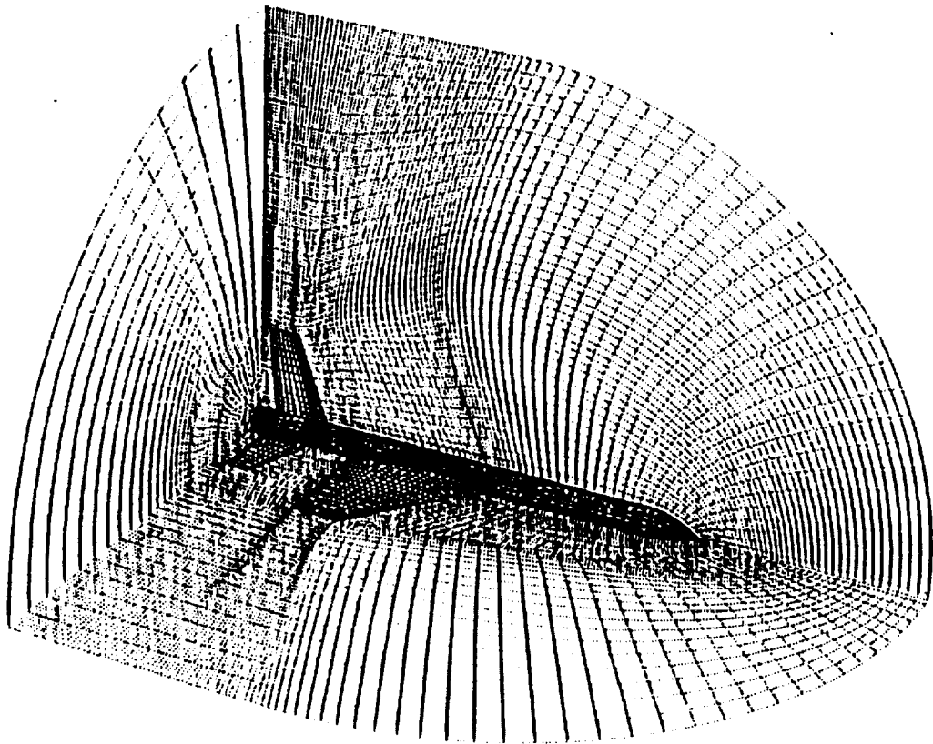
Fig. A.3 Grid on the physical and non-physical surfaces.
