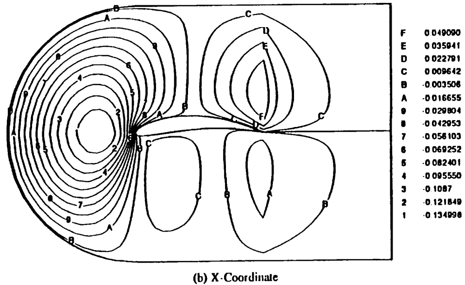
Fig. 6.12 Coordinate sensitivity with respect to grid orthogonality. parameter K_1 .
