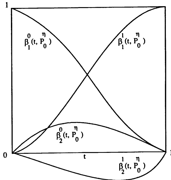
Fig. 3.6 Hermite cubic blending functions.
