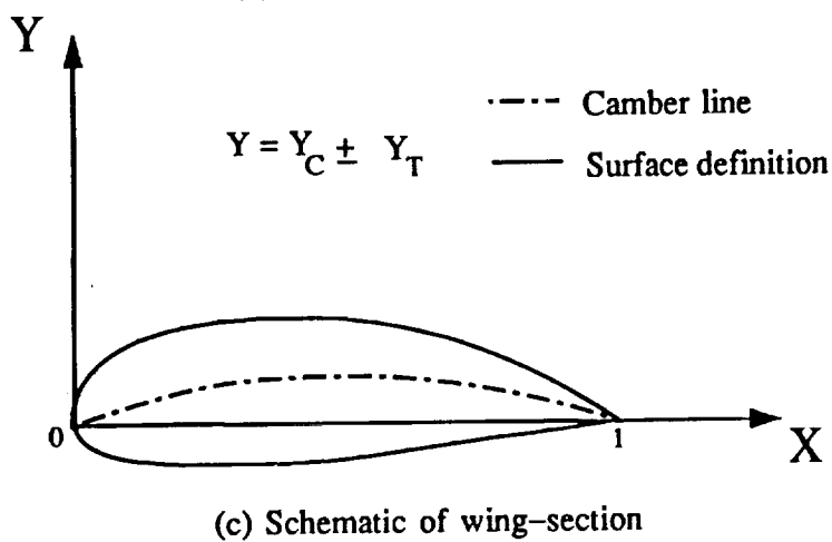
Fig. 2.1 Wing-section specification for NACA four-digit series.
