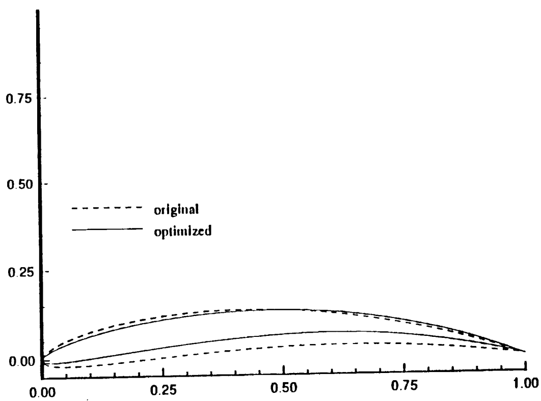
Fig. 6.18 Original and optimized wing-section.
