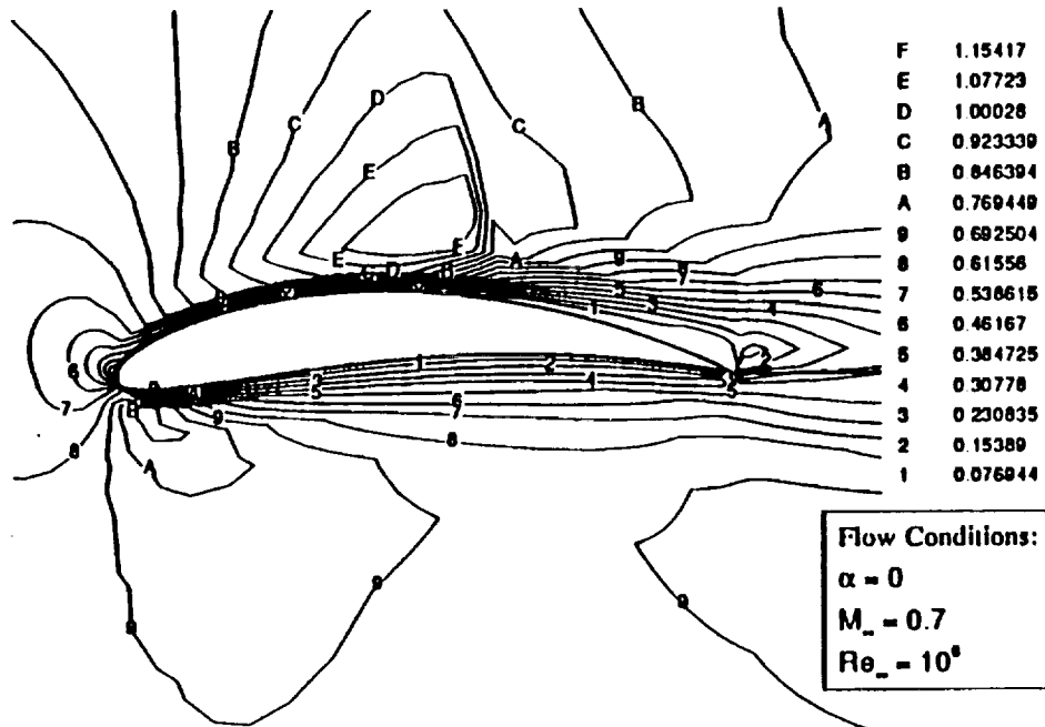
Fig. 6.15 Mach number contours for NACA 8512 wing-section.
