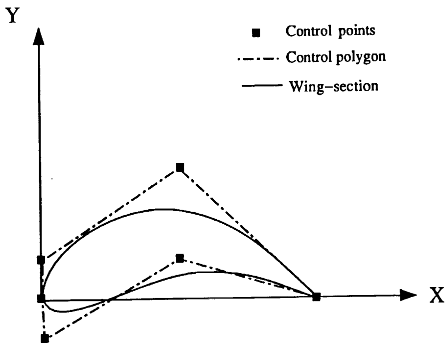
Fig. 2.8 Effect of control point movement.
