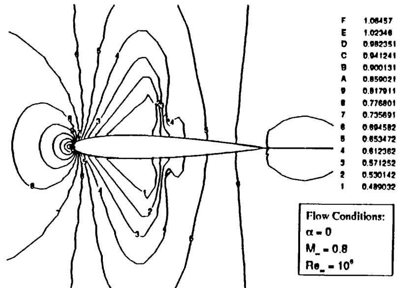
Fig. 6.4 Pressure contours for NACA 0012 wing-section.
