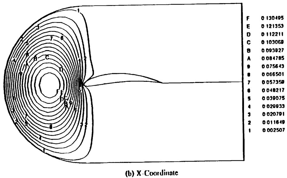
Fig. 6.10 Coordinate sensitivity with respect to grid stretching parameter B_3 .
