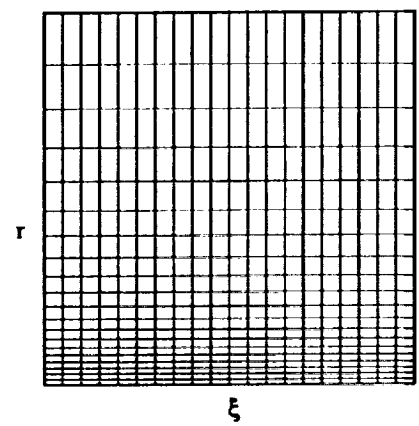
Fig. 3.4 Grid resulting from typical distribution functions.
