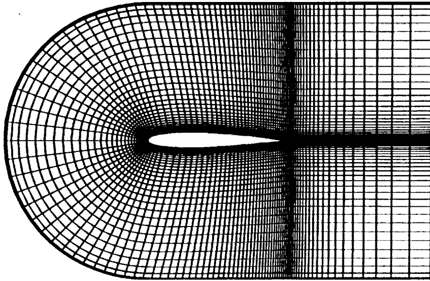
Fig. 3.9 Example grid for NACA 0012 wing-section
