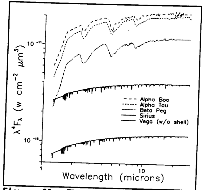
Figure 29. The Atlas of calibrated stellar spectra.
