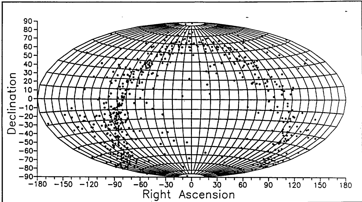
Figure 3. Stars with potential flux contamination from nearby neighbors.
