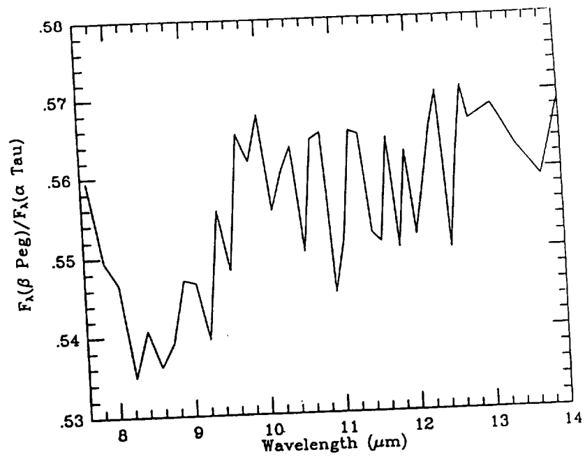
Figures 14b and 14c: Differential effects in the LRS database.
