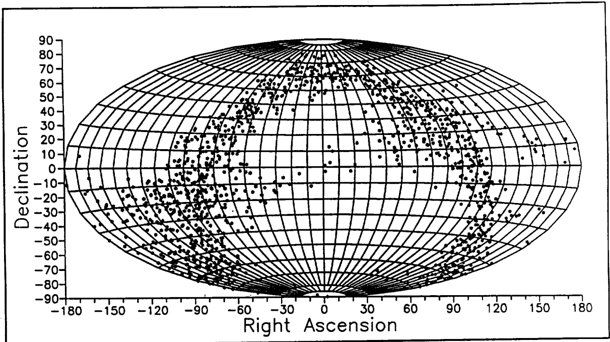
Figure 5. Stars with potential flux contamination by infrared cirrus.
