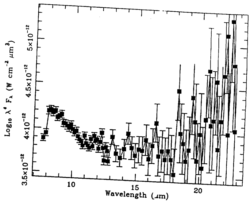
Fig. 15: LRS spectrum of \alpha CMA \lambda^4 F_\lambda space. Note the "emission" feature from 8-10 \mu\text{m} .
