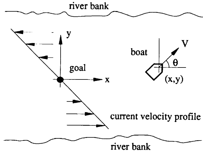
Figure 3: Control of a boat navigating through a river with linear current profile.
