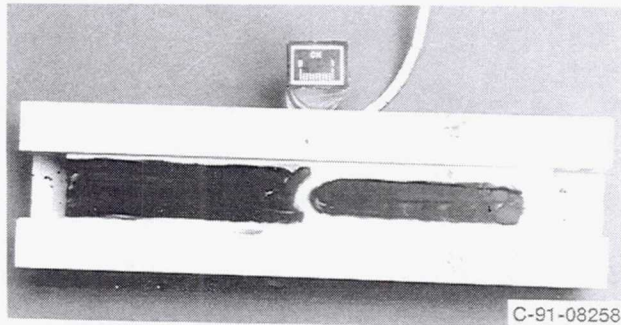
Figure 10.—Pt13Rh/Pt thin film thermocouple on silicon nitride substrate for arc lamp heat-flux-calibrator test.
