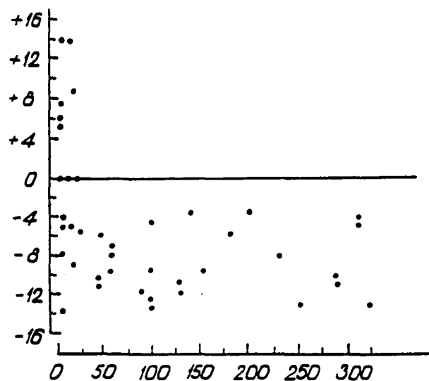
Figure: Dynamics of hematocrit value (in %) in cosmonauts during flights varying in duration Abscissa - days of flight; ordinate - percent change of hematocrit compared to preflight
