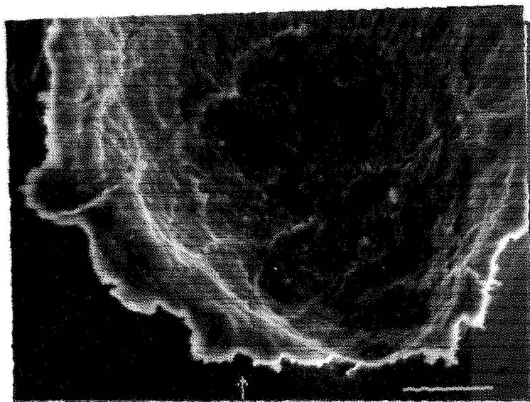
Micrograph 5: View of micrograph 4 at the leading edge. Note the lack of any crater lip (near the scale bar). [ X1700, 10 \mu\text{m} bar, Vel. = 5.6 \text{km.s}^{-1} ]
