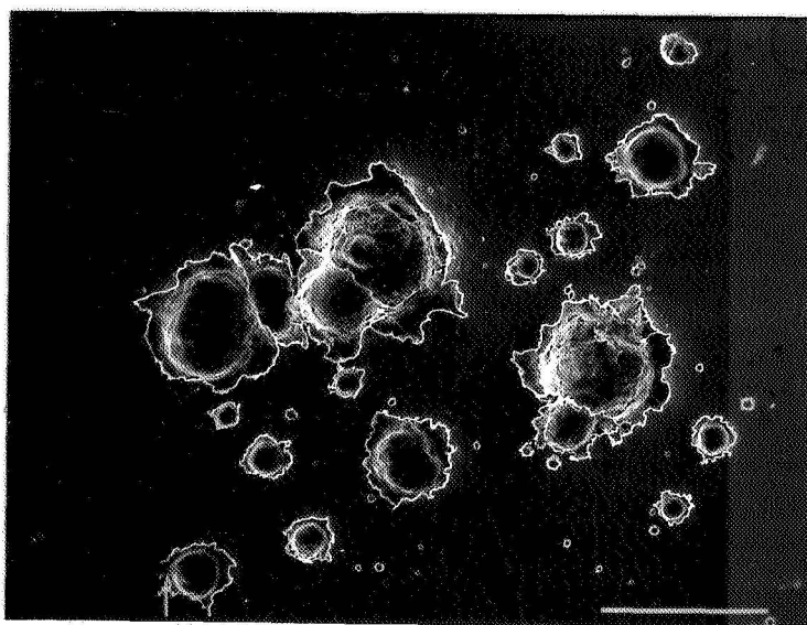
Micrograph 2: 30^\circ impact formed by olivine particle which broke up. Note how the morphology is the same as micrograph 1. [X200, 100\ \mu\text{m} bar, V = 8.3\ \text{km.s}^{-1} ].
