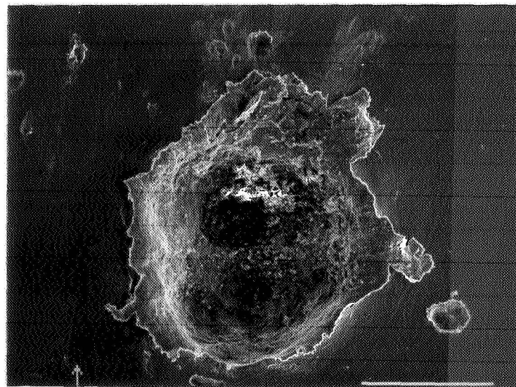
Micrograph 8: 60 ° impact of a partially broken up particle. [X250, 100 \mu\text{m} bar, \text{Vel.} = 4.6 \text{ km.s}^{-1} ]
