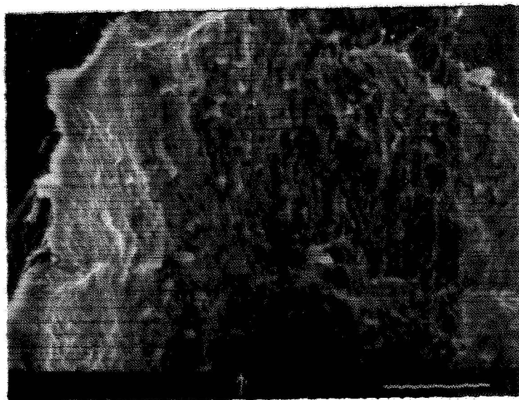
Micrograph 6: Trailing edge of crater in micrograph 4. Closer inspection shows more olivine grains, and X-ray analysis gives more intense peaks in this area. [ X2000, 10 \mu\text{m} bar, V = 5.6 \text{km.s}^{-1} ]
