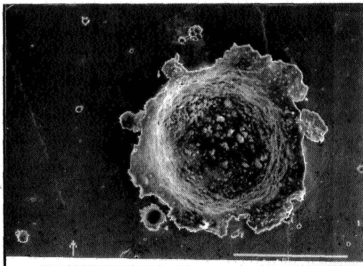
Micrograph 1: 30^\circ impact crater formed by olivine particle. Olivine coating throughout the interior, with visible particle grains. Arrow in lower left-hand corner of all micrographs points toward the crater trailing edge. [X300, 100\ \mu\text{m} bar, V = 7.0\ \text{km.s}^{-1} ]
