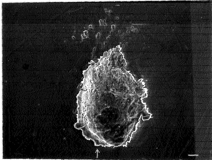
Micrograph 4: 60° impact formed by olivine. Note elliptical shape of crater. [ X500, 10 \mu\text{m} bar, V = 5.6 \text{ km.s}^{-1} ]
