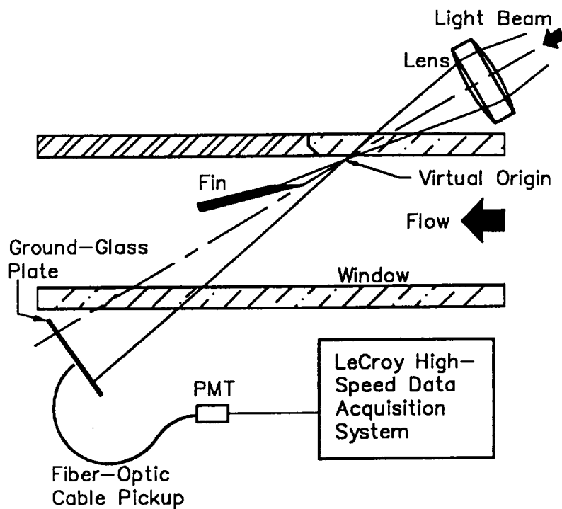
Fig. 5 Conical deflectometry setup
