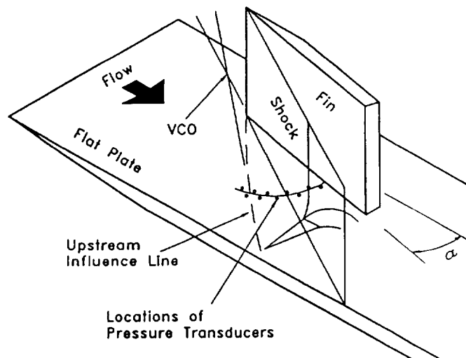
Fig. 4 - Model schematic showing transducer locations
