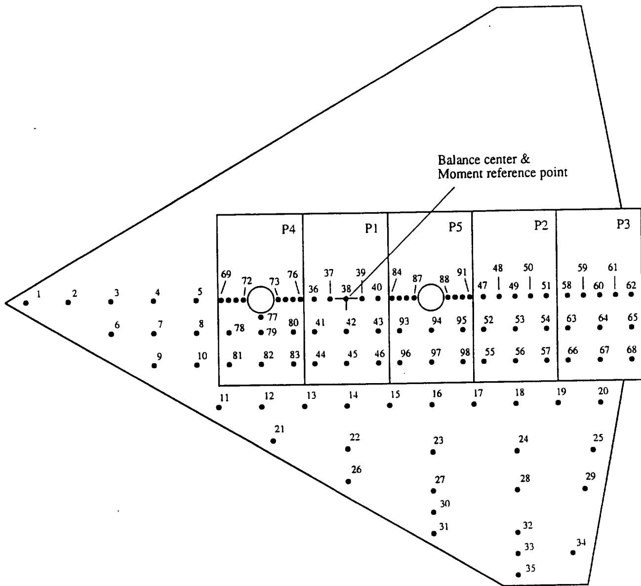
Figure 53. Configuration 2C_8_0_DW; D_e = 1.697 in., A_{jet} = 2.26 in. 2 .
