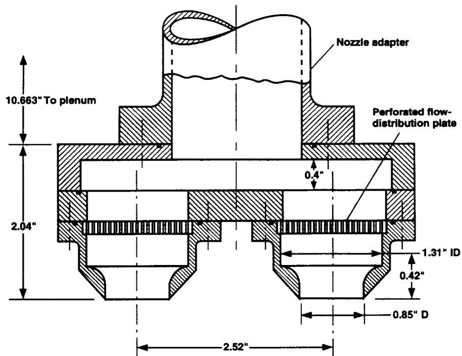
Figure 23. Nozzle-type 4, 0.85-in.-diameter side-by-side nozzles (2.52 in. spacing).
