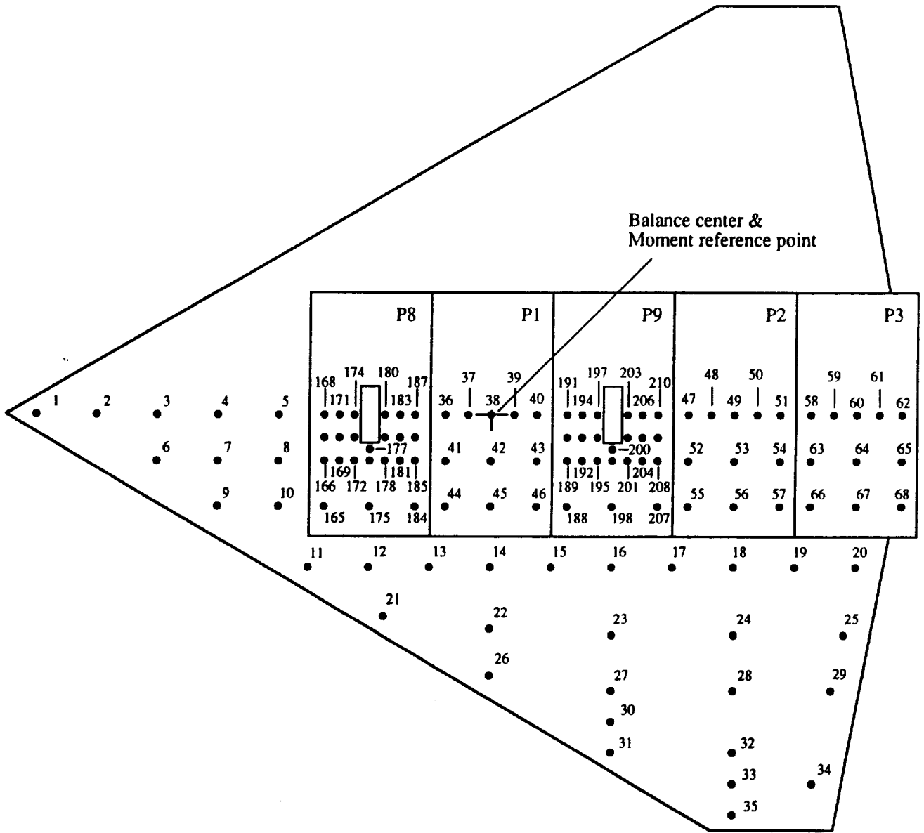
Figure 71. Configuration 2R_8_0_DW; D_e = 1.695 in., A_{jet} = 2.26 in. 2 .
