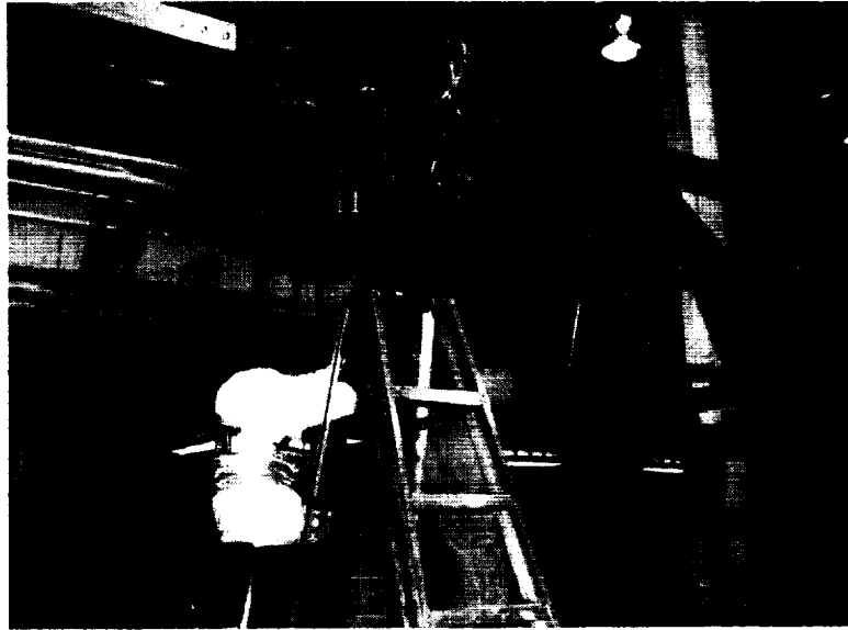
Figure 3. The hover test rig (HTR) support with a delta-wing configuration attached.
