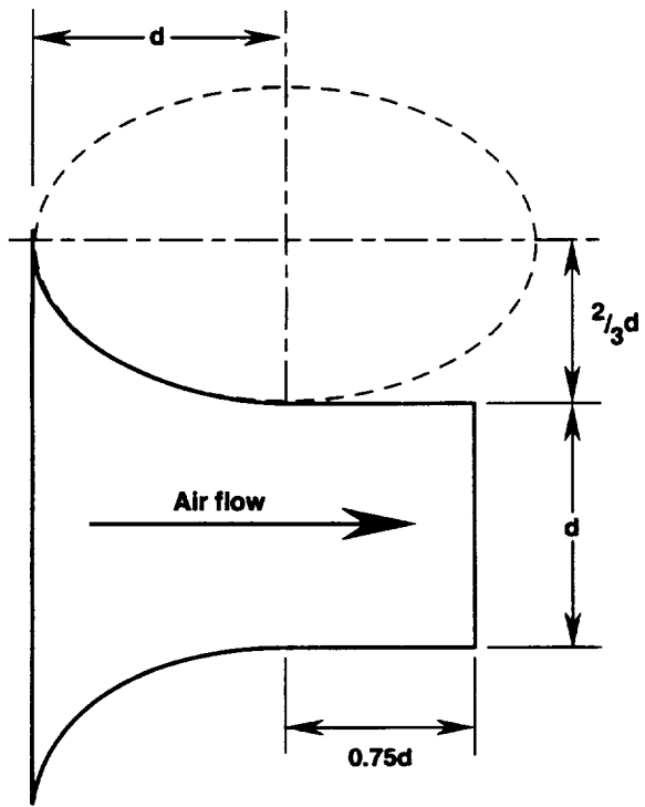
Figure 19. American Society of Mechanical Engineers (ASME) long-radius nozzle definition.
