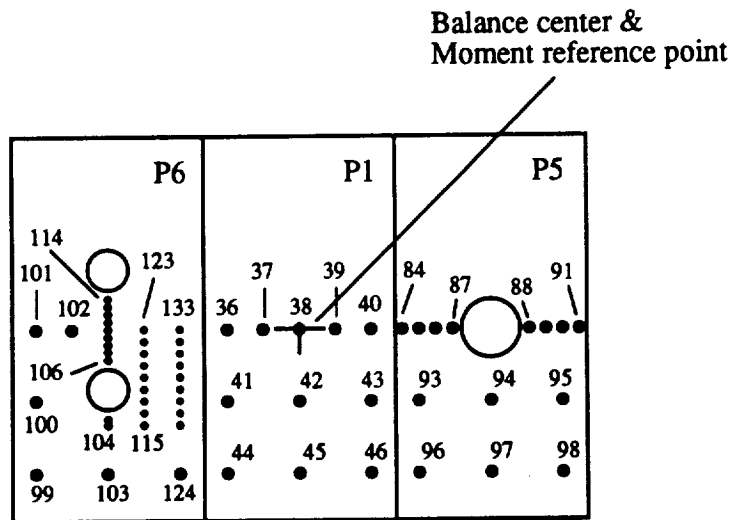
Figure 74. Configuration 3C_8_2.5_12/8; D_e = 1.699 in., A_{jet} = 2.27 in. 2 .
