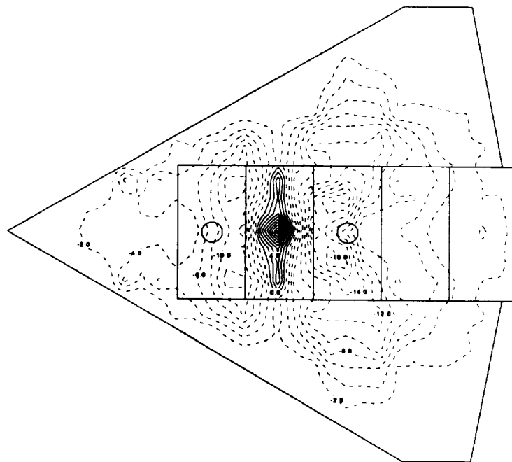
(a) 8-in.-jet spacing (R187P7), c_{pmax} = 0.0188 , c_{pmin} = -0.0260 .
