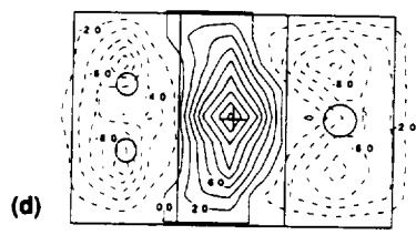
Figure 45. Continued. (c) 3C_8_2.5_DW (R260P7), h/D_e = 3.53 ( h = 6 in.), c_{pmax} = 0.0121 , c_{pmin} = -0.0191 , (d) 3C_8_2.5_12/8 (R268P9), h/D_e = 3.53 ( h = 6 in.), c_{pmax} = 0.0168 , c_{pmin} = -0.0245 .
