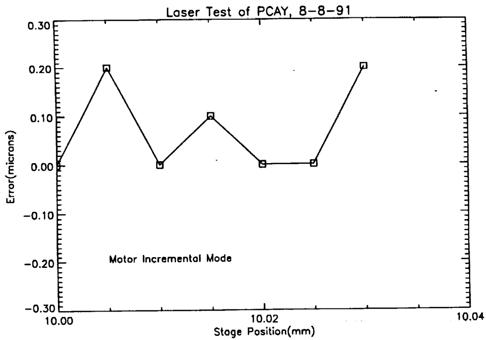
Figure 7. PCAZ Stage Position Errors - Full Travel
