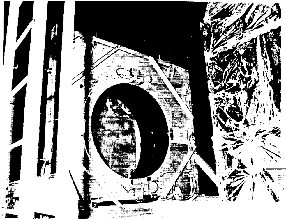
Figure 3. VXDS Beam Normalization Detectors
