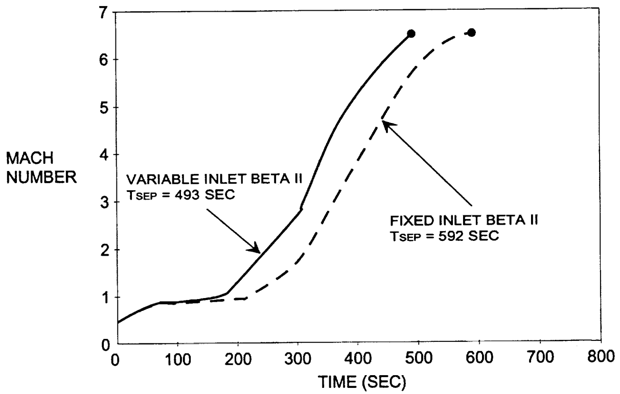
Figure 14. Inlet Study Trajectory
