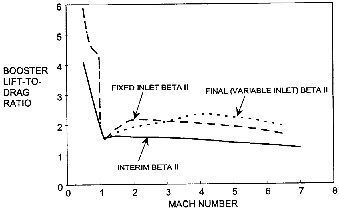
Figure 12. Beta II Lift to Drage Comparison
