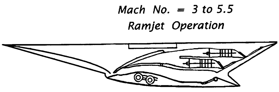
Figure 13. Beta II Nacelle Concept
