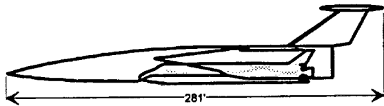
Figure 9. Interim Beta II Booster Concept
