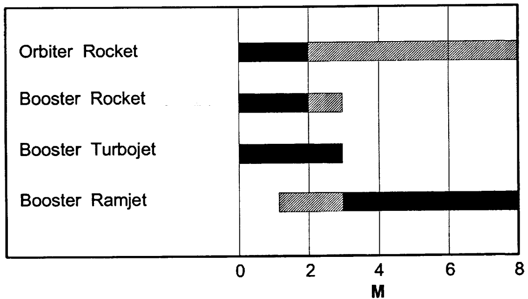
Figure 6. Beta I Engine Operating Schedule
