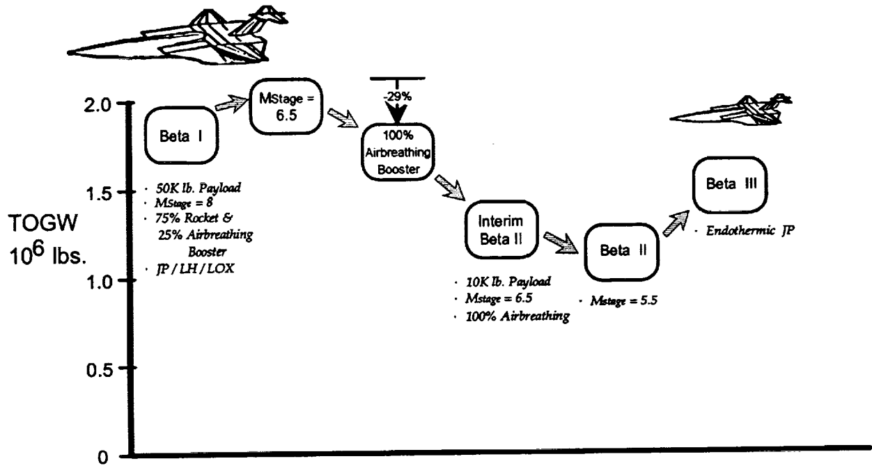
Figure 7. Evolution of Beta Airbreathing Launch Vehicle
