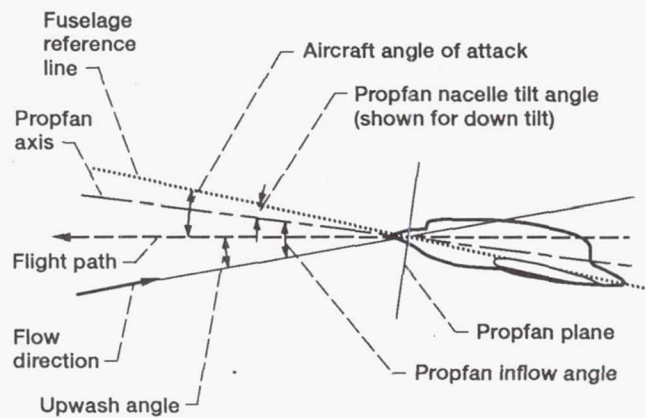
Figure 12.—Propeller installation and flow angles.
