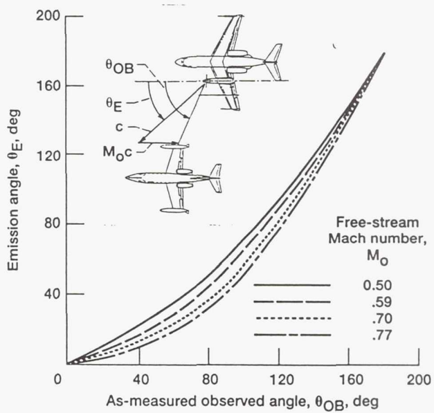
Figure 13.—Relationship between observed and emission angles. \theta_E = \theta_{OB} - \sin^{-1}(M_0 \sin \theta_{OB}) , where c is the local speed of sound.
