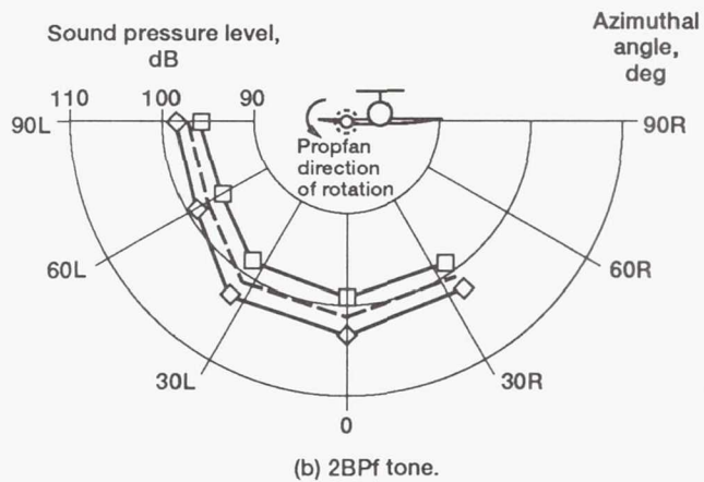
Figure 16.—PTA aircraft azimuthal directivity viewing upstream for case 1 conditions. Mach 0.70; altitude, 10 668 m (35 000 ft); data adjusted to 152-m (500-ft) free field conditions. (Wingtip microphone used at 60° and 90°; cabin roof microphone used at 0° and 30°.)
