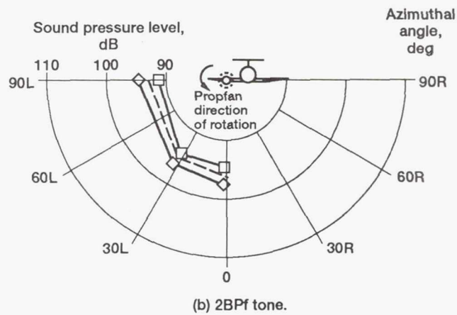
Figure 28.—PTA aircraft azimuthal directivity viewing upstream for case 8 conditions. Mach 0.70; altitude, 10 668 m (35 000 ft); data adjusted to 152-m (500-ft) free field conditions.
