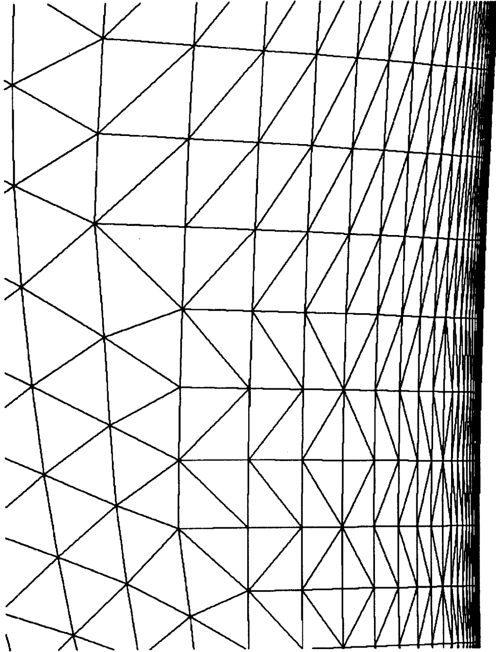
Figure 5- Unstructured viscous grid on the upper surface of a NACA 0012 airfoil showing highly stretched cells.
