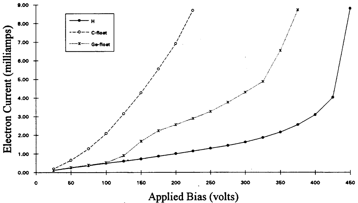
Figure 2 - Electron Current vs Bias
