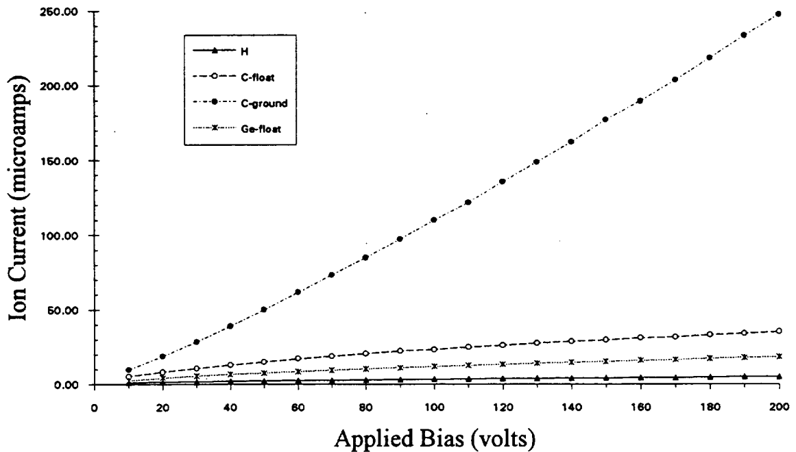
Figure 1 - Ion Current vs Bias
