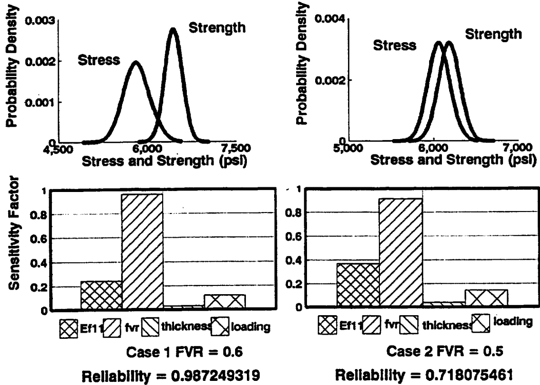
Figure 3.—Reliability analysis of the node at the crown for ply configuration (90/45/-45/0/90) s and sensitivity of random variables to the reliability.
