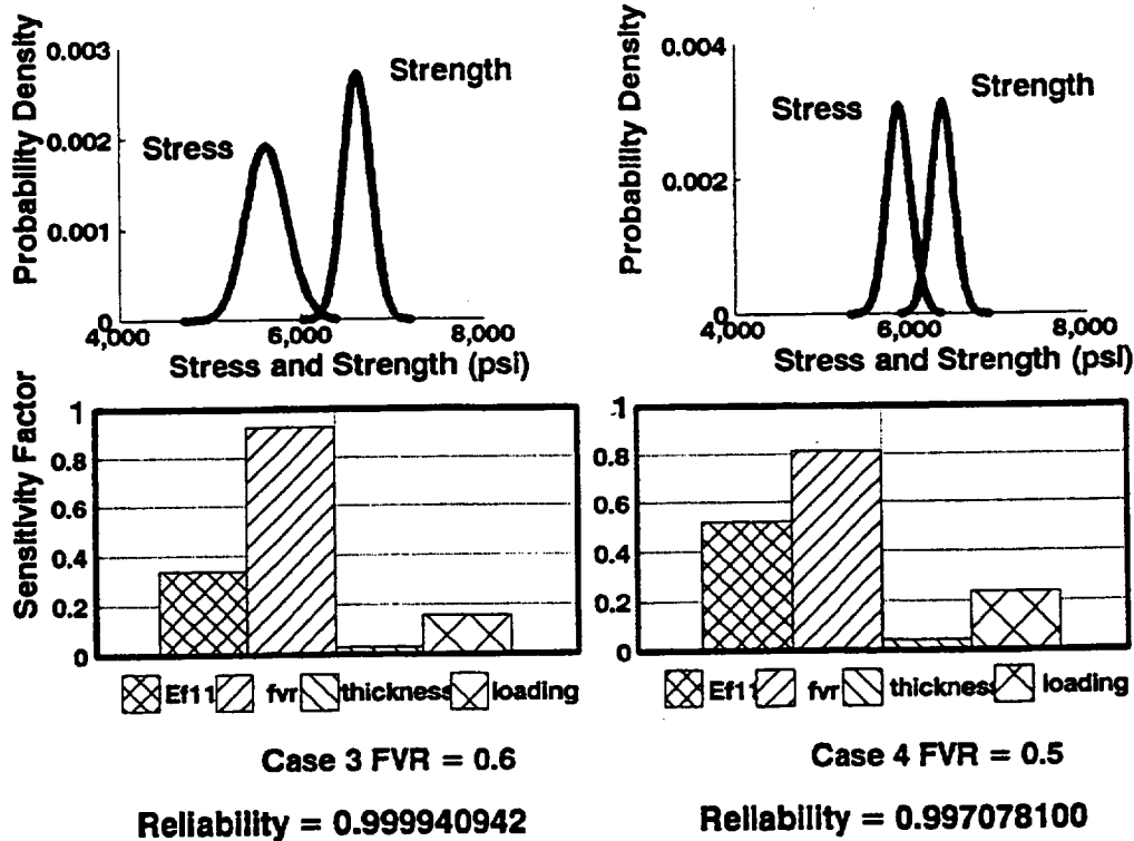
Figure 4.—Reliability analysis of the node at the crown for ply configuration (0/0/90/90)_3 and sensitivity of random variables to the reliability.
