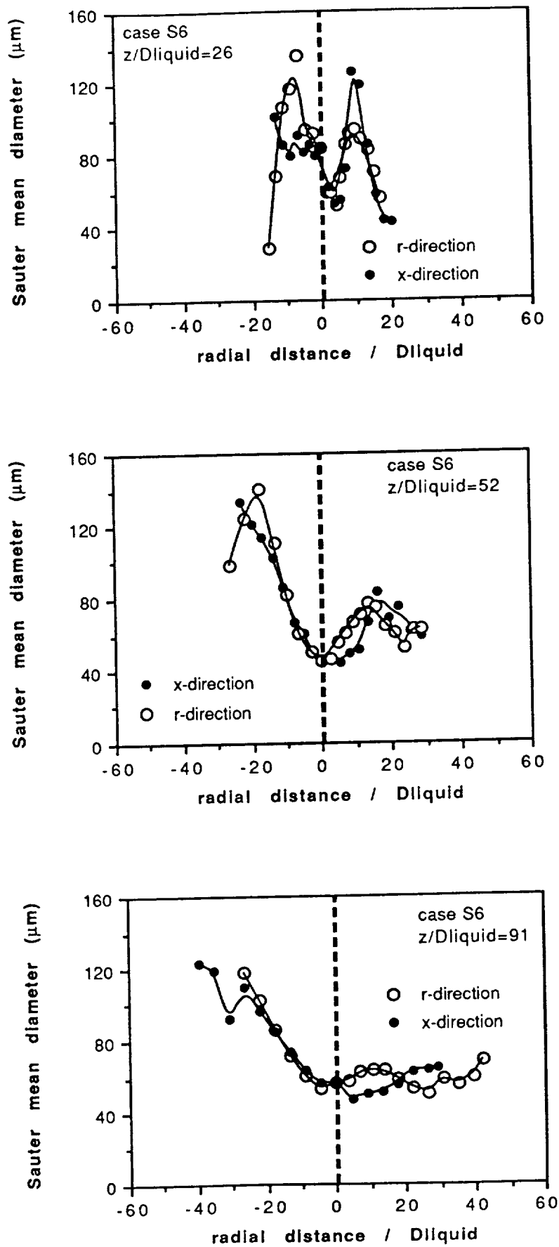
Figure 14. Characteristics of sprays produced by high swirl number gaseous stream nozzles with 3 mm annulus. Conditions according to case S6 of table 3. Radial profiles at z/D_{\text{liquid}} = 26, 52 and 91 of (a) Sauter mean diameter and (b) liquid flux normalised by the measured maximum value for each axial location.
