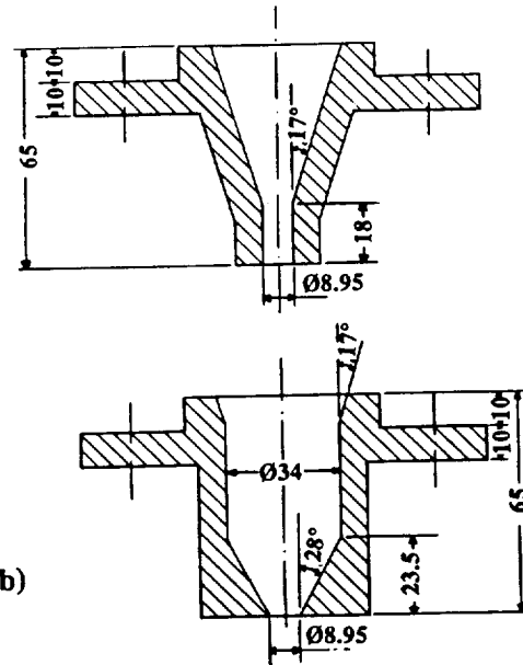
Figure 1. (a) Experimental arrangement of the coaxial atomizer with 10 mm annular width; (b) nozzles used for the coaxial atomizers with 3 mm annular widths with straight and converging exit.
