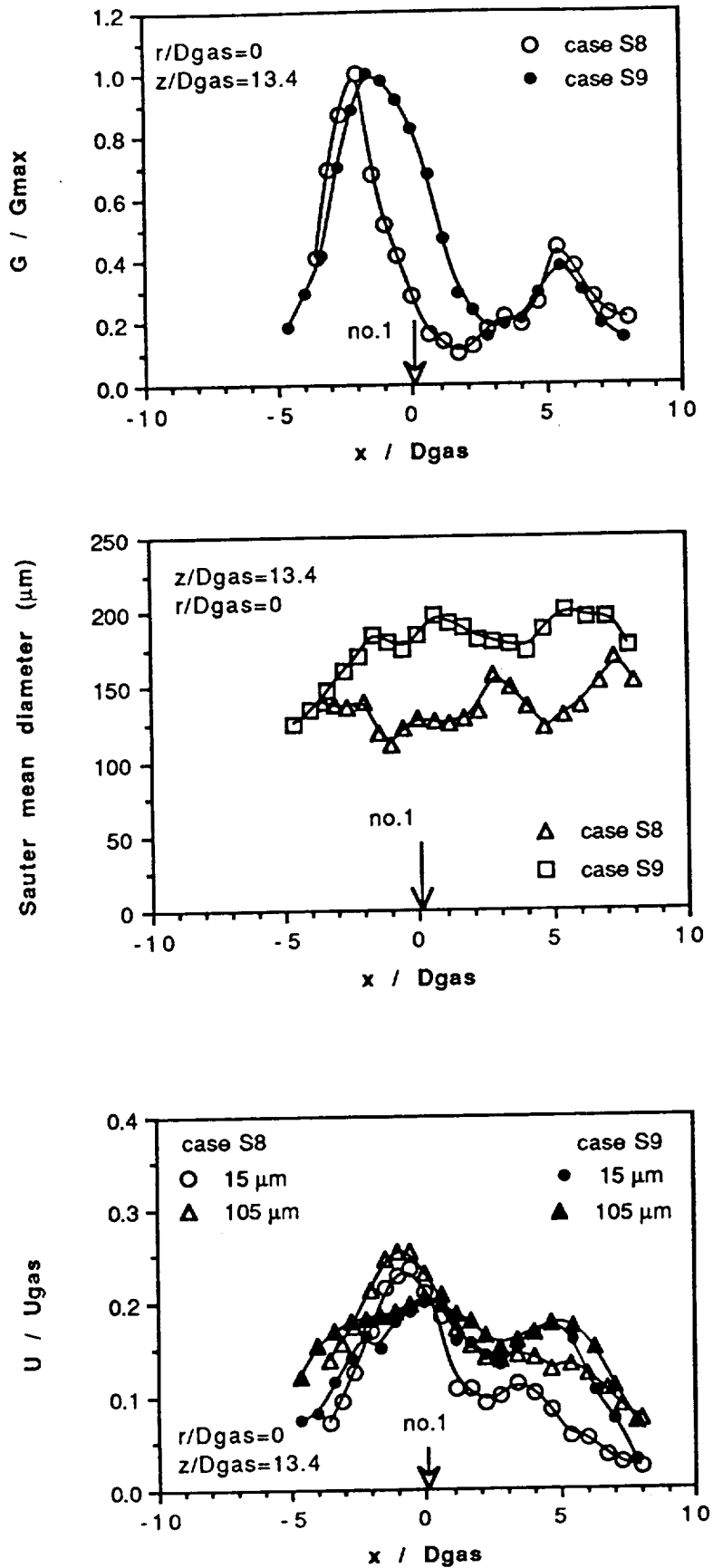
Figure 32. Comparison between the liquid flux, the Sauter mean diameter and the axial velocity of the 15 and 105 \mu m droplets of the three interacting sprays produced by nozzles with 50% differences in the liquid flowrate according to cases S8 and S9 of table 3. (a) z/D_{gas} = 13.4 , r/D_{gas}=0 ; (b) z/D_{gas}=23.5 ; x/D_{gas}=1.68 .
