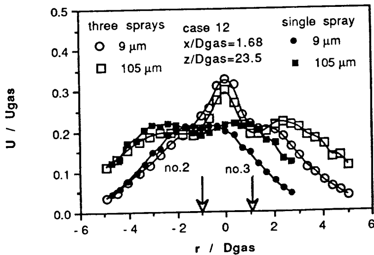
Figure 28. Comparison between the Sauter mean diameter, the liquid flux and the axial velocity of the 9 and 105 \mu\text{m} droplets of the three interacting and the single sprays produced by nozzles according to case 12 of table 1a. (a) z/D_{\text{gas}} = 23.5 , x/D_{\text{gas}} = 1.68 ; (b) z/D_{\text{gas}} = 23.5 ; r/D_{\text{gas}} = 0 .
