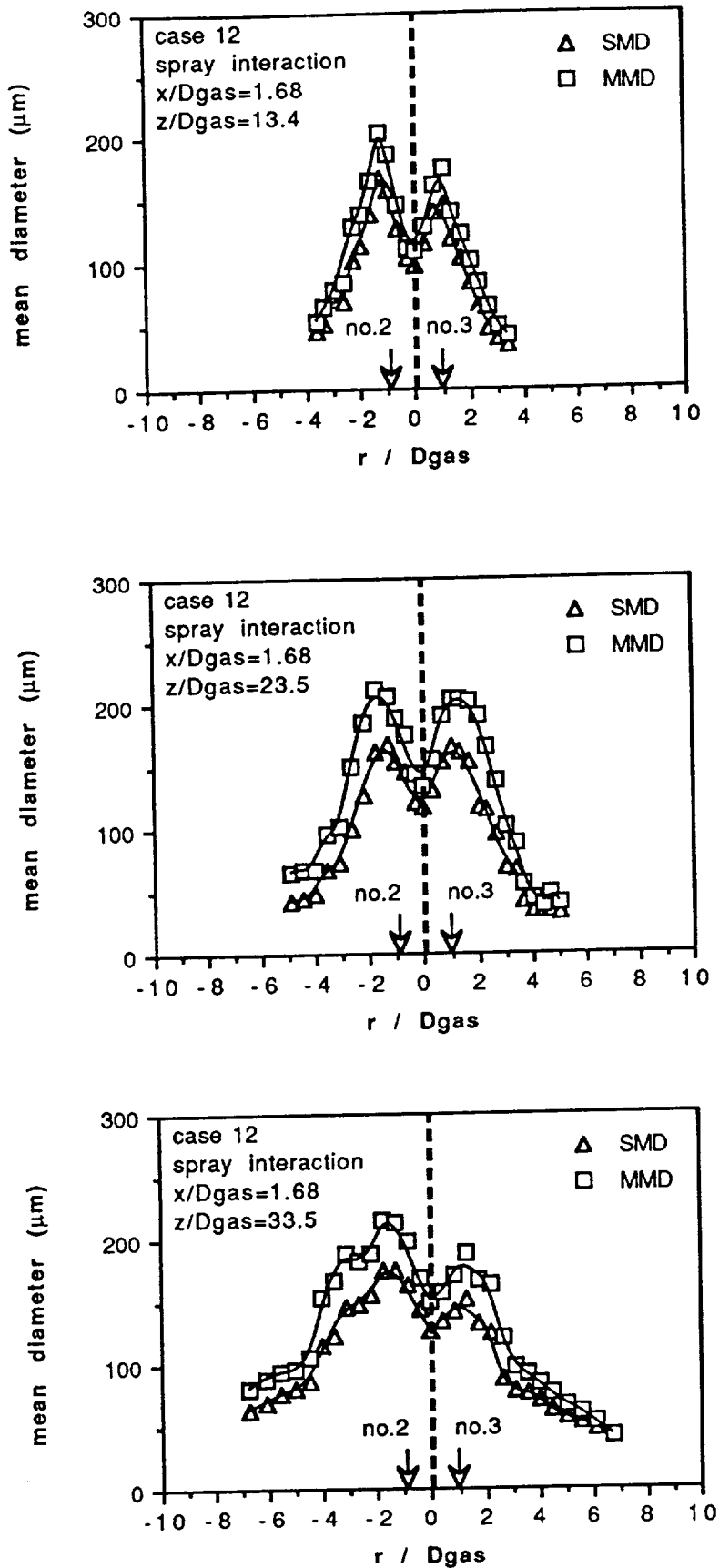
Figure 25. Radial profiles of (a) mean diameters, (b) liquid flux and (c) mean axial velocity of 9, 50 and 105 \mu\text{m} droplets and single phase at axial distances z / D_{\text{gas}} = 13.4 , 23.5 and 33.5 from the faceplate of three nozzles producing sprays according to case 12 of table 1a along the r direction at x / D_{\text{gas}} = 1.68 .
