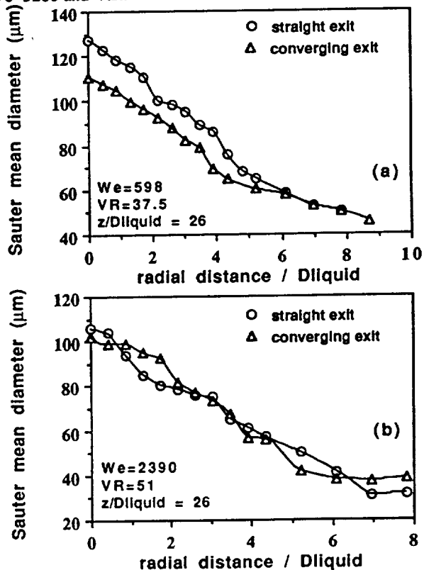
Figure 6. Radial profiles of Sauter mean diameter : D_l =2.3 mm with the straight and converging exit nozzle with D_{gas} =8.95 mm at axial distance from the nozzle z/D_l =26. (a) We =598 and V.R. =37.5 (b) We =2390 and V.R. =51.
