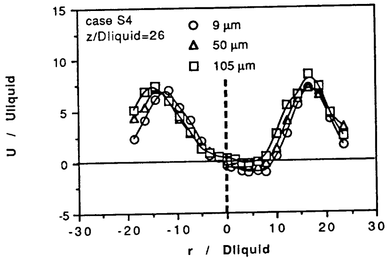
Figure 10. Characteristics of sprays produced by high swirl number gaseous stream nozzles with 10 mm annulus. Conditions according to case S4 of table 3. Radial profiles of (a) mean axial velocity of 9, 50 and 105 \mu\text{m} droplets at axial distances from the nozzle of z/D_{liquid} = 1.3 and 26 and (b) mean radial and tangential velocity of the 9, 50 and 105 \mu\text{m} droplets at z/D_{liquid} = 1.3 .
