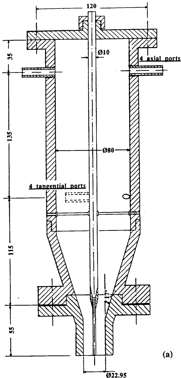
Figure 1. (a) Experimental arrangement of the coaxial atomizer with 10 mm annular width; (b) nozzles used for the coaxial atomizers with 3 mm annular widths with straight and converging exit.
