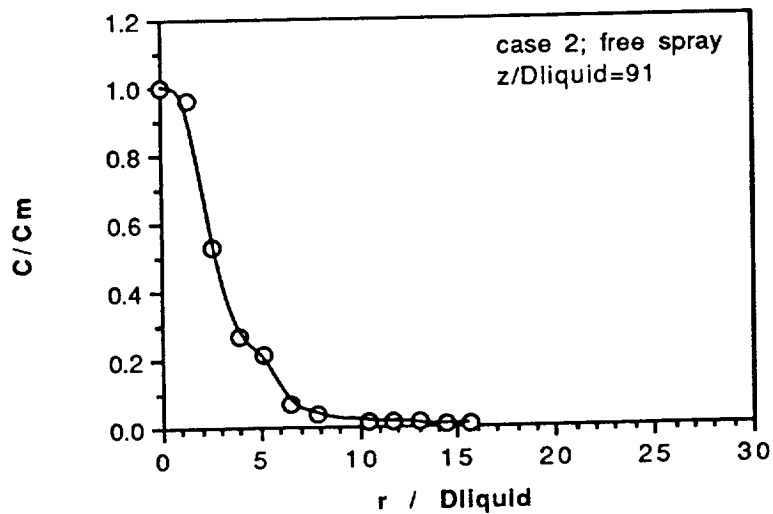
Figure 18. The characteristics of the free spray produced by a nozzle according to the conditions of case 2 of table 1a at an axial distance from the nozzle of z/D_{\text{liquid}}=91 . (a) Mean diameters; (b) normalised volume flux of the liquid content of the spray; (c) normalised concentration of the volume of liquid; (d) mean axial velocity of 9, 50 and 105 \mu\text{m} droplets and (e) rms fluctuations of the axial velocity of 9, 50 and 105 \mu\text{m} droplets.
