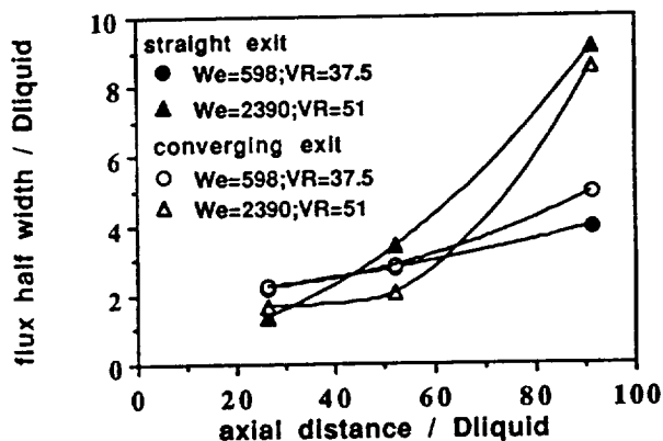
Figure 8. Flux half width of the sprays with the axial distance from the nozzle : D_l =2.3 mm with the straight and converging exit nozzle with D_{gas} =8.95 mm for We =598, V.R. =37.5 and for We =2390, V.R. =51.
