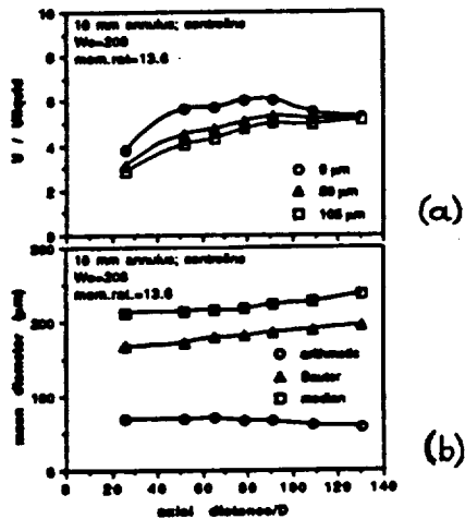
Figure 3. Centreline characteristics of a spray produced by a coaxial atomiser with annular width of 10 mm and exit Weber number=208 and gas-to-liquid momentum ratio=13.6. (a) Mean axial velocity of 9, 50 and 105 µm droplets; and (b) arithmetic, Sauter and median diameter of the droplet size distributions.
