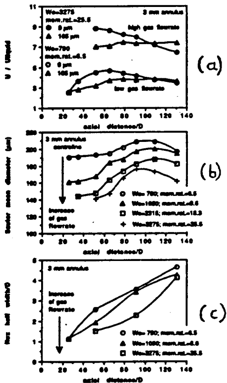
Figure 4. Influence of the gas flowrate on the spray characteristics, while the liquid flowrate remains constant. (a) Centerline development of the mean axial velocity of the 9 and 105 µm droplets; (b) centreline development of the Sauter mean diameter; and (c) change of the flux half width of the sprays with the axial distance from the nozzle.
