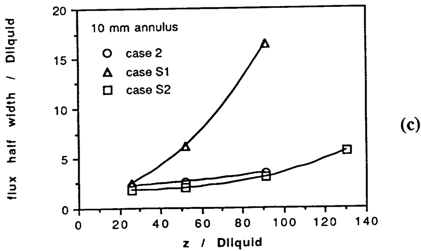
Figure 15. Comparison between the characteristics of sprays produced by axial and low swirl number gaseous stream nozzles. Centreline development of (a) Sauter mean diameter; (b) mean axial velocity of the gas phase; (c) flux half width.
