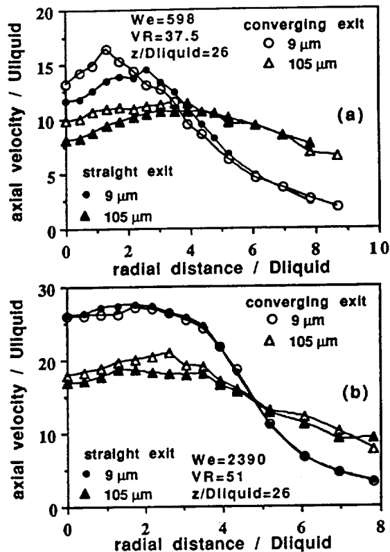
Figure 7. Radial profiles of axial velocity of 9 and 105 μm droplets : D_l =2.3 mm with the straight and converging exit nozzle with D_{gas} =8.95 mm at axial distance from the nozzle z/D_l =26. (a) We =598 and V.R. =37.5 (b) We =2390 and V.R. =51.
