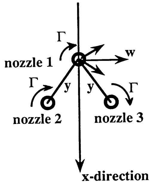
Figure 31. (a) Atomization mechanism in the three interacting sprays produced by nozzles with swirling gaseous stream. (b) The induced velocity by two irrotational vortices, nozzles 2 and 3, on the axis of the third, nozzle 1, explaining the deflection of the liquid jet.
