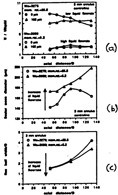
Figure 5. Influence of the liquid flowrate on the spray characteristics, while the gas flowrate remains constant. (a) Centerline development of the mean axial velocity of the 9 and 105 µm droplets; (b) centreline development of the Sauter mean diameter; and (c) change of flux half width of the sprays with the axial distance from the nozzle.
