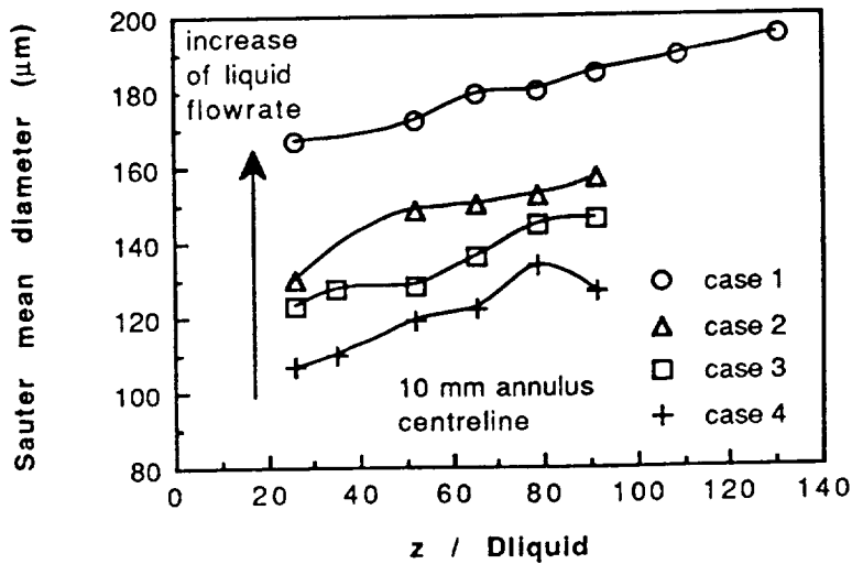
Figure 7. Effect of liquid flowrate on the characteristics of sprays produced by nozzles with 3, 6 and 10 mm annular widths. (a) Centreline development of the Sauter mean diameter; (b) Flux half width.
