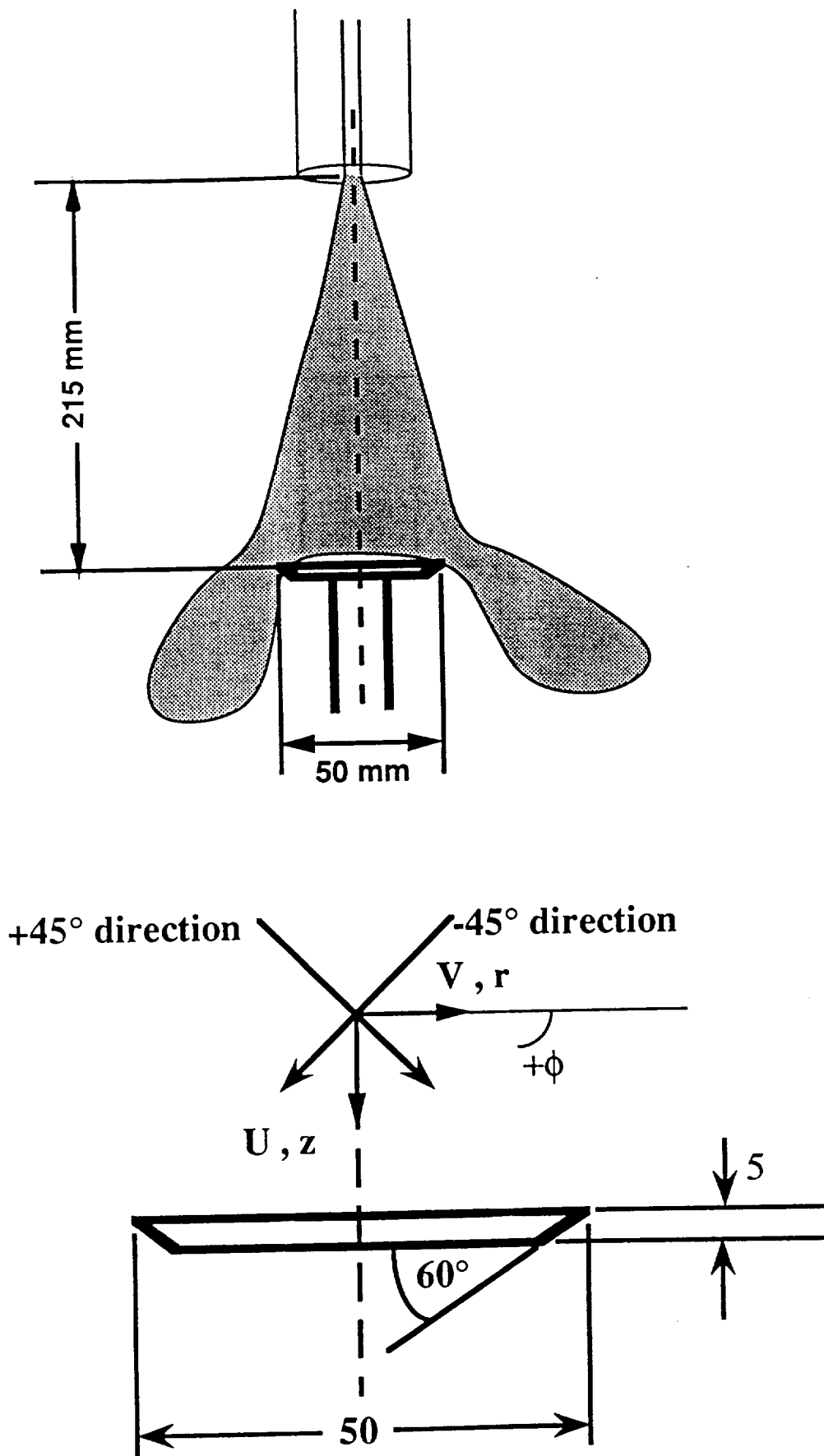
Figure 3. Experimental setup and coordinate system for the spray impingement on a flat disc.
