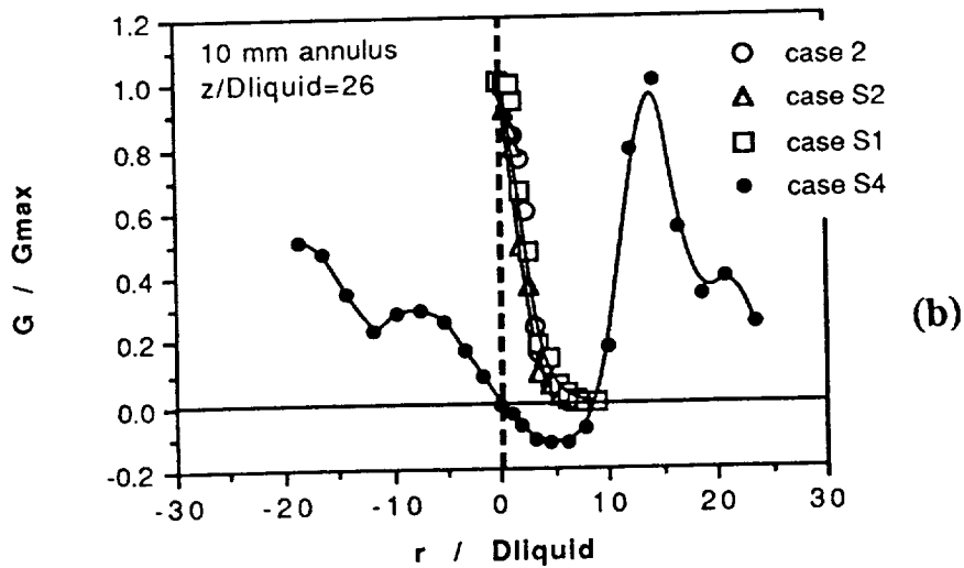
Figure 17. Comparison between the characteristics of sprays produced by axial and swirling gaseous stream nozzles. Radial profiles at z/D_{liquid} = 26 of (a) Sauter mean diameter; (b) liquid flux normalised by the maximum value of flux at the axial location.
