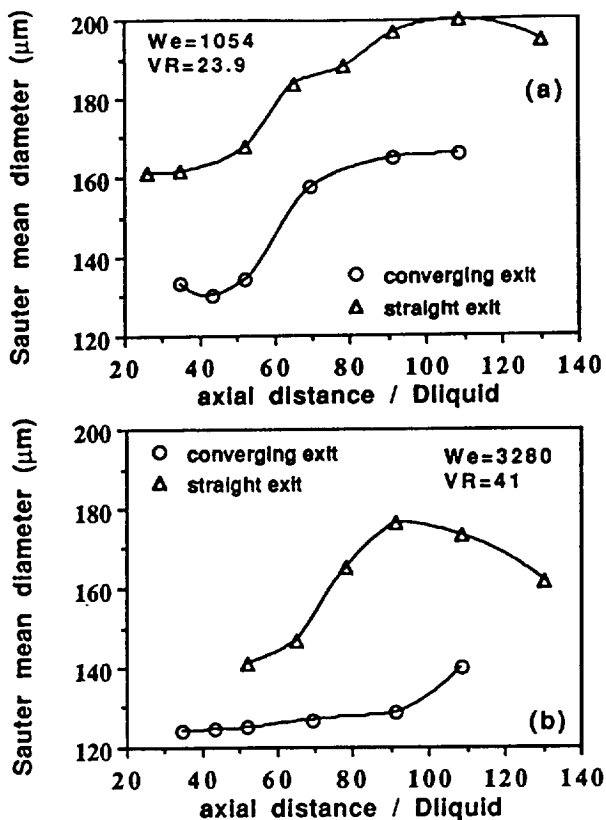
Figure 5. Centreline development of the Sauter mean diameter : D_{liquid} (or D_l ) = 2.3 mm with the straight and converging exit nozzle with D_{gas} =8.95 mm (a) We =1054 and V.R. =23.9 (b) We =3280 and V.R. =41.
