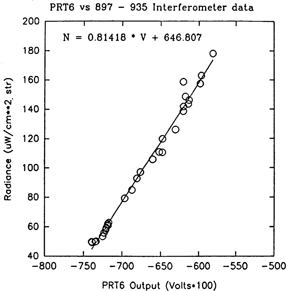
Figure 6: Calibration curve.
