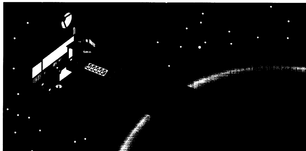
Nearly 35 percent of the computer graphics produced at the Goddard CGF, such as this colorful illustration, support the Earth Observing System (EOS) Project—NASA's centerpiece of "Mission to Planet Earth."
