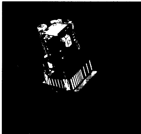
SOHO will help us understand the interactions between the Sun and the Earth's environment.
