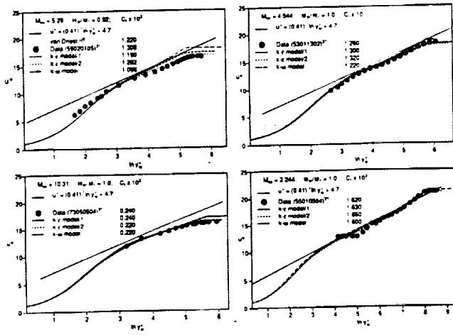
Figure 1. Comparison of calculated u^+ with measurements.
