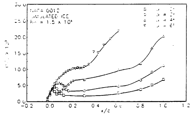
Fig. 6 Measured Momentum Thickness in the Upper Surface Separation Bubble.
