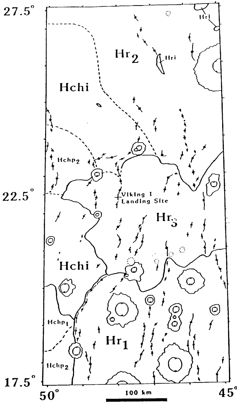
Figure 1. Generalized geologic map of the central Chryse Planitia region and the Viking 1 landing site. See text for explanation of units.
