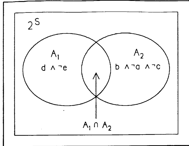
Figure 21 Restrictions on combinations of program elements
