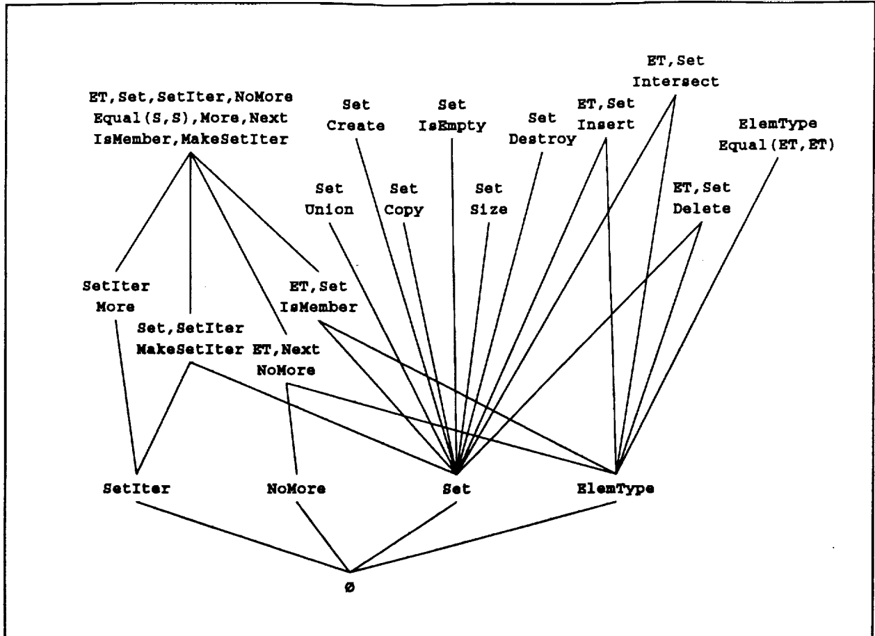
Figure 19 Poset of singleton visible elements of SetPkgTemplate (with \emptyset added)
