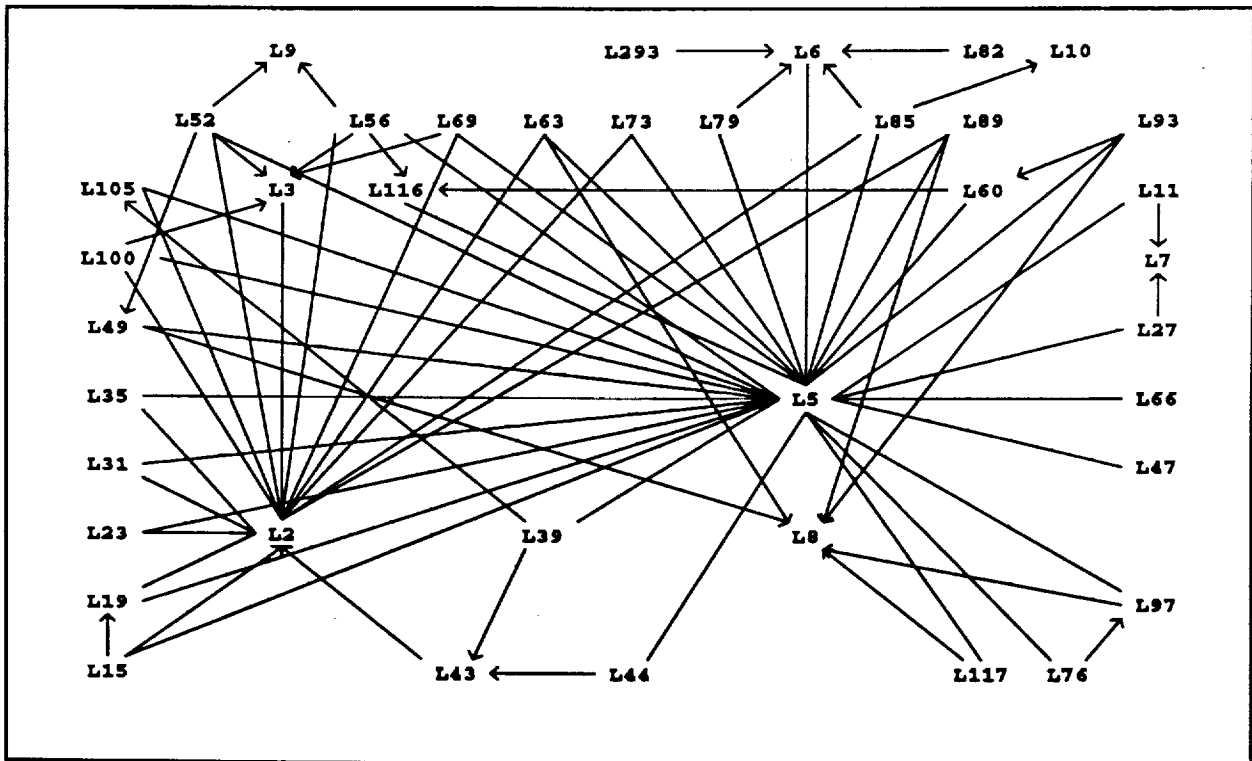
Figure 13 Interface dependence graph for ListPkgTemplate
