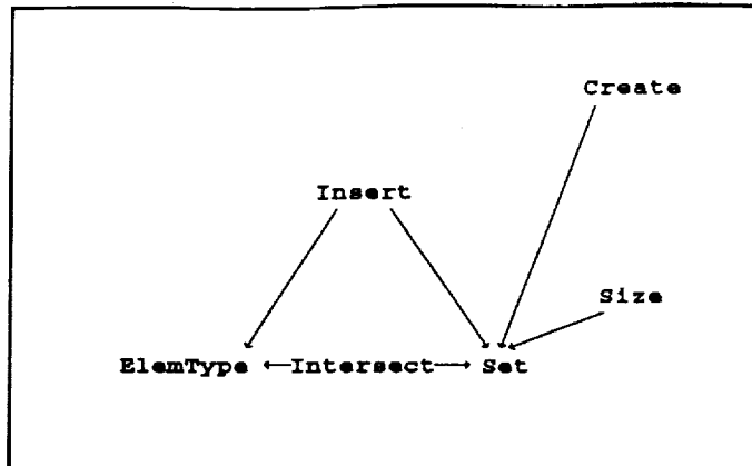
Figure 12 SetPkgTemplate sliced on \langle \text{Create}, \text{Insert}, \text{Intersect}, \text{Size}, \text{Set}, \text{ElemType} \rangle
