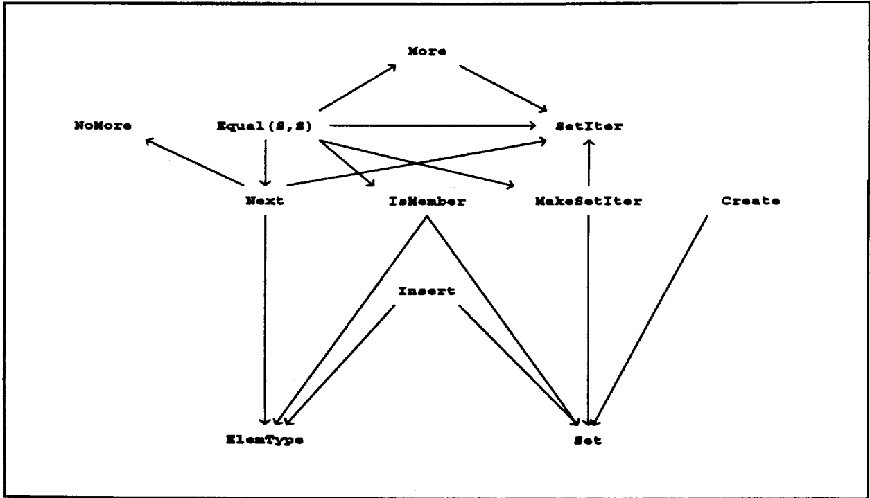
Figure 11 SetPkgTemplate sliced on \langle \text{Create, Insert, Equal, Set, ElemType} \rangle
