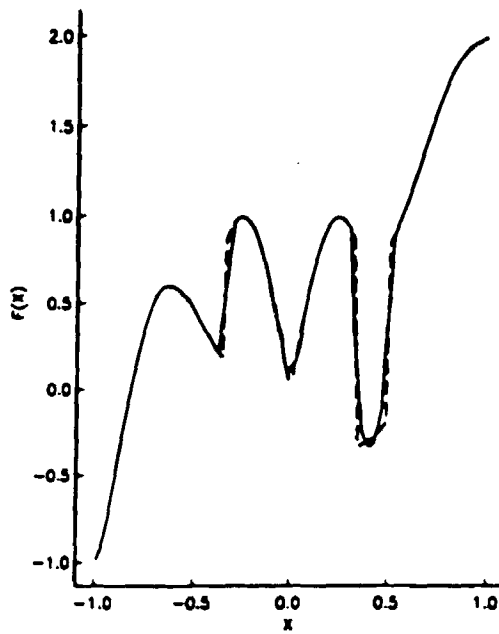
Figure 3.12: Cross-section at Y = 0 of the E.N.O. interpolation (a) and the E.N.O. reconstruction (b) for 1600 nodes the mesh. 46
