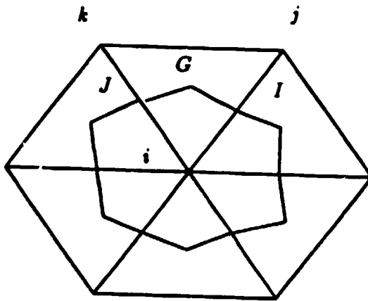
Figure 2.2: Control volume around i
