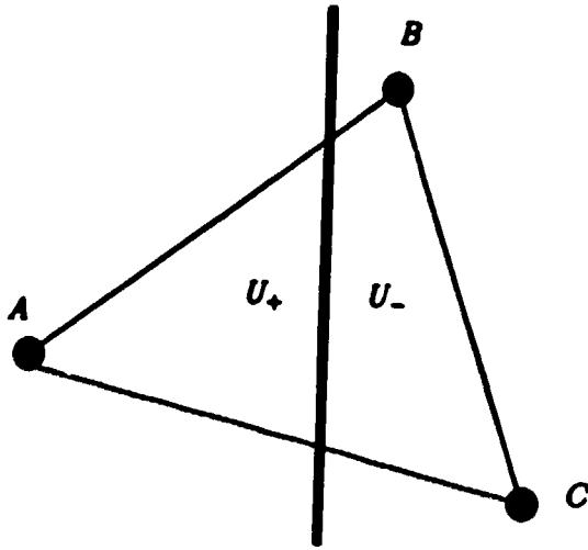
Figure 2.1: Stencil and discontinuity curve
