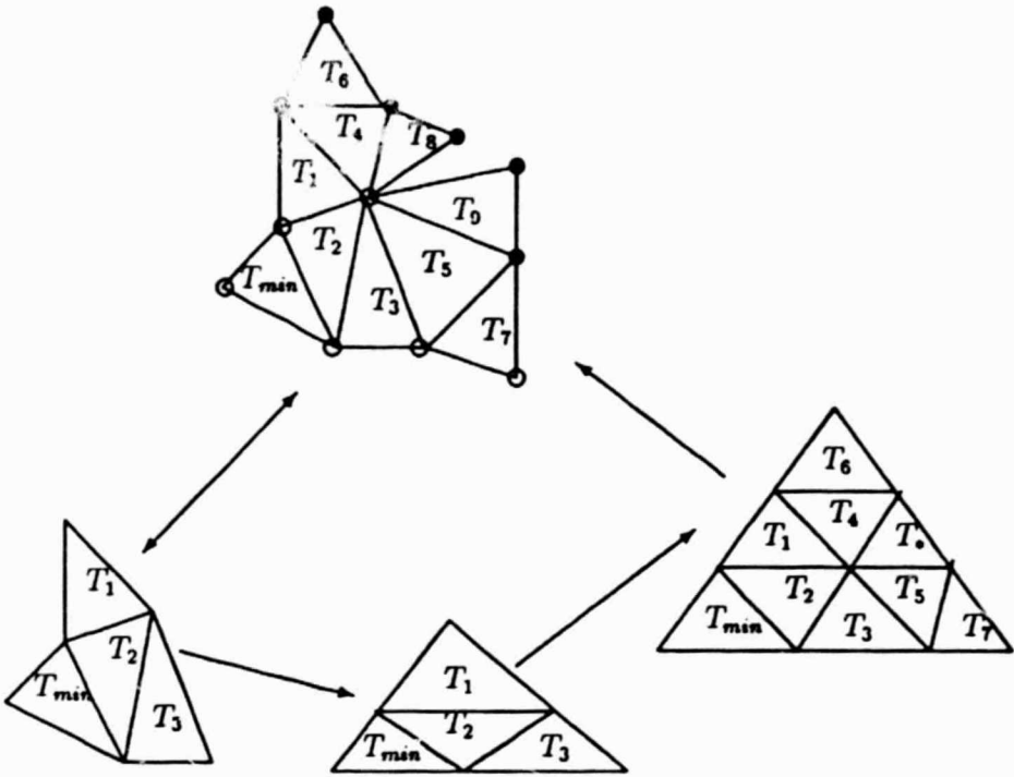
Figure 2.4: Construction of a stencil for fourth order approximation : the black circles represent the points to be added to a stencil for third order approximation (circles). The standard P_3 stencil is shown.
