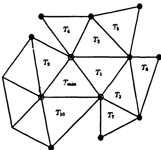
Figure 2.3: Some possible interpolation points. Circles : points of T_{min} (second order interpolation), black circles : points that may be added to obtain a stencil for third order interpolation.
