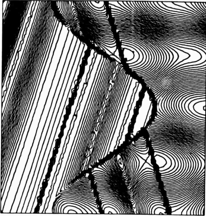
Figure 3.11: 3th order E.N.O. reconstruction with the 6400 nodes mesh from the deconvolution technique. Min=-1.325, Max=2.650, \delta = 0.8281 \cdot 10^{-2} .
