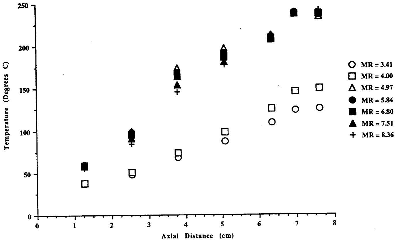
Figure 8: Inner Wall Thermocouple Data
