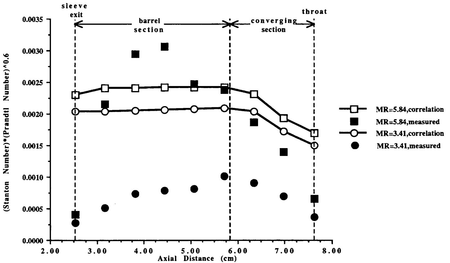
Figure 15: Stanton-Prandtl Grouping Number vs. Axial Distance Laminar Pipe Flow Correlation and Measured Values
