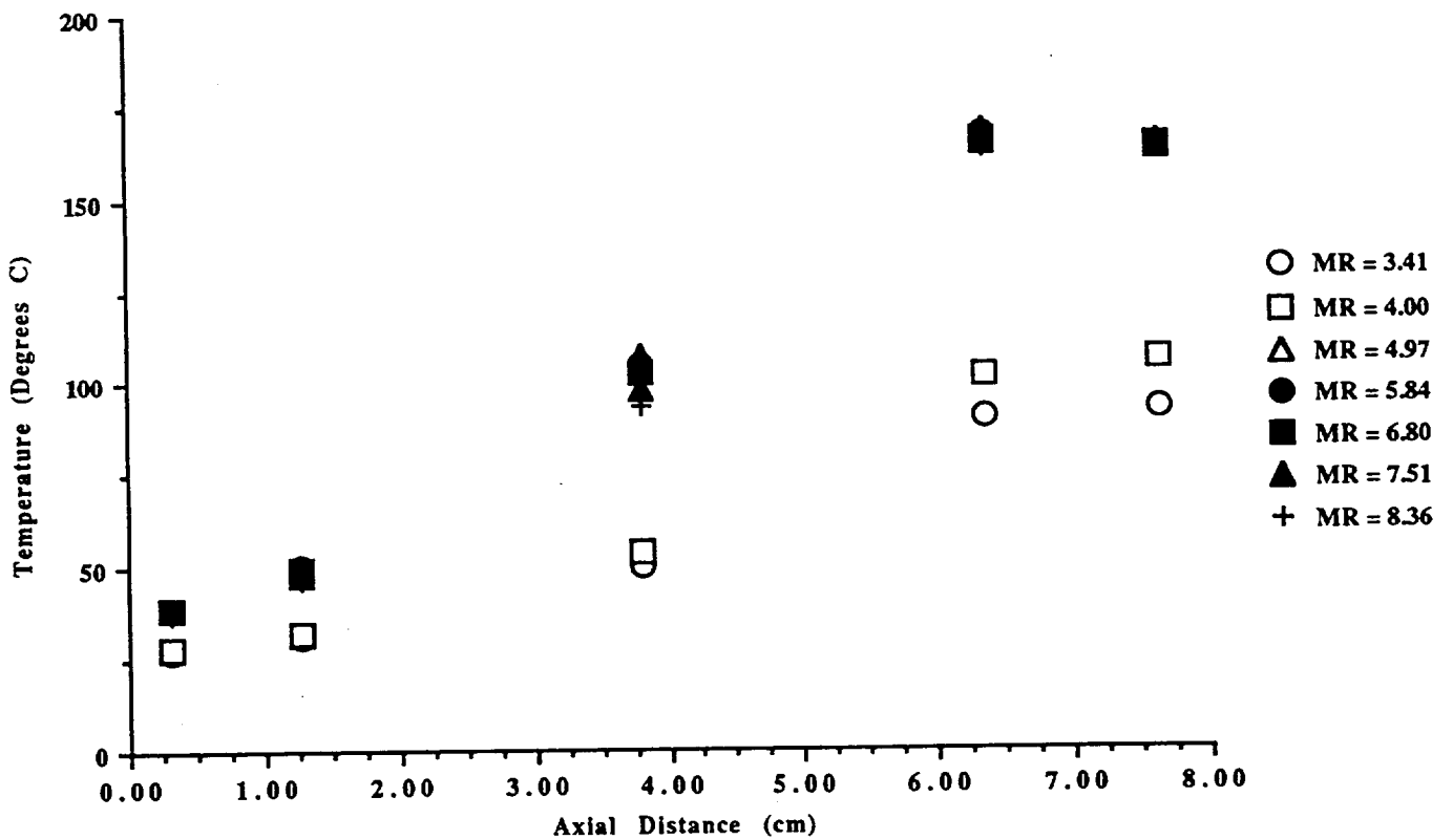
Figure 9: Outer Wall Thermocouple Data
