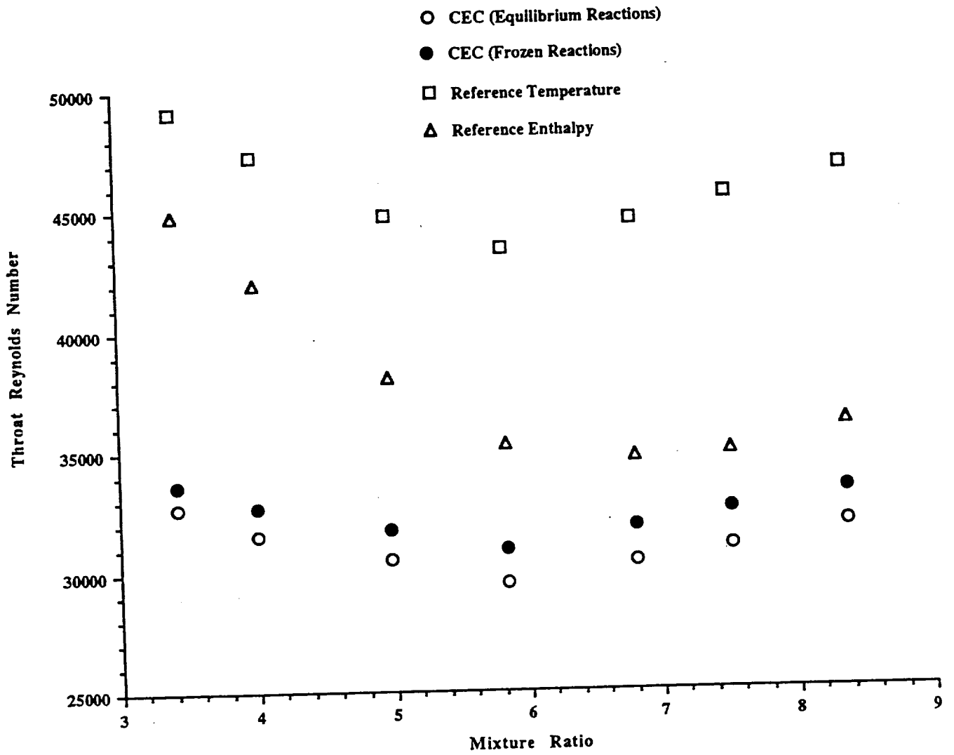
Figure 16: Throat Reynolds Number vs. Mixture Ratio
