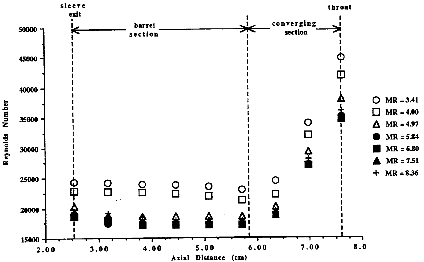
Figure 13: Reynolds Number vs. Axial Distance Viscosity Evaluated at Reference Properties
