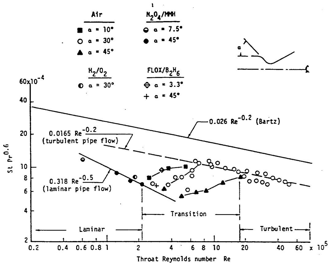
Figure 1: Heat Transfer vs. Throat Reynolds Number 12
