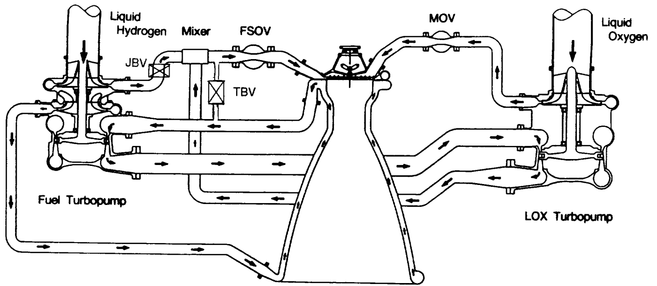
Figure 7. Split-Expander Cycle
