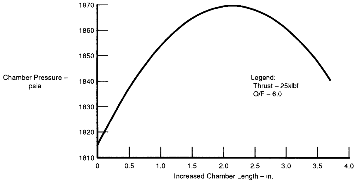
Figure 30. Advanced Split-Expander Cycle P_c Improvement Due to Increased Chamber Length
