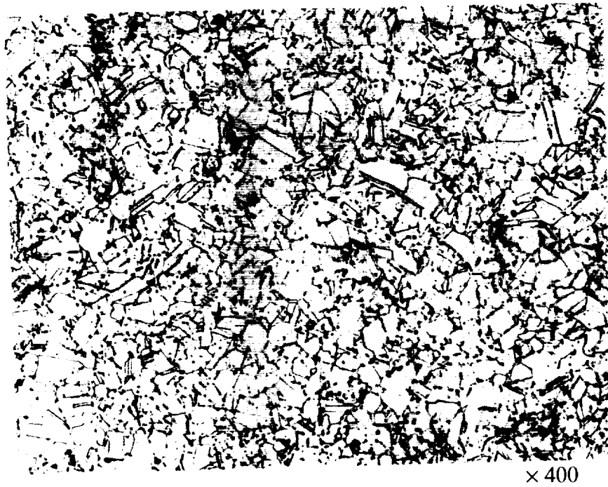
Figure 6. Grain structure in cold-worked Inconel 718.
