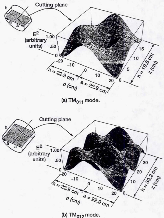
Figure 2.—Resonant electric power density contour.
