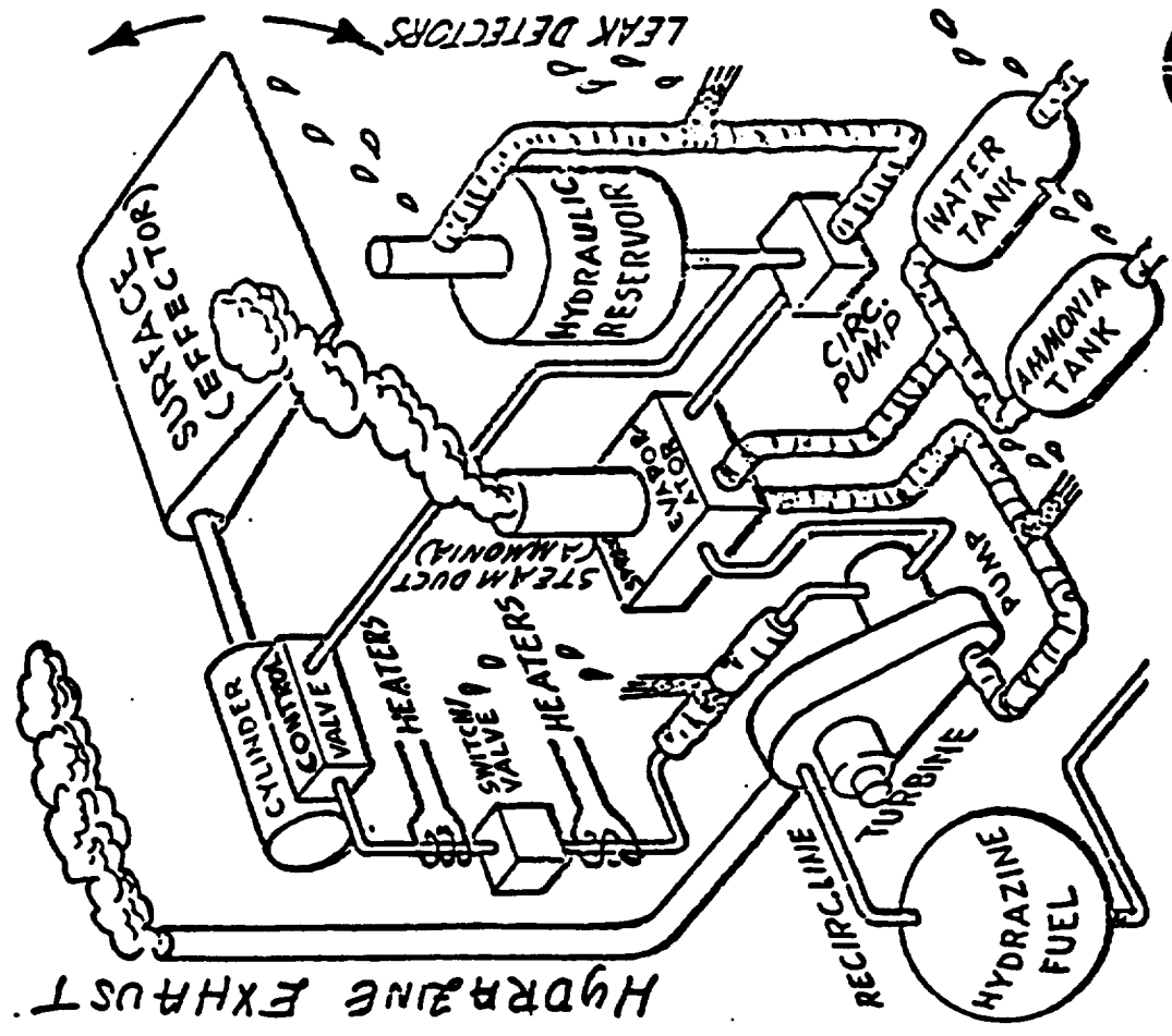
HYDRAULIC (PRESENT)
