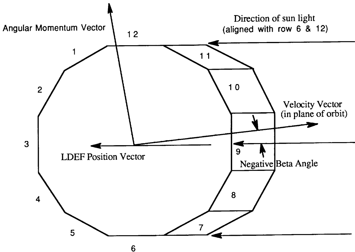
Figure 4. Alignment of yaw and beta angles near sunrise.
