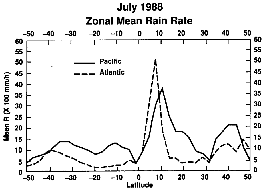
c) Monthly mean zonally averaged rain rate (mm/h x 100) for the Atlantic and Pacific Oceans derived from SSM/I July 1988 measurements at 19-, 37-, and 85- GHz.
