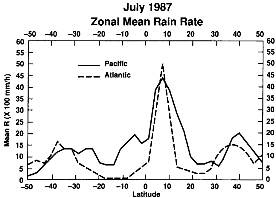
Fig. 11: a) Monthly mean zonally averaged rain rate (mm/h x 100) for the Atlantic and Pacific Oceans derived from SSM/I July 1987 measurements at 19-, 37-, and 85- GHz.
