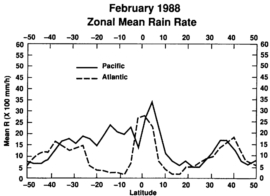
b) Monthly mean zonally averaged rain rate (mm/h x 100) for the Atlantic and Pacific Oceans derived from SSM/I Feb. 1988 measurements at 19-, 37-, and 85- GHz.
