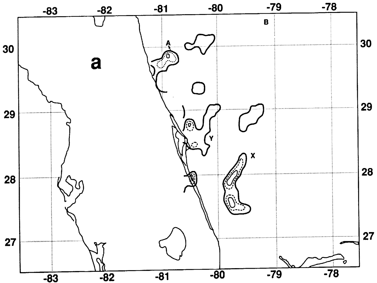
Fig. 9: Rain event of Jan. 25, 1988 (00:04 Z) over the Atlantic Ocean to the east of Florida. Letters A, B, X, and Y, adopted from Fig. 7, indicate local rain areas of interest.
