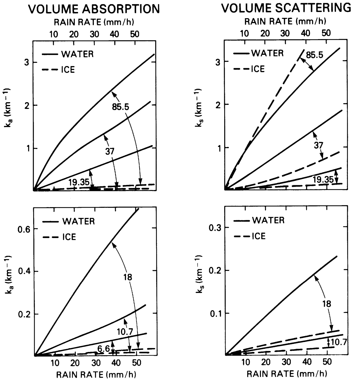
Fig. 1: Volume absorption and scattering coefficients, k_a ( \text{km}^{-1} ) and k_s ( \text{km}^{-1} ) in the microwave region between 6.6 and 85 GHz (based on: Olson, 1987, Spencer et al. , 1989).
