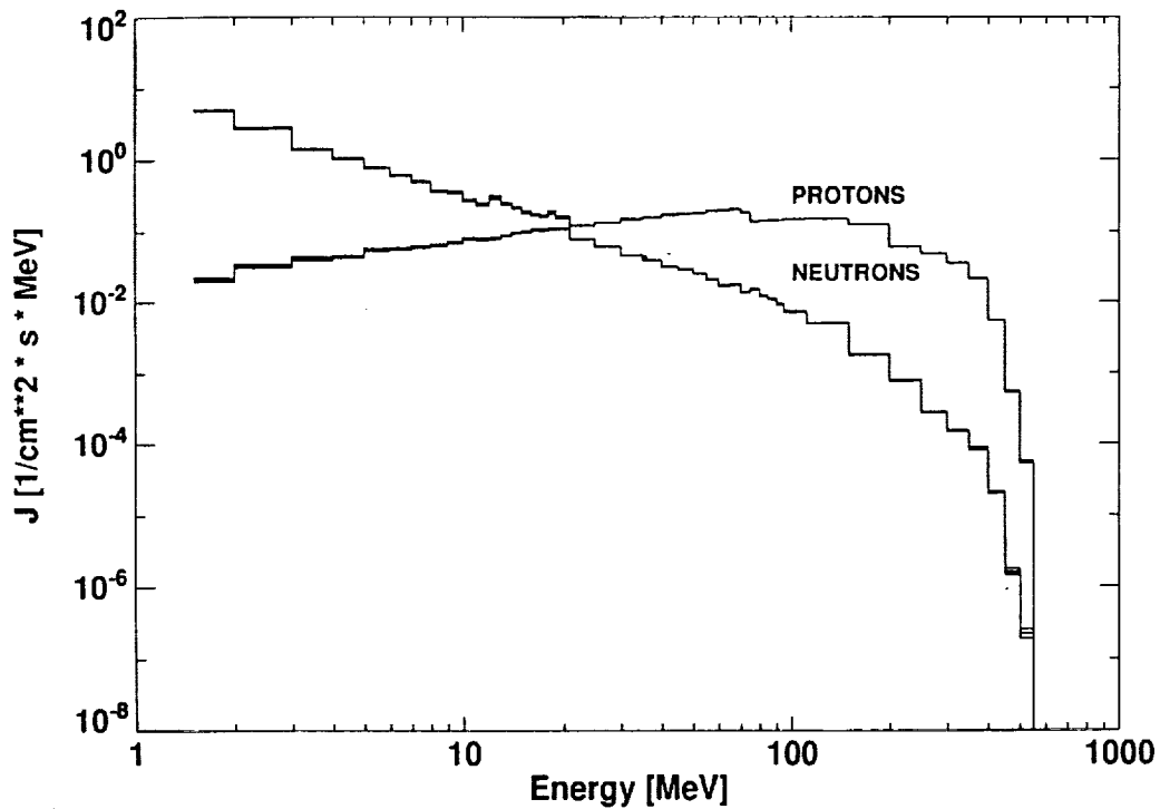
Figure 2. Proton and neutron fluxes calculated by the LAHET Code System as crossing a surface 0.59 cm ( 4.5 \text{ g/cm}^2 ) deep in a steel sphere of radius 4.125 cm ( 31.5 \text{ g/cm}^2 ). The incident flux was the geographic-east, 500-km trapped proton one from ref. 10. The fluxes of protons dominate except for energies below 20 MeV.
