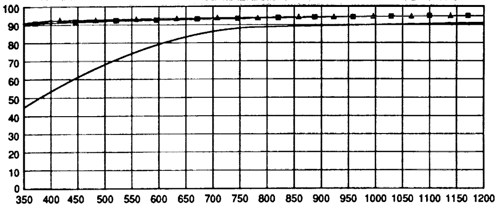
Figure 6. Spectral transmission of uncoated ULE™ sample
