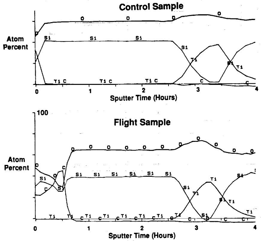
Figure 12. XPS profiles antireflection coated fused silica
