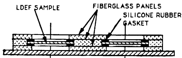
Figure 1. Sample mounting
