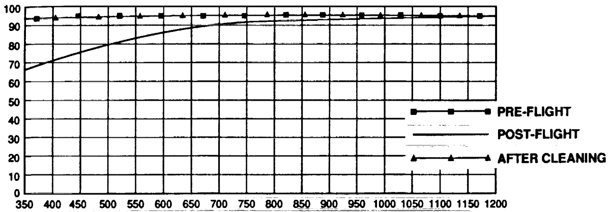
Figure 5. Spectral transmission of uncoated fused silica
