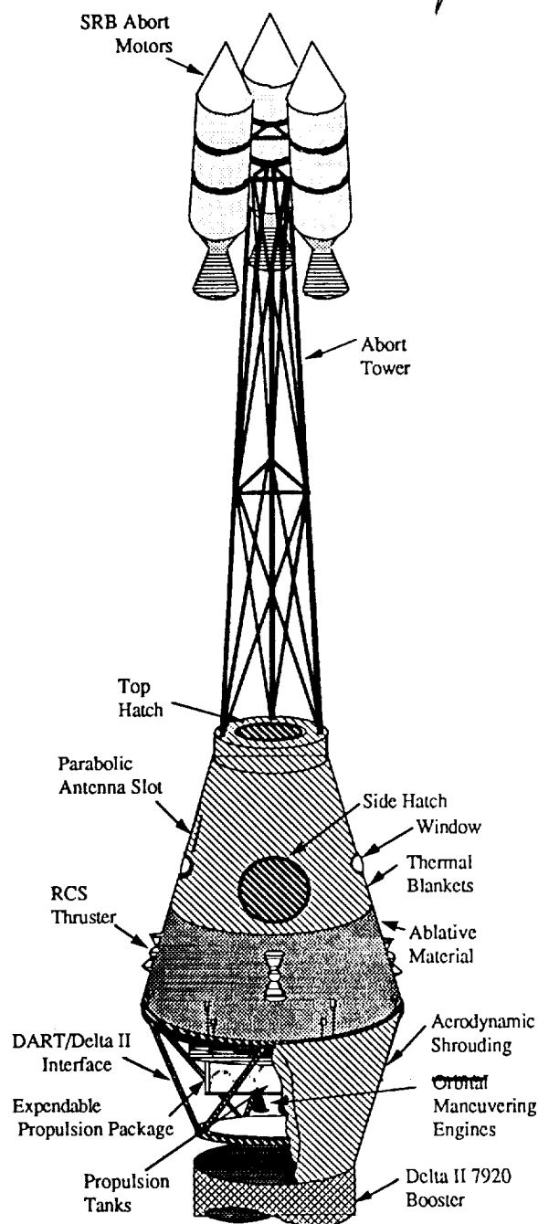
Fig. 1. DART AMS concept.
