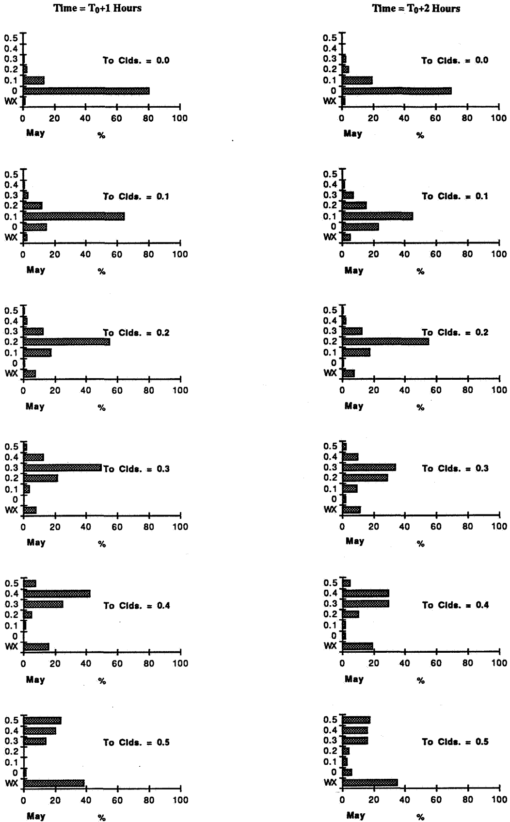
Figure G5 - Percent Occurrence of Weather Conditions for May at One and Two Hours After a Given Cloud Coverage.
