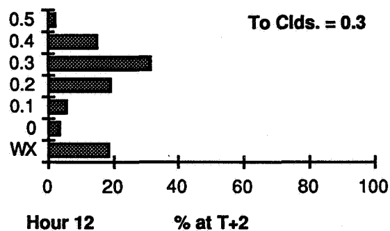
Figure 11. Percent occurrence of cloud cover and weather conditions at two hours after an initial condition of 0.2 and 0.3 cloud cover for Hour 12.
