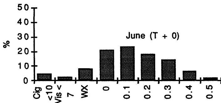
Figure 17. Climatology of weather conditions for June using complete data.
