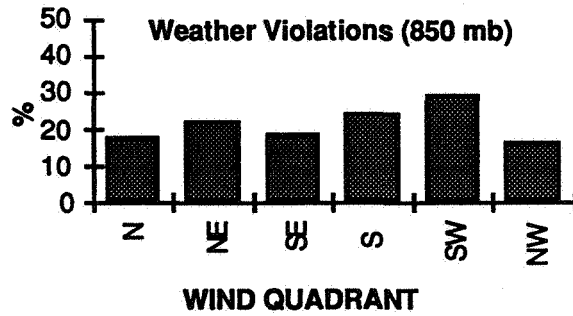
Figure 19. Percent occurrence of weather violations for 850 mb wind sectors.
