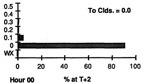
Figure 13b. Percent occurrence of cloud cover and weather conditions at two hours after an initial condition of 0.0 cloud cover for Hour 00.
