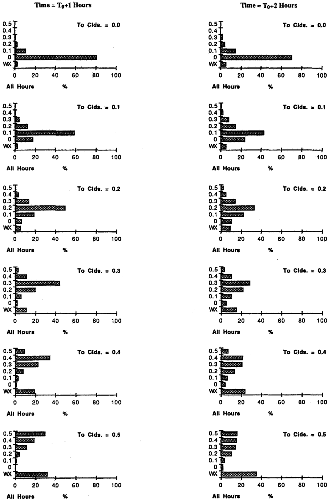
Figure B1 - All Hours View of Percent Occurrence of Weather Conditions at One and Two Hours After a Given Cloud Coverage.
