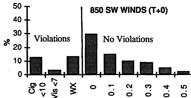
Figure 23. Percent occurrence of weather conditions for 850 mb southwest wind sector.
