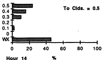
Figure E15 - Percent of Weather Violations for Hour 1400 UTC at One and Two Hours from a Given Cloud Coverage.
