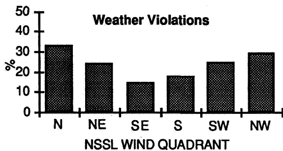
Figure 8. Percentage of weather violations by surface wind direction.
