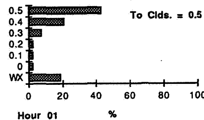
Figure E2 - Percent of Weather Conditions for Hour 0100 UTC at One and Two Hours from a Given Cloud Coverage.
