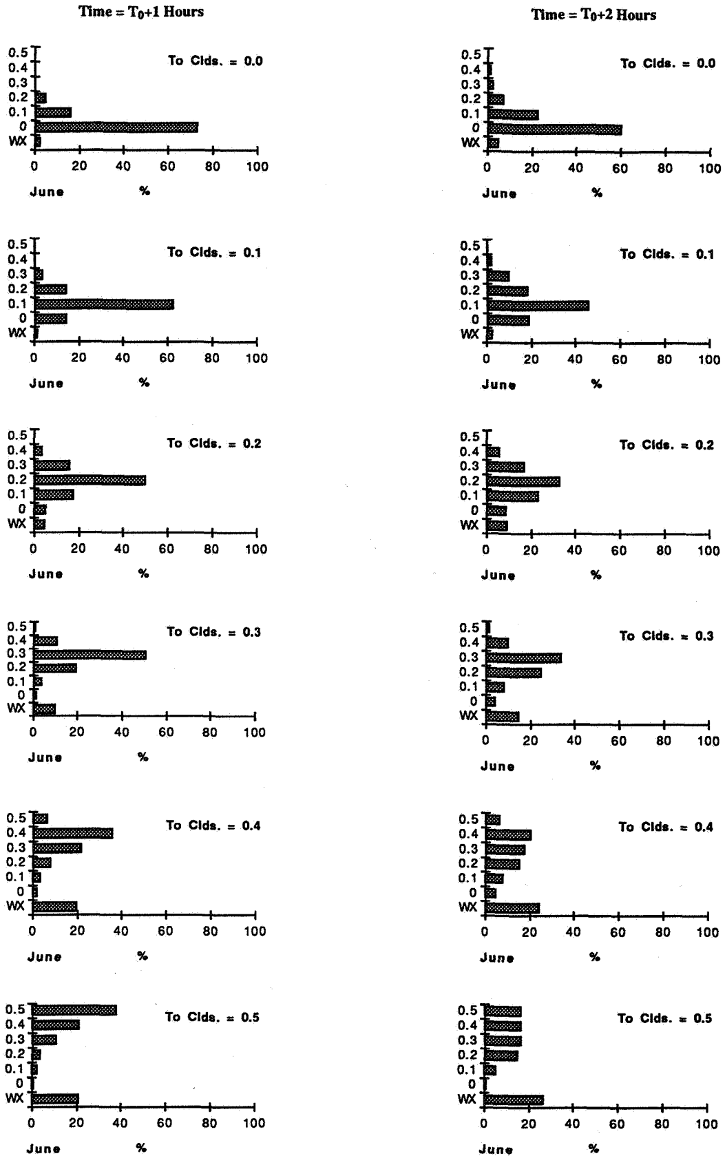
Figure D6 - Percent Occurrence of Weather Conditions for June at One and Two Hours After a Given Cloud Coverage.
