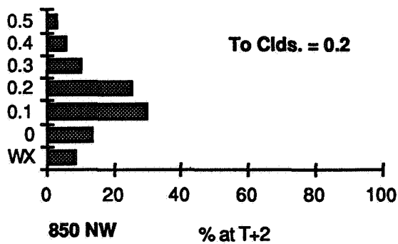
Figure 24. Percent occurrence of cloud cover and weather conditions at two hours after an initial condition of 0.2 cloud cover for 850 mb Northwest wind sector.
