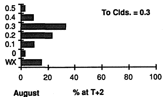
Figure 10b. Percent occurrence of cloud and weather conditions at two hours after an initial condition of 0.2 and 0.3 cloud cover.
