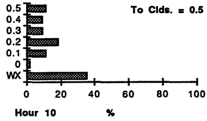
Figure E11 - Percent of Weather Conditions for Hour 1000 UTC at One and Two Hours from a Given Cloud Coverage.
