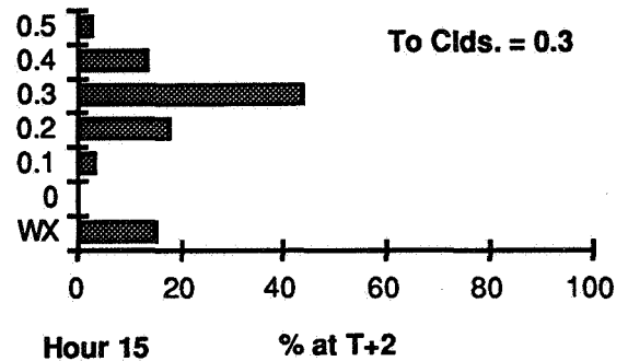
Figure 14b. Percent occurrence of cloud cover and weather conditions at two hours after an initial condition of 0.2 and 0.3 cloud cover for Hour 15.
