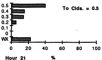
Figure E22 - Percent of Weather Conditions for Hour 2100 UTC at One and Two Hours from a Given Cloud Coverage.
