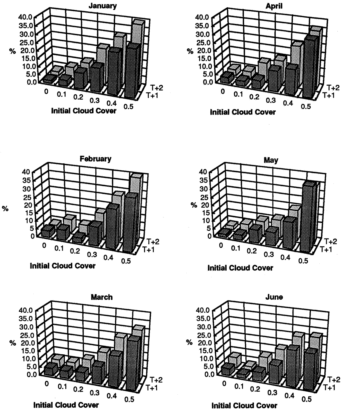
Figure H1. Percent Occurrence of Weather Violations for January to June For T+1 and T+2 Hours.
