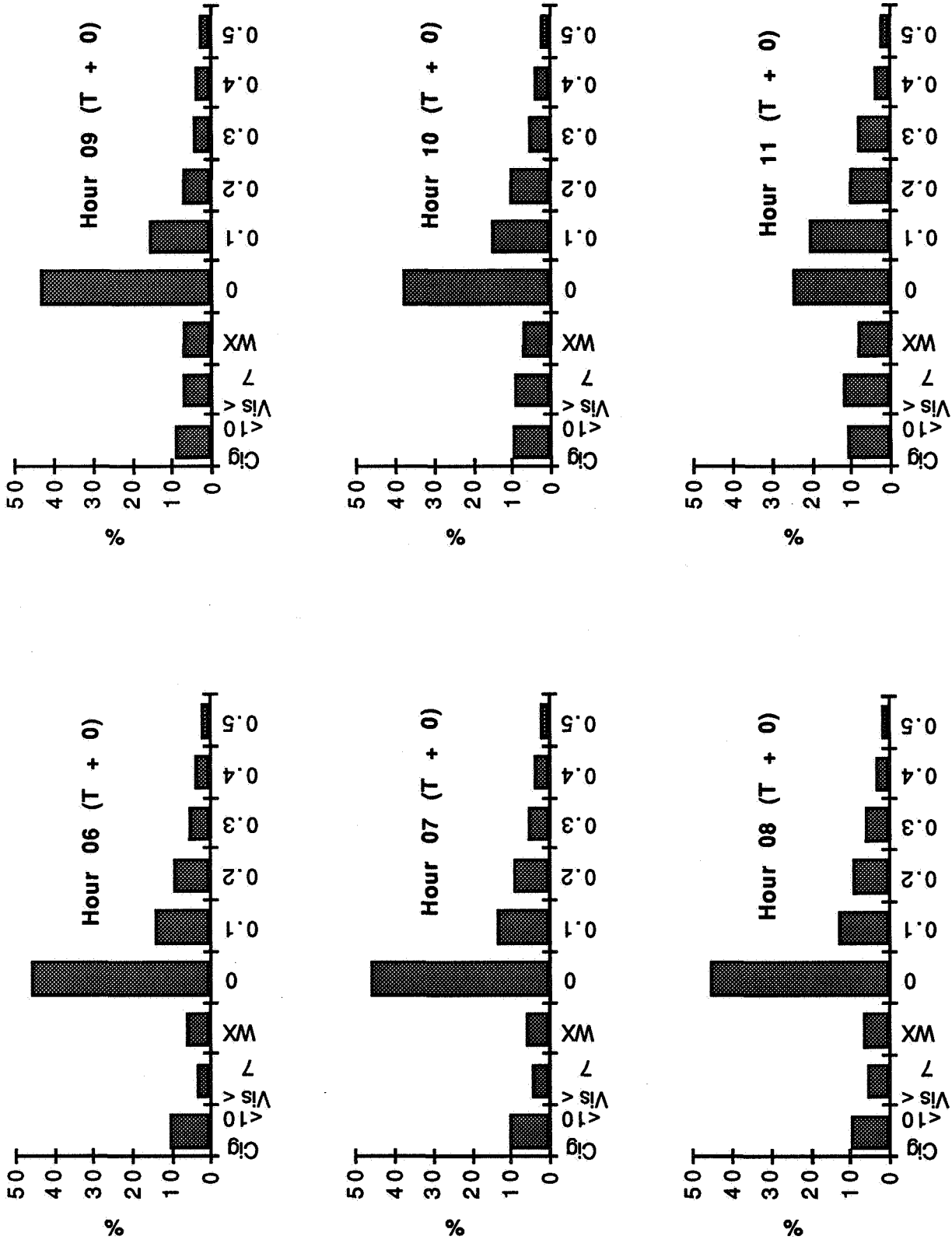
Figure A6- Percent Occurrence of Initial Weather Conditions for Hours 0600-1100 UTC for All Months and All Years.
