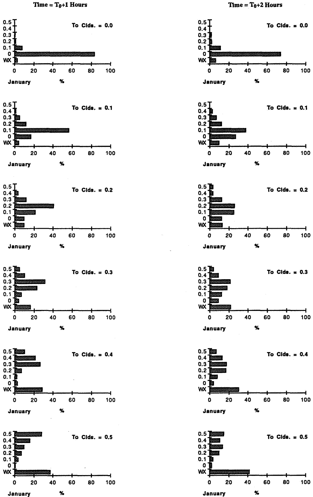
Figure D1 - Percent Occurrence of Weather Conditions for January at One and Two Hours After a Given Cloud Coverage.
