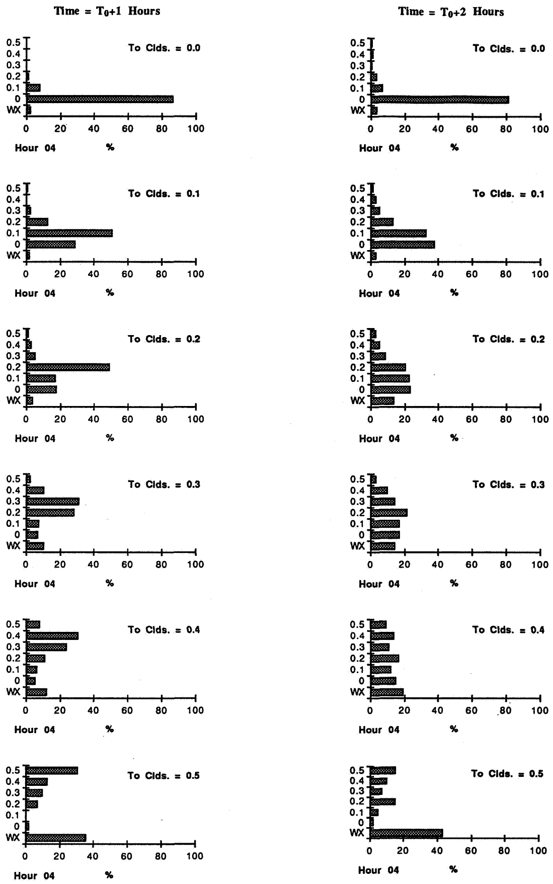
Figure E5 - Percent of Weather Conditions for Hour 0400 UTC at One and Two Hours from a Given Cloud Coverage.
