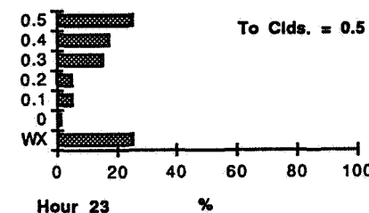
Figure E24 - Percent of Weather Conditions for Hour 2300 UTC at One and Two Hours from a Given Cloud Coverage.
