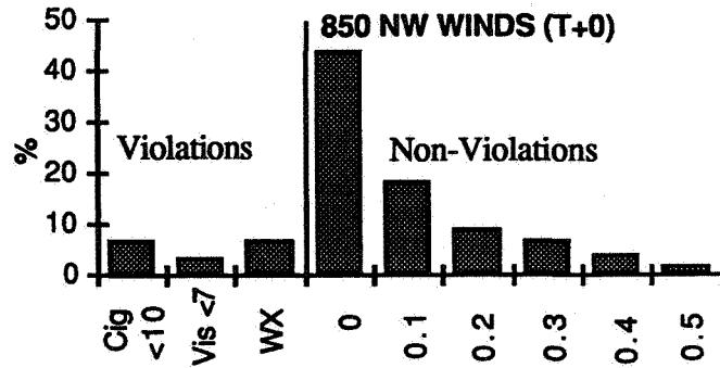
Figure 21. Percent occurrence of weather conditions for 850 mb northwest wind sector.
