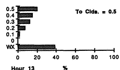
Figure E14 - Percent of Weather Conditions for Hour 1300 UTC at One and Two Hours from a Given Cloud Coverage.
