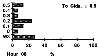
Figure E9 - Percent of Weather Conditions for Hour 0800 UTC at One and Two Hours from a Given Cloud Coverage.
