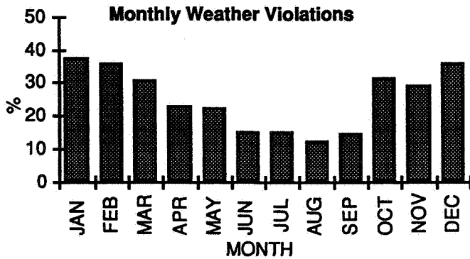
Figure 1. Percent occurrence of weather violations by month.
