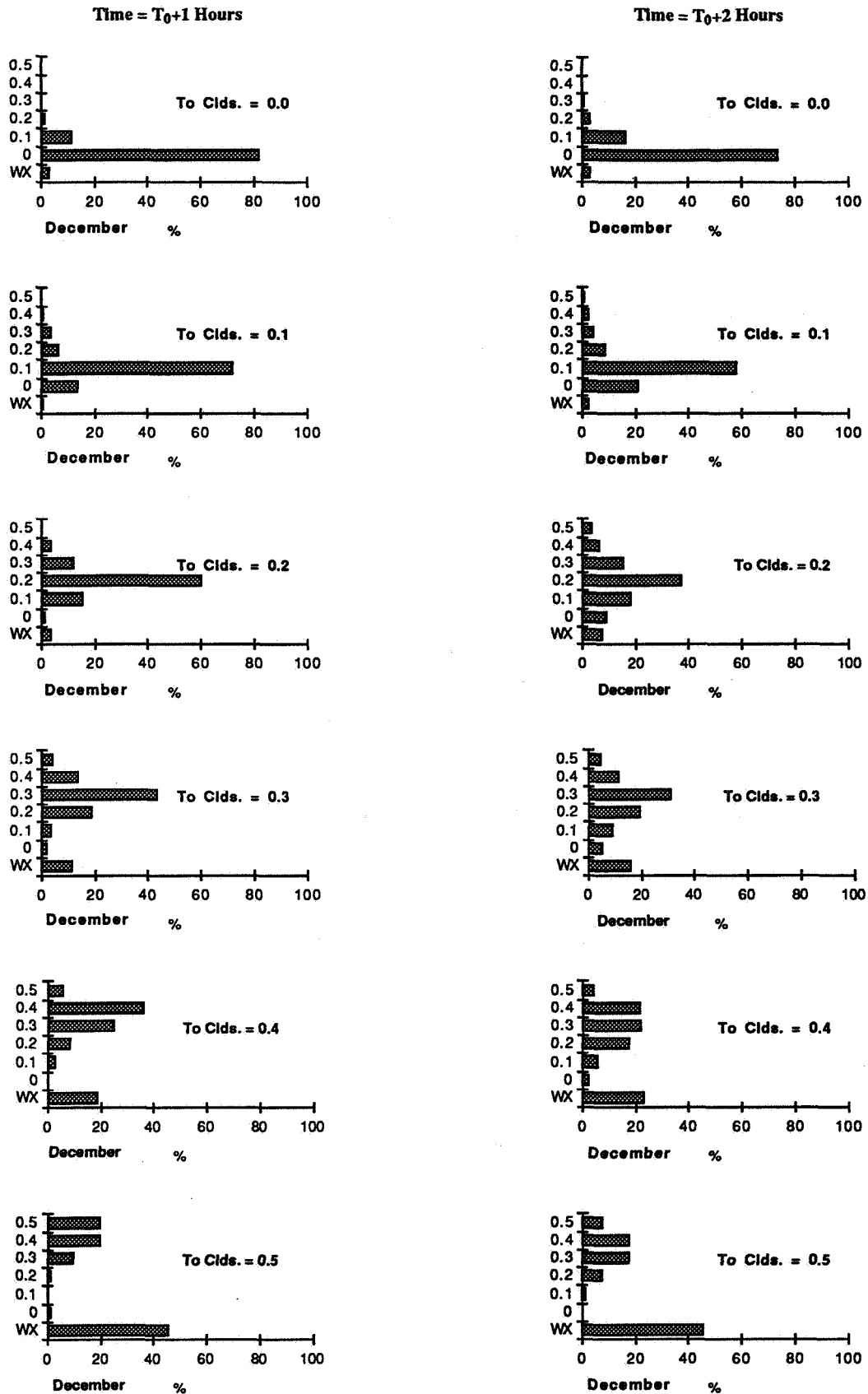
Figure G12 - Percent Occurrence of Weather Conditions for December at One and Two Hours After a Given Cloud Coverage.
