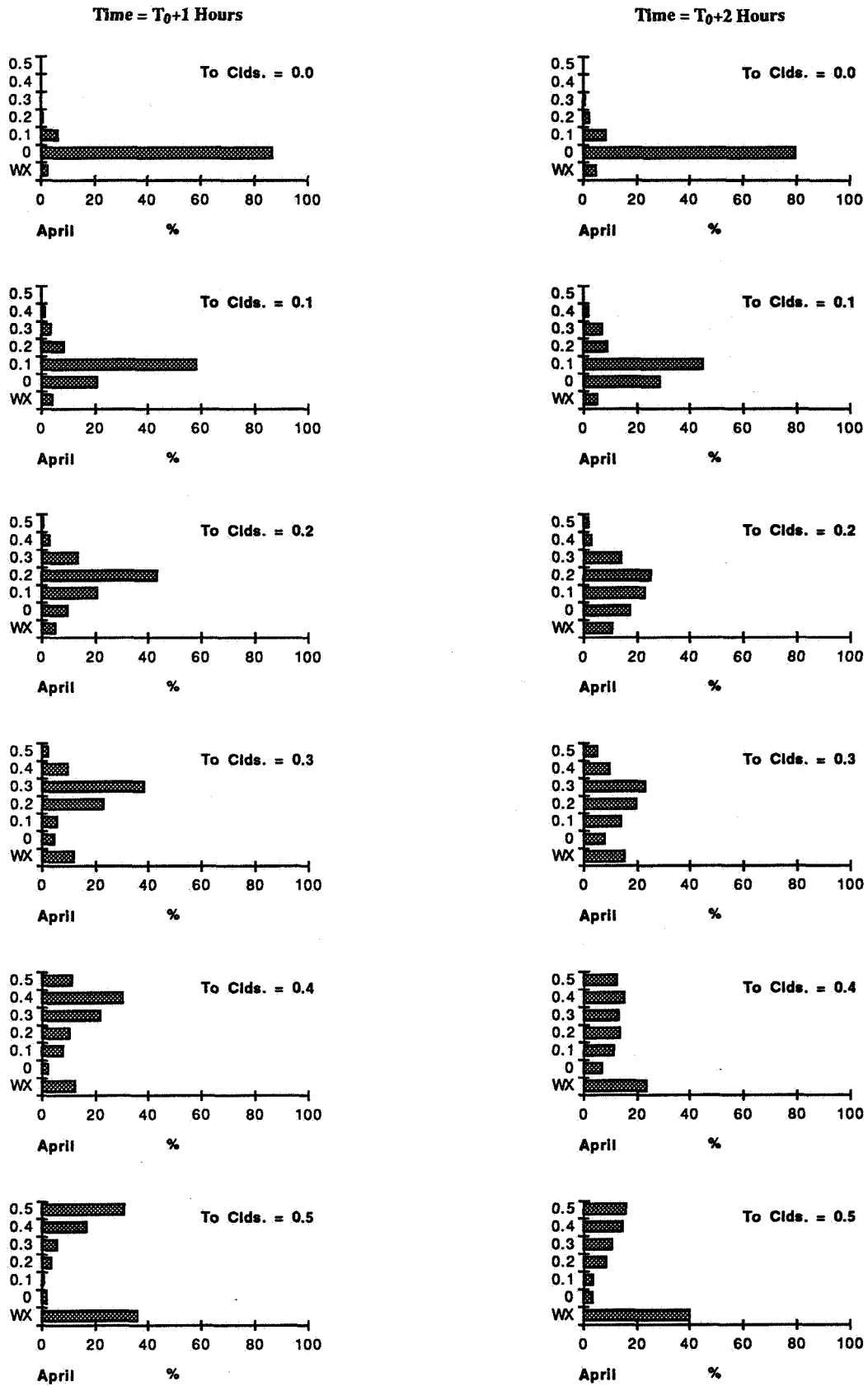
Figure D4 - Percent Occurrence of Weather Conditions for April at One and Two Hours After a Given Cloud Coverage.
