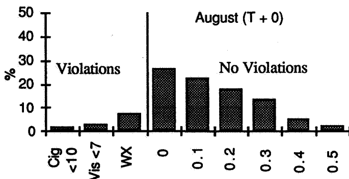
Figure 3. Percent occurrence of weather violations and cloud cover for August.
