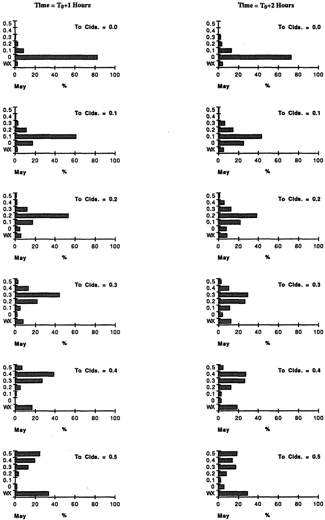
Figure D5 - Percent Occurrence of Weather Conditions for May at One and Two Hours After a Given Cloud Coverage.
