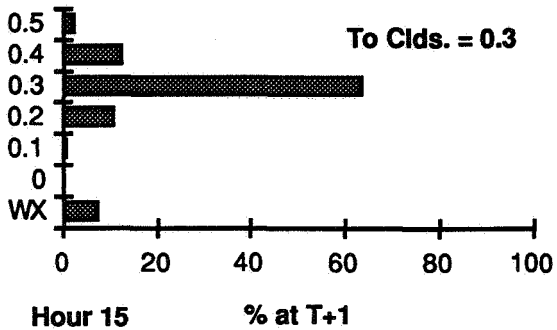
Figure 14a. Percent occurrence of cloud cover and weather conditions at one hour after an initial condition of 0.2 and 0.3 cloud cover for Hour 15.
