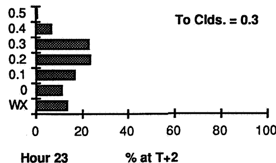
Figure 12. Percent occurrence of cloud cover and weather conditions at two hours after an initial condition of 0.2 and 0.3 cloud cover for Hour 23.
