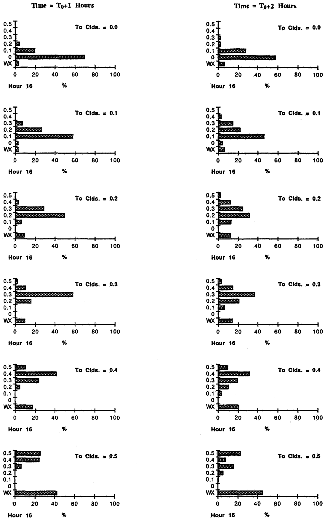
Figure E17 - Percent of Weather Conditions for Hour 1600 UTC at One and Two Hours from a Given Cloud Coverage.
