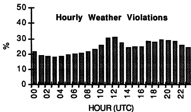
Figure 6. Percentage of hourly weather violations.
