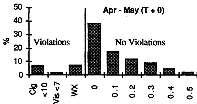
Figure 5. Percent occurrence of weather violations and cloud cover for the spring period.
