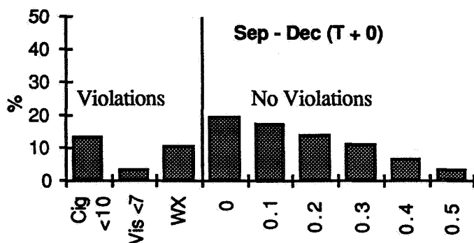
Figure 4. Percent occurrence of weather violations and cloud cover for the fall period.
