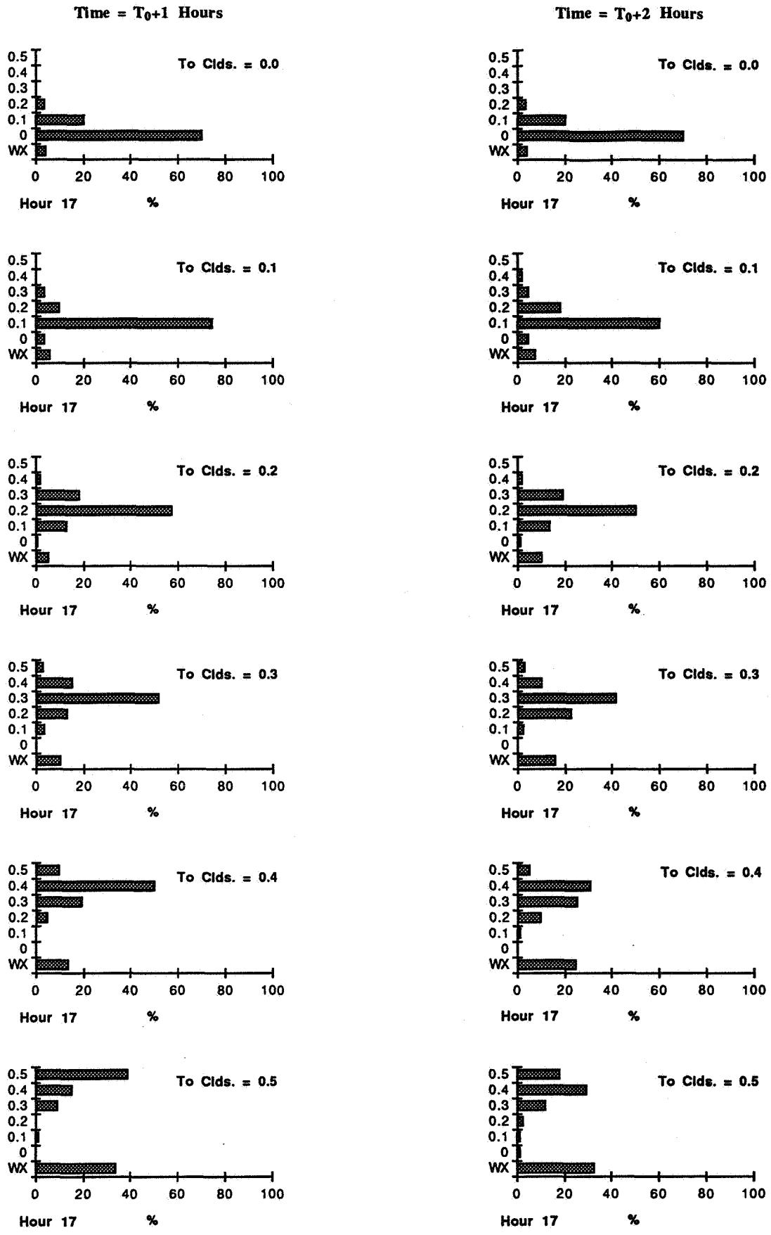
Figure E18 - Percent of Weather Conditions for Hour 1700 UTC at One and Two Hours from a Given Cloud Coverage.
