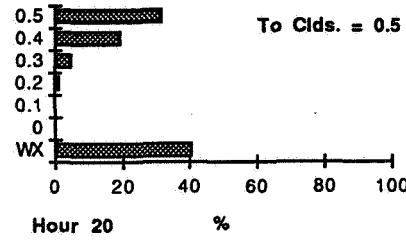
Figure E21 - Percent of Weather Conditions for Hour 2000 UTC at One and Two Hours from a Given Cloud Coverage.
