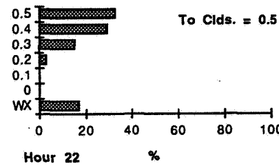
Figure E23 - Percent of Weather Conditions for Hour 2200 UTC at One and Two Hours from a Given Cloud Coverage.
