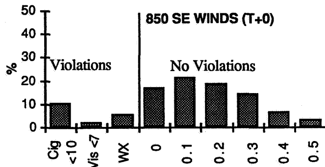
Figure 22. Percent occurrence of weather conditions for 850 mb southeast wind sector.
