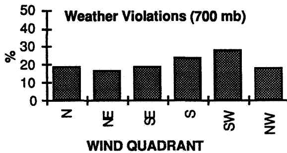
Figure 20. Percent occurrence of weather violations for 700 mb wind sectors.
