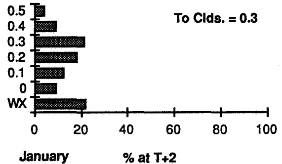
Figure 9b. Percent occurrence of cloud and weather conditions at two hours after initial condition of 0.2 and 0.3 cloud cover.
