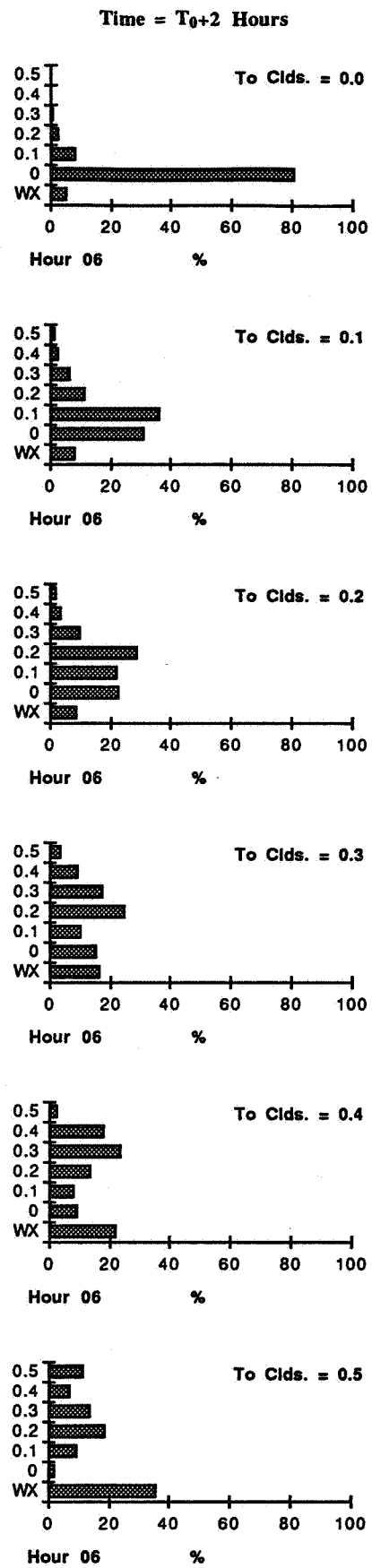
Figure E7 - Percent of Weather Conditions for Hour 0600 UTC at One and Two Hours from a Given Cloud Coverage.
