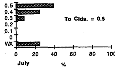
Figure G7 - Percent Occurrence of Weather Conditions for July at One and Two Hours After a Given Cloud Coverage.
