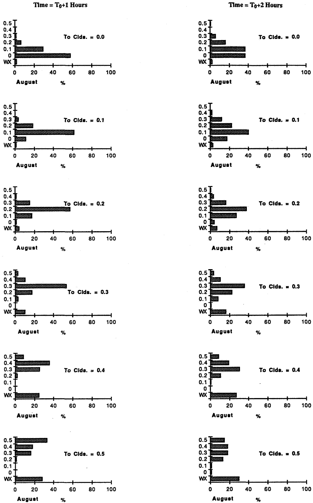
Figure G8 - Percent Occurrence of Weather Conditions for August at One and Two Hours After a Given Cloud Coverage.
