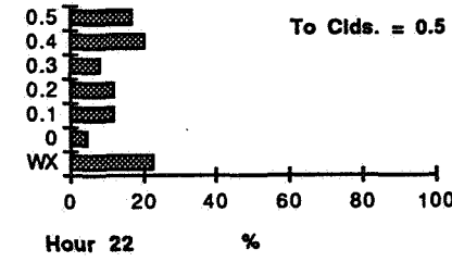
Figure E23 - Percent of Weather Conditions for Hour 2200 UTC at One and Two Hours from a Given Cloud Coverage.
