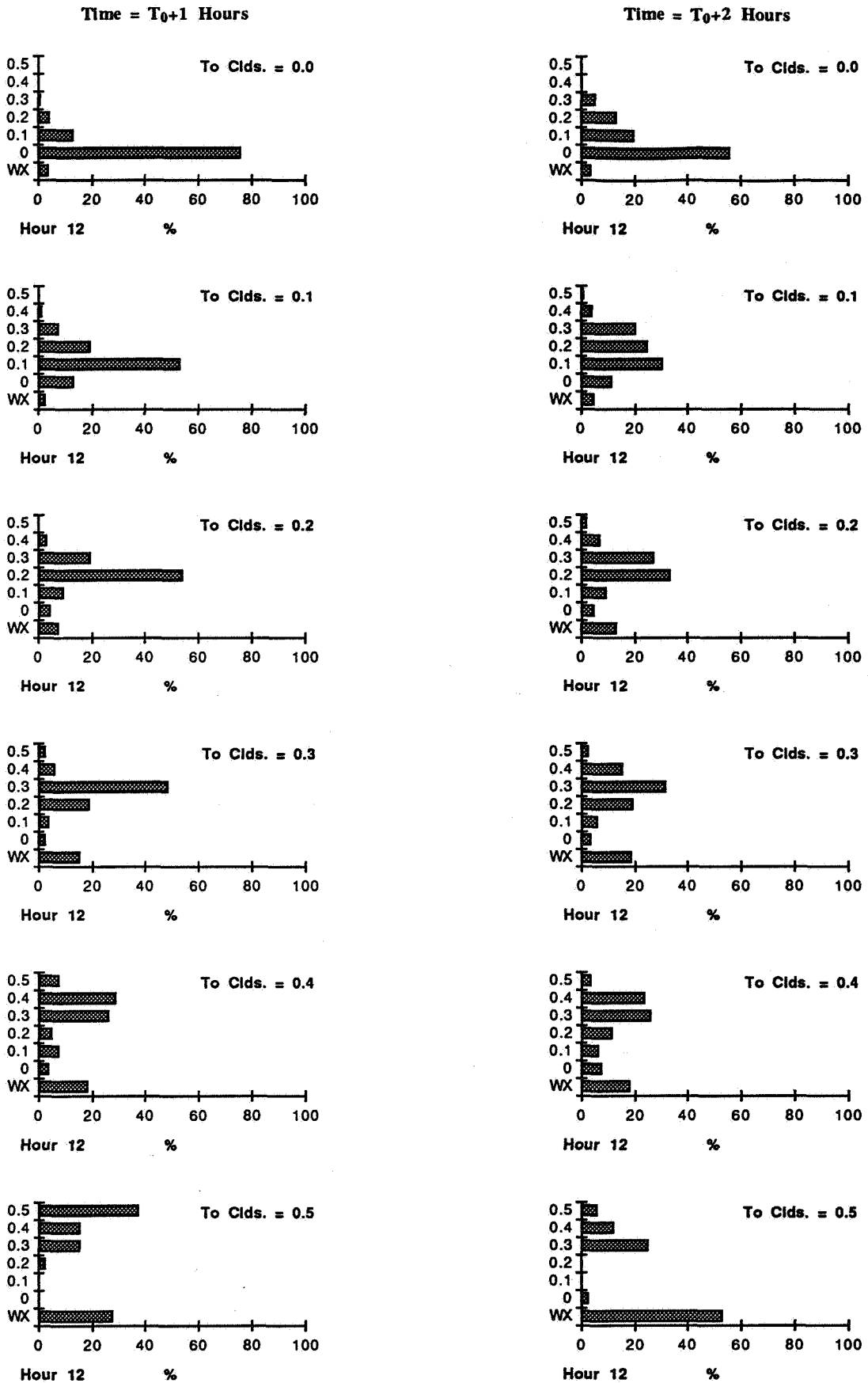
Figure E13 - Percent of Weather Violations for Hour 1200 UTC at One and Two Hours from a Given Cloud Coverage.
