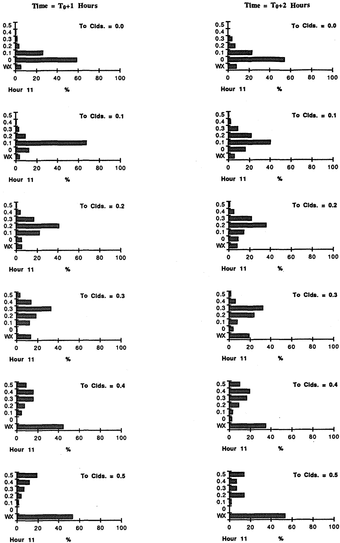
Figure E12 - Percent of Weather Condition for Hour 1100 UTC at One and Two Hours from a Given Cloud Coverage.
