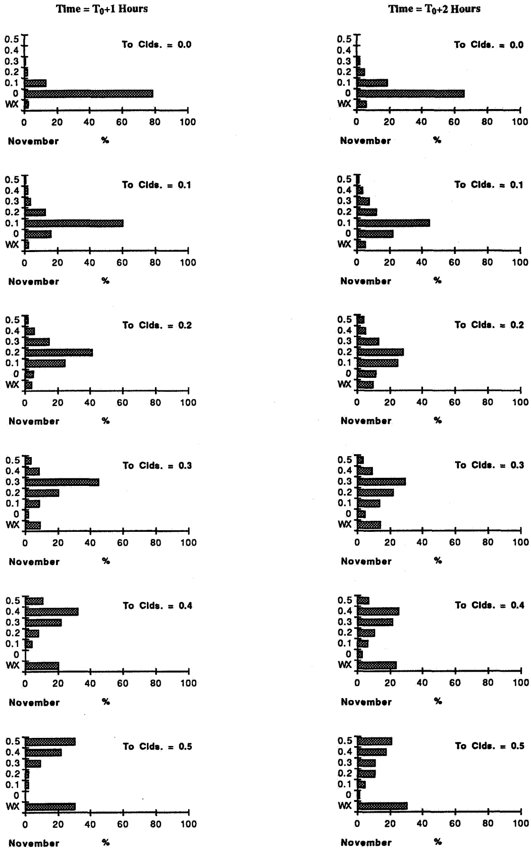
Figure D11 - Percent Occurrence of Weather Conditions for November at One and Two Hours After a Given Cloud Coverage.
