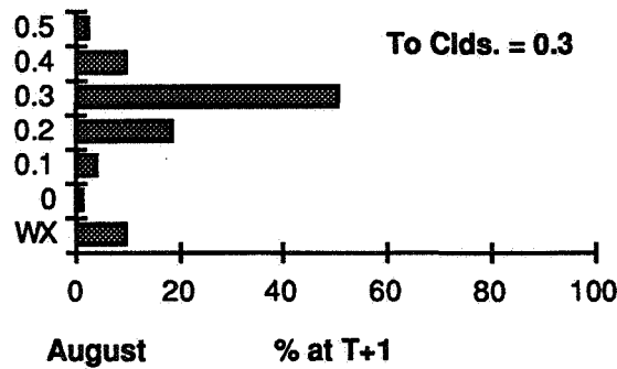
Figure 10a. Percent occurrence of cloud and weather conditions at one hour after an initial condition of 0.2 and 0.3 cloud cover.
