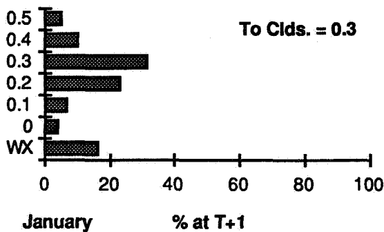
Figure 9a. Percent occurrence of cloud and weather conditions at one hour after initial condition of 0.2 and 0.3 cloud cover.
