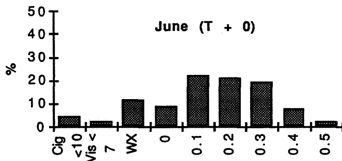
Figure 18. Climatology of weather conditions for June using daytime data.
