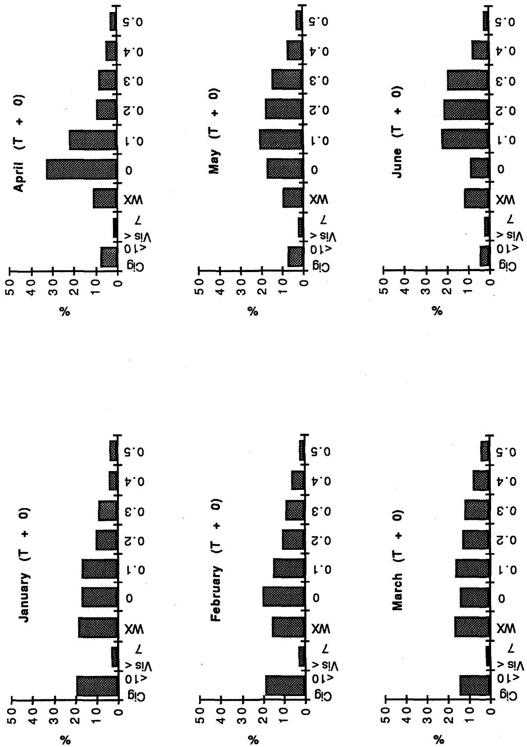
Figure A11 - Percent Occurrence of Weather Violations for initial conditions by month for Daytime data only.
