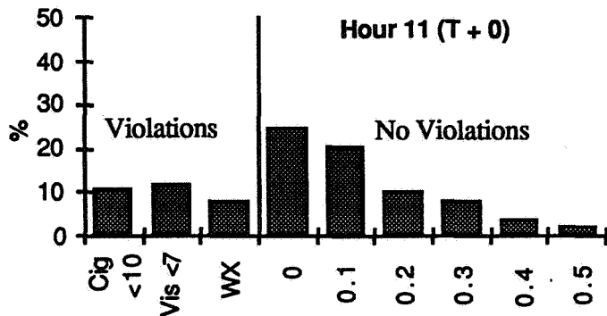
Figure 7. Percent occurrence of weather violations and cloud cover for Hour 11.
