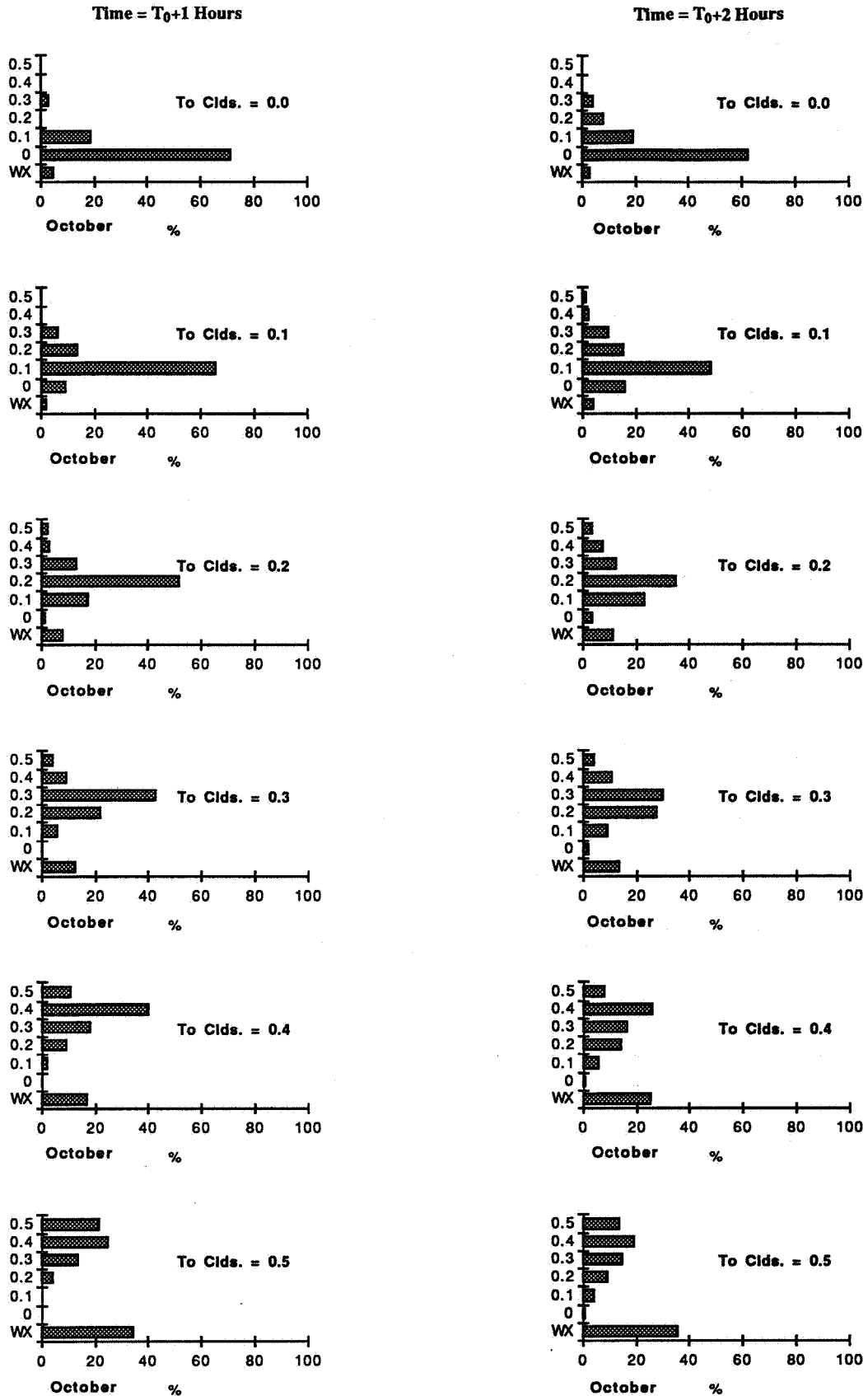
Figure G10 - Percent Occurrence of Weather Conditions for October at One and Two Hours After a Given Cloud Coverage.
