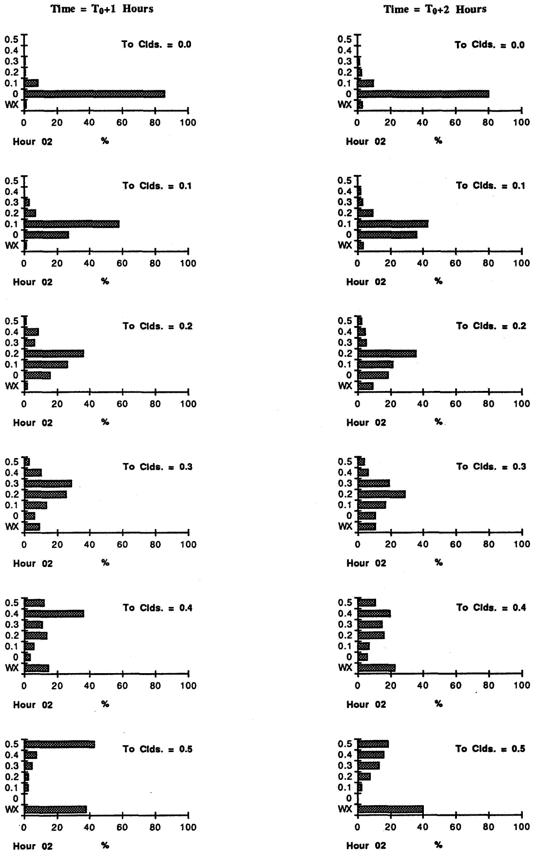
Figure E3 - Percent of Weather Violations for Hour 0200 UTC at One and Two Hours from a Given Cloud Coverage.
