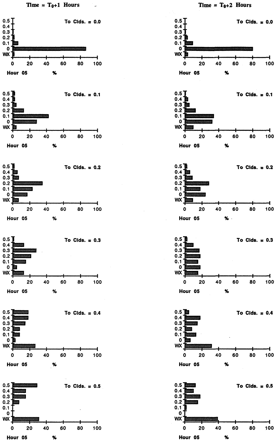
Figure E6 - Percent of Weather Conditions for Hour 0500 UTC at One and Two Hours from a Given Cloud Coverage.
