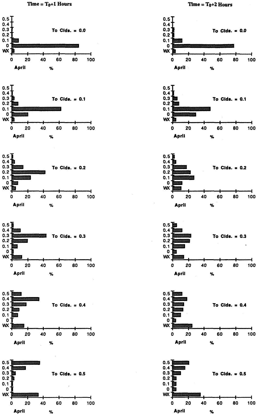
Figure G4 - Percent Occurrence of Weather Conditions for April at One and Two Hours After a Given Cloud Coverage.
