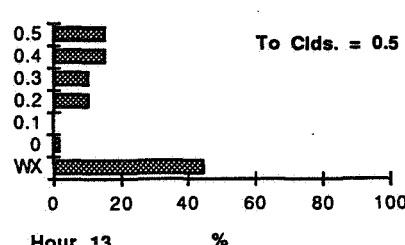
Figure E14 - Percent of Weather Conditions for Hour 1300 UTC at One and Two Hours from a Given Cloud Coverage.
