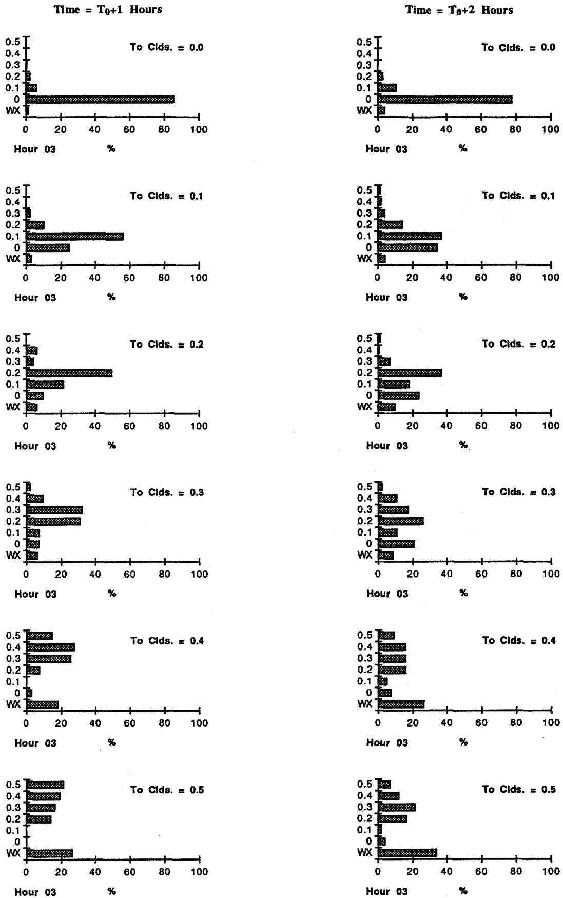
Figure E4 - Percent of Weather Violations for Hour 0300 UTC at One and Two Hours from a Given Cloud Coverage.
