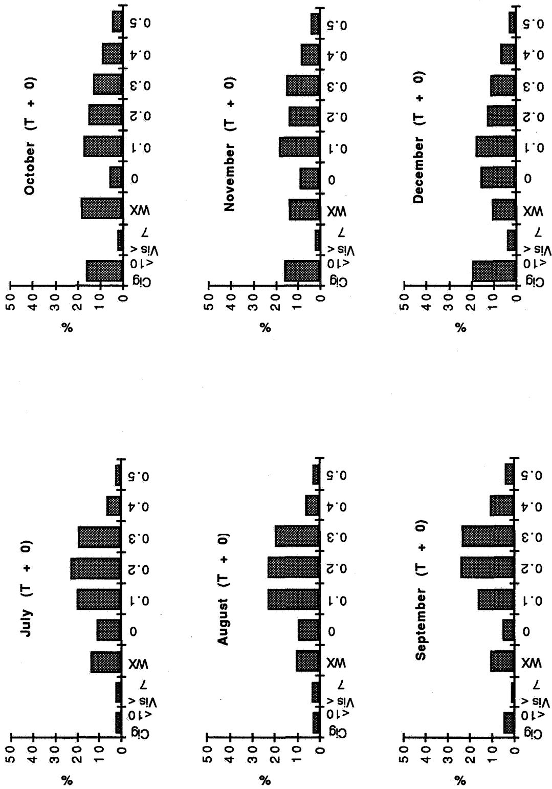
Figure A12 - Percent Occurrence of Weather Violations for initial conditions by month for Daytime data only.
