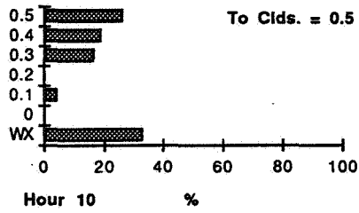
Figure E11 - Percent of Weather Conditions for Hour 1000 UTC at One and Two Hours from a Given Cloud Coverage.
