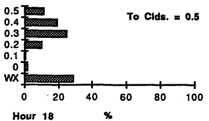
Figure E19 - Percent of Weather Conditions for Hour 1800 UTC at One and Two Hours from a Given Cloud Coverage.
