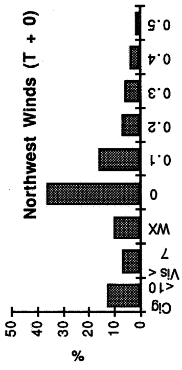
Figure A10 - Percent Occurrence of Initial Weather Conditions for All Hours Stratified by Wind Direction.
