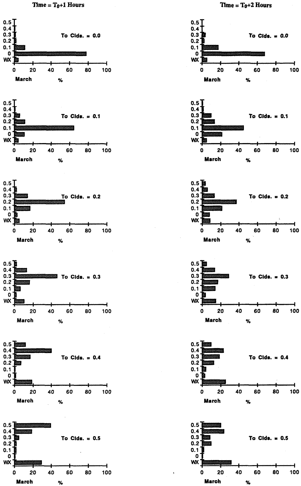
Figure G3 - Percent Occurrence of Weather Conditions for March at One and Two Hours After a Given Cloud Coverage.
