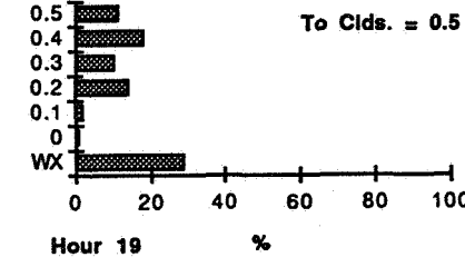
Figure E20 - Percent of Weather Conditions for Hour 1900 UTC at One and Two Hours from a Given Cloud Coverage.
