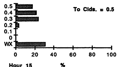
Figure E16 - Percent of Weather Conditions for Hour 1500 UTC at One and Two Hours from a Given Cloud Coverage.
