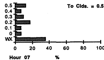
Figure E8 - Percent of Weather Conditions for Hour 0700 UTC at One and Two Hours from a Given Cloud Coverage.
