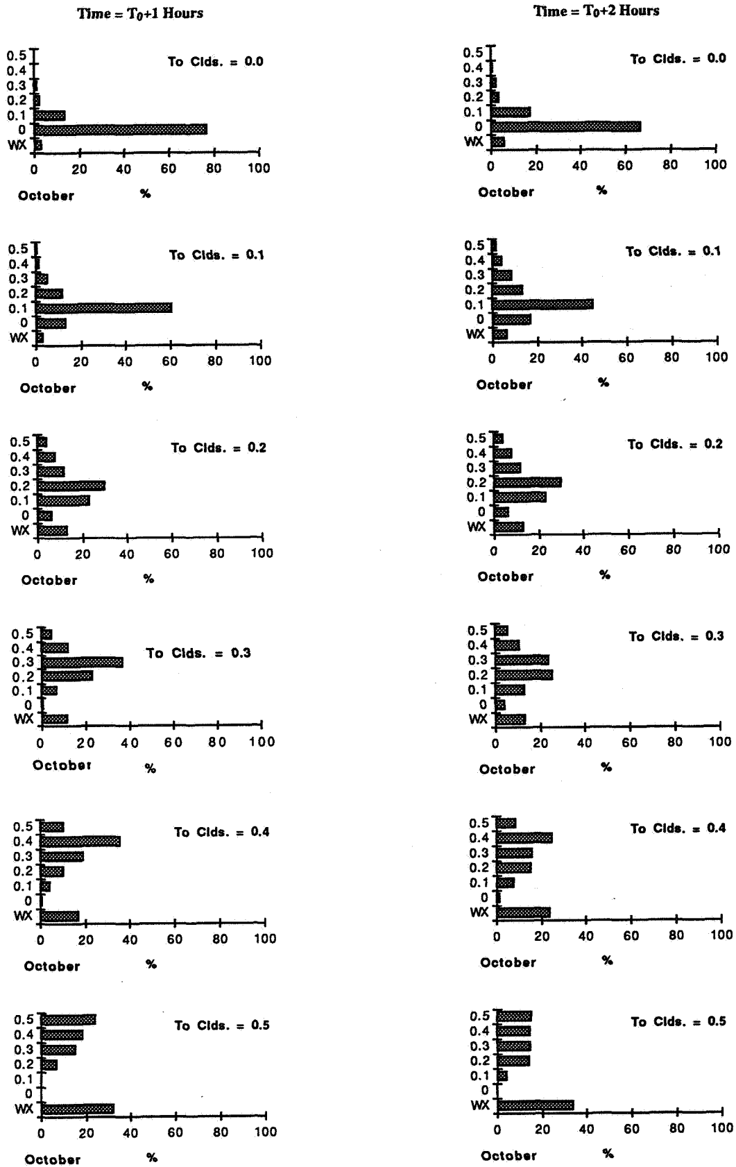
Figure D10 - Percent Occurrence of Weather Conditions for October at One and Two Hours After a Given Cloud Coverage.
