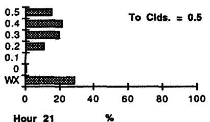
Figure E22 - Percent of Weather Conditions for Hour 2100 UTC at One and Two Hours from a Given Cloud Coverage.
