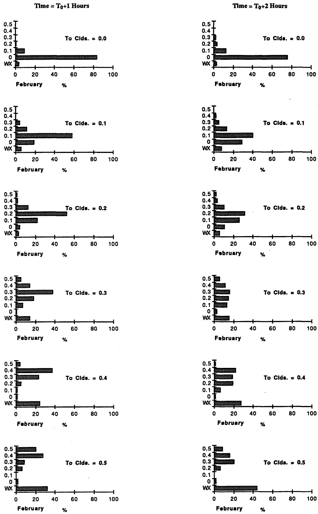
Figure G2 - Percent Occurrence of Weather Conditions for February at One and Two Hours After a Given Cloud Coverage.
