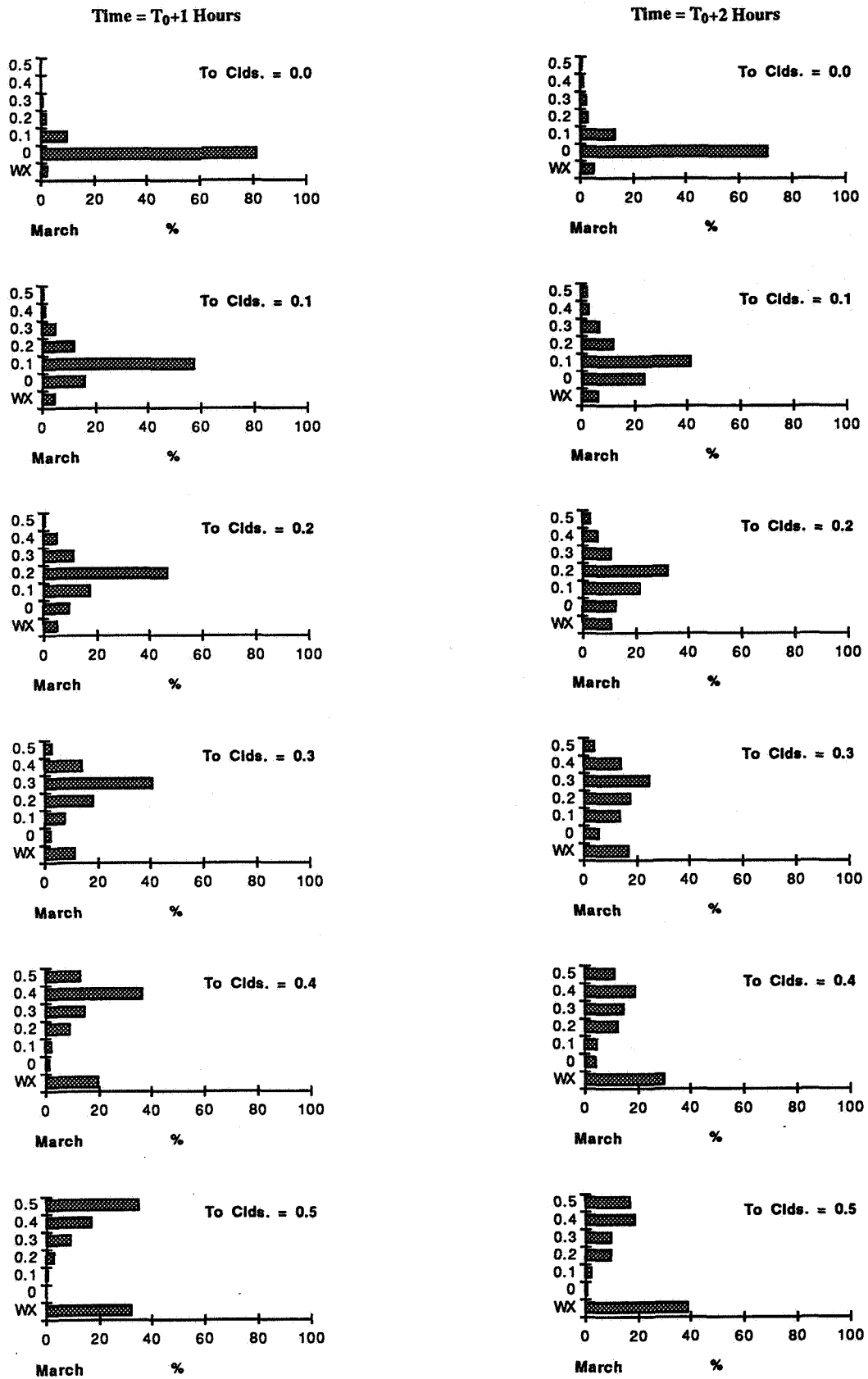
Figure D3 - Percent Occurrence of Weather Conditions for March at One and Two Hours After a Given Cloud Coverage.
