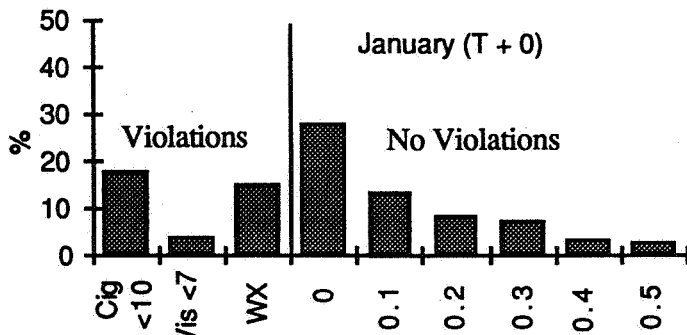
Figure 2. Percent occurrence of weather violations and cloud cover for January.
