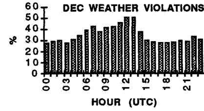
Figure J1 - Climatology of Weather Violations Categorized by Month and Hour of Day.
