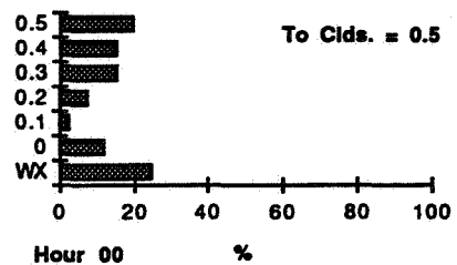
Figure E1 - Percent of Weather Conditions for Hour 0000 UTC at One and Two Hours from a Given Cloud Coverage.
