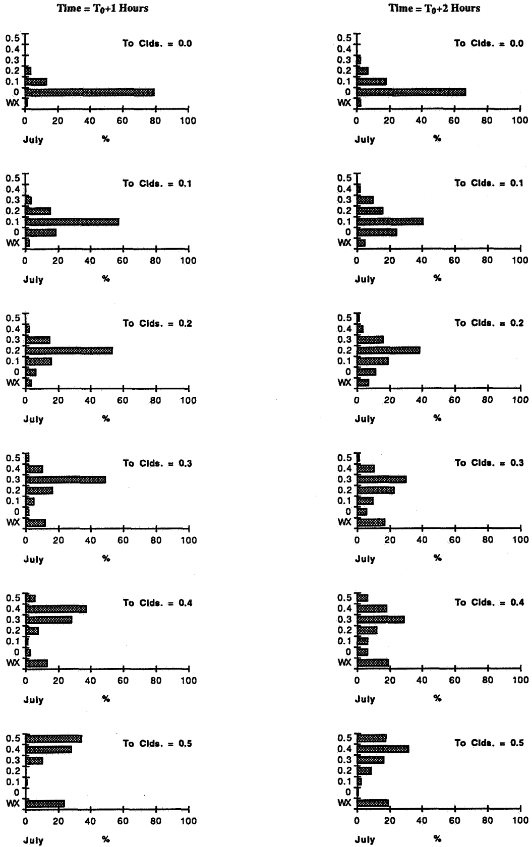
Figure D7 - Percent Occurrence of Weather Conditions for July at One and Two Hours After a Given Cloud Coverage.
