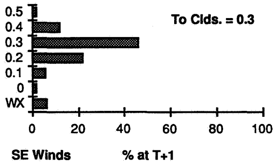
Figure 16a. Percent occurrence of cloud cover and weather conditions at one hour after an initial condition of 0.2 and 0.3 cloud cover for southeast winds.
