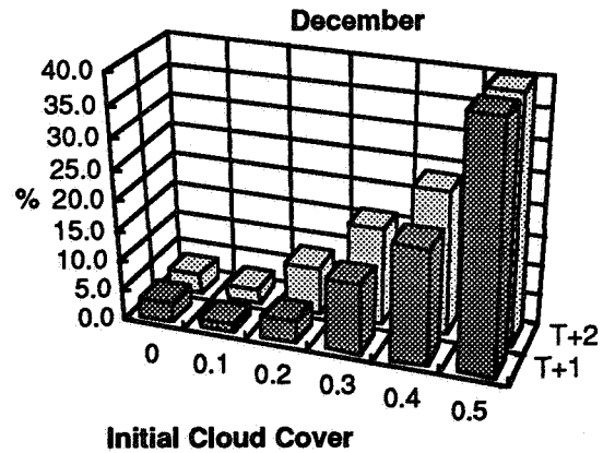
Figure H2. Percent Occurrence of Weather Violations for July to December For T+1 and T+2 Hours.
