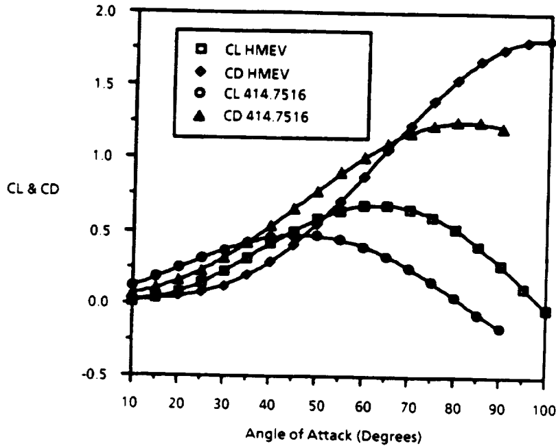
Figure 11-10. Aerodynamic Coefficients for BMEV and HMEV
