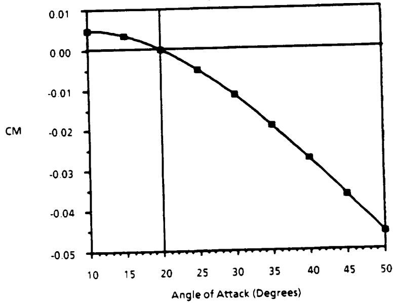
Figure 11-12. Moment Coefficient for Concept 414.7516
