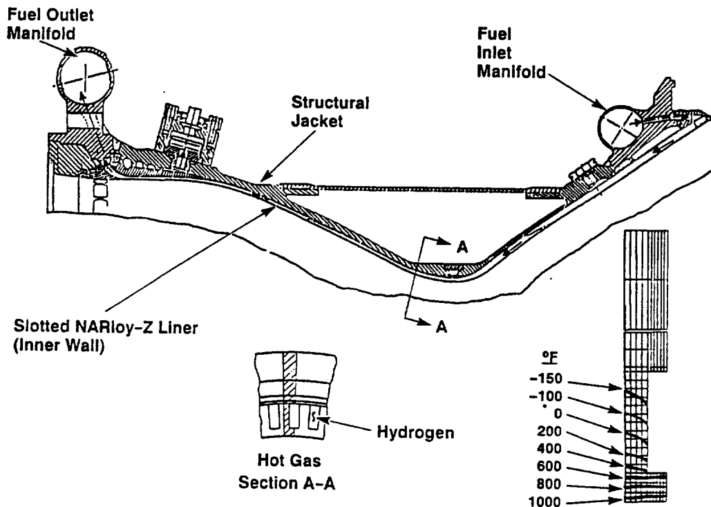
Figure 7. Typical Main Combustion Chamber Geometry.
