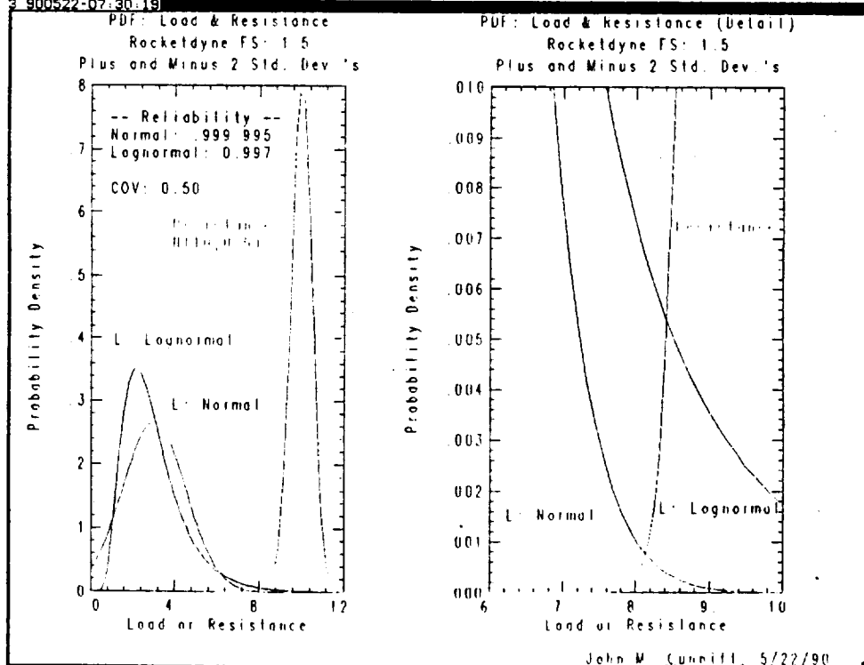
Figure 5. Reliability vs. Factor of Safety of 1.5.
