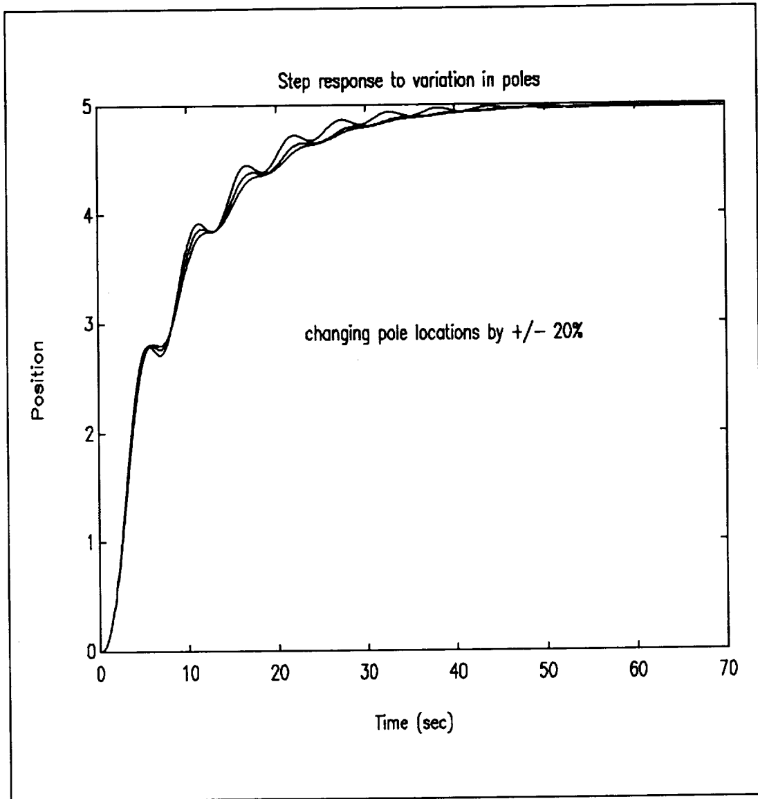
Figure 3.21. Step response to variations in pole location.
