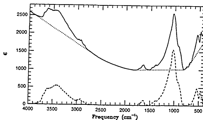
Fig. 1. Solid line is the initial calculated mass extinction coefficient ( \epsilon ) of one palagonite sample. The dotted line is the straight line continuum and the dashed line is the difference between \epsilon and the continuum.
