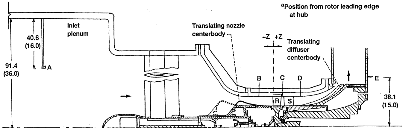
Figure 5.—Transducer positions. All dimensions in centimeters (inches).
