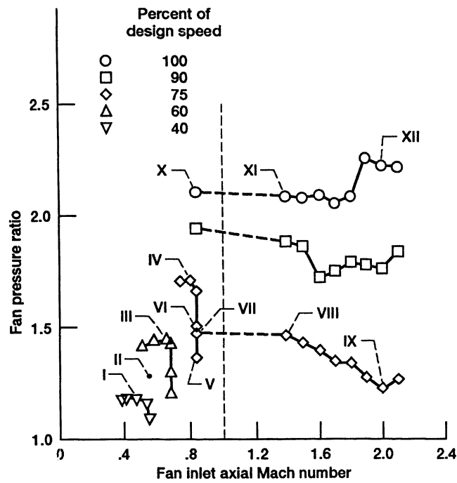
Figure 6.—Test conditions.
