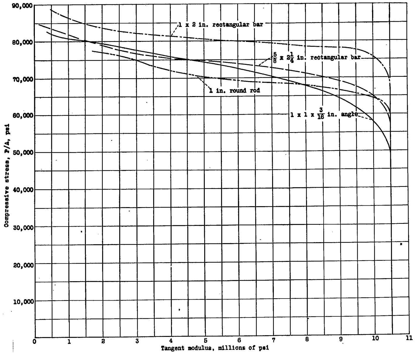
Figure 6.- Compressive stress tangent modulus curves for 758-T extruded shapes and rolled and drawn rod.
