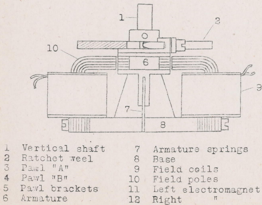
Fig.2 Diagrammatic drawing of direct current synchronous motor.
