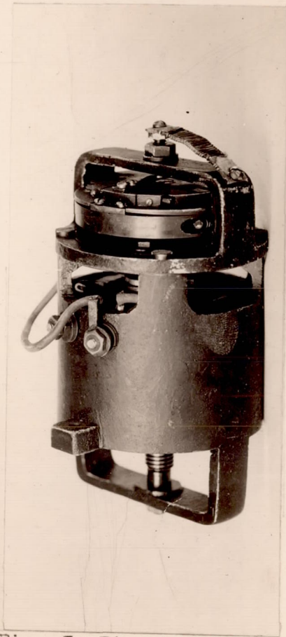
Fig. 5 Direct current governed series motor now used in instruments
