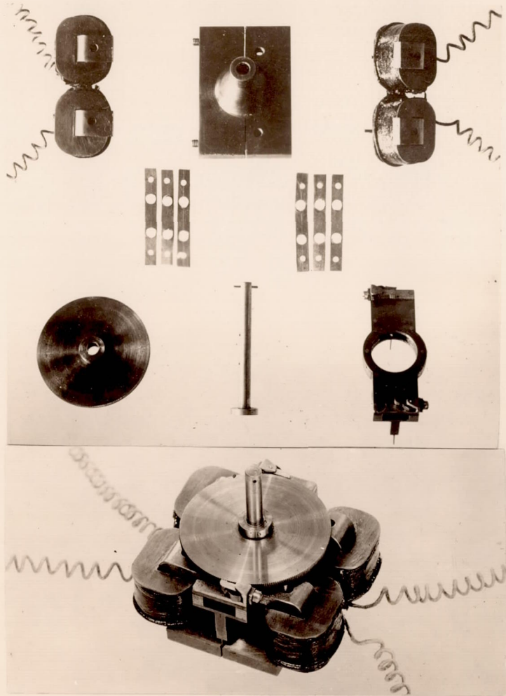
Fig. 1 Details and Assembly of direct current synchronous motor.
