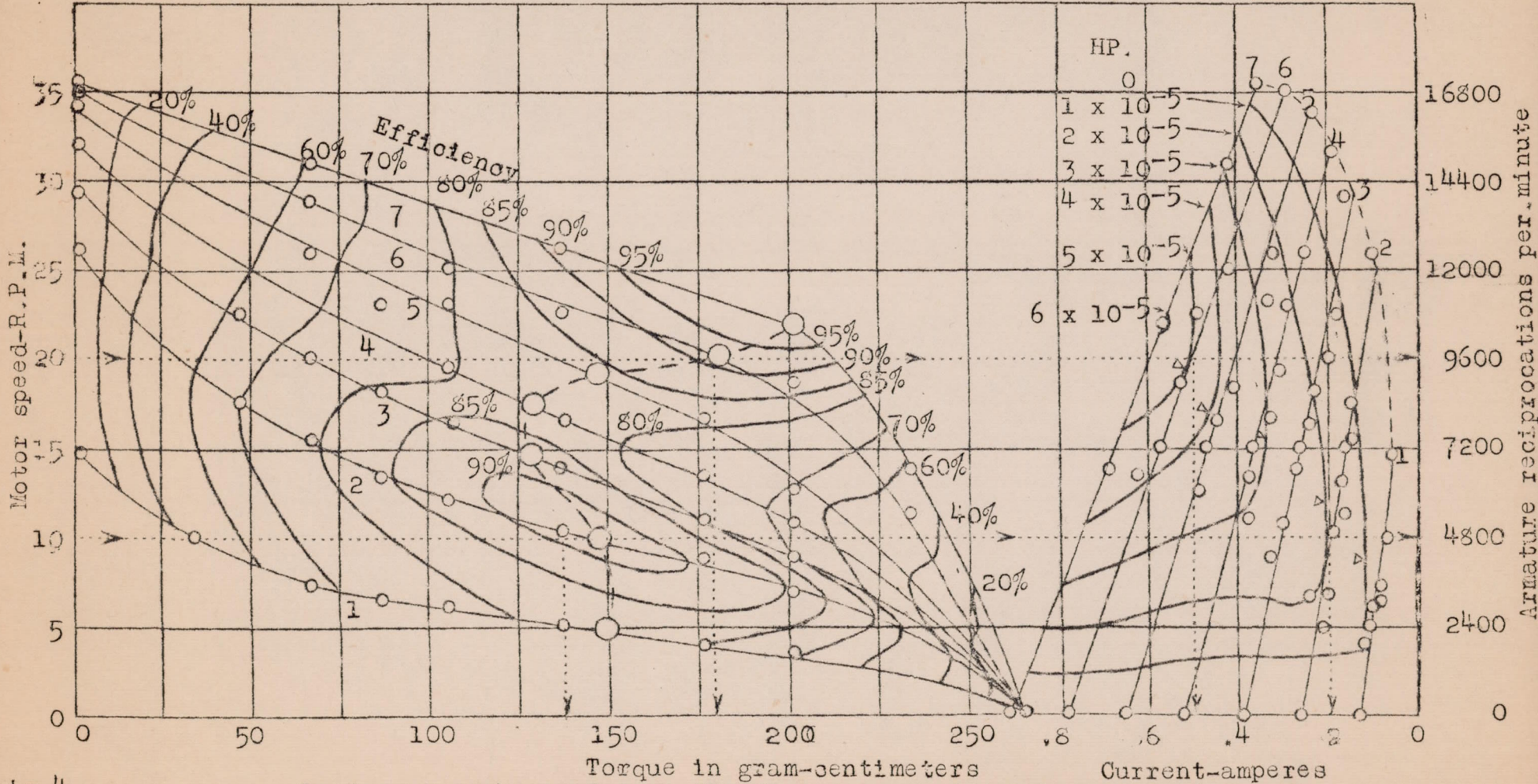
fig. 4 Performance chart of type "B" direct current synchronous motor
